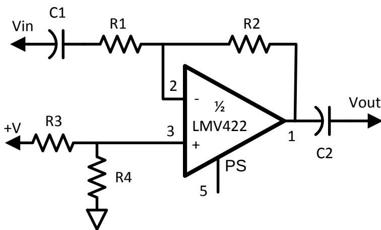
Figure 1. AC Coupled Application
