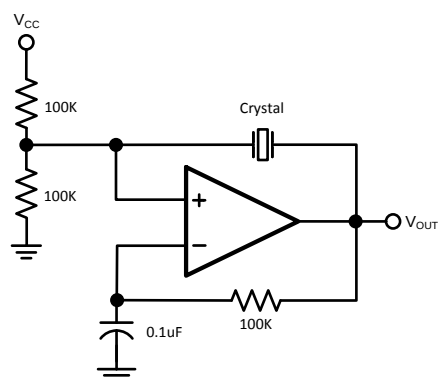
Figure 1. Crystal Oscillator
