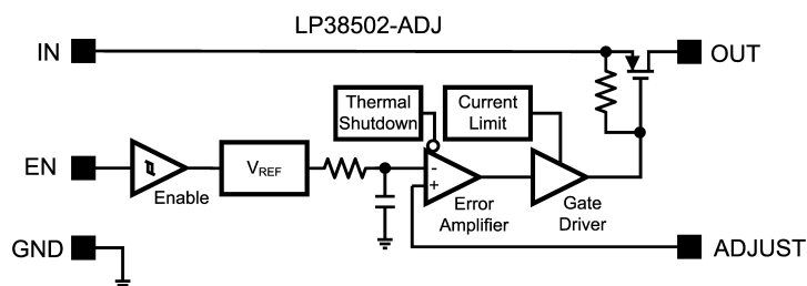
Figure 19. LP38502-ADJ DDPak/TO-263 Block Diagram
