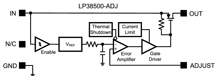
Figure 18. LP38500-ADJ DDPak/TO-263 Block Diagram
