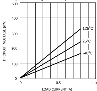
Dropout Voltage vs Output Load Current
