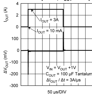
Load Transient Response, C_{OUT} = 100\text{ }\mu\text{F} Tantalum
