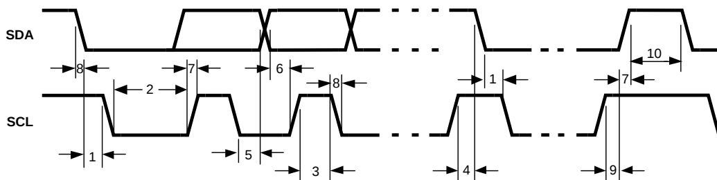
Figure 27. I²C Timing Diagram
