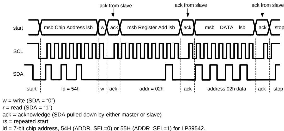
Figure 25. I²C Write Cycle
