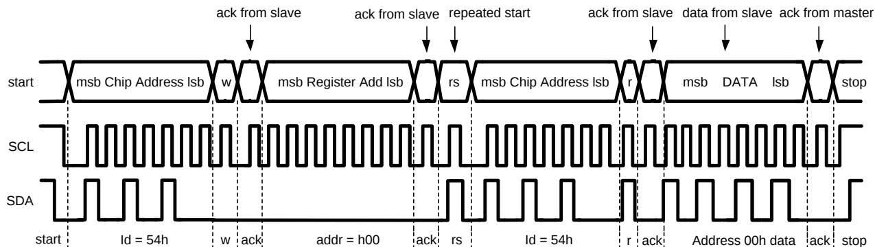
Figure 26. I²C Read Cycle
