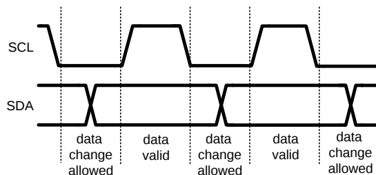
Figure 23. I²C Signals: Data Validity
