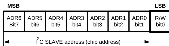
Figure 24. I²C Chip Address
