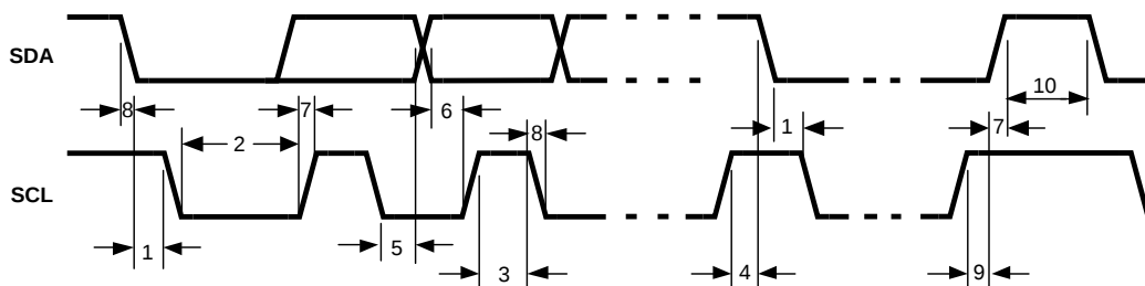
Figure 27. I²C Timing Diagram
