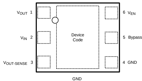
Figure 2. Top View WSOP-6 Package See Package Number NGC0006D
