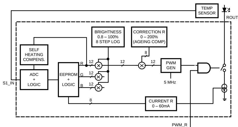
Figure 12. LED control principle
