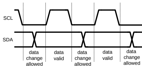
Figure 26. I²C Signals: Data Validity
