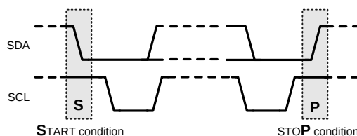
Figure 27. I²C Start and Stop Conditions
