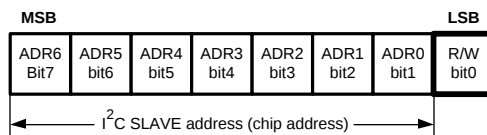
Figure 28. I²C Chip Address
