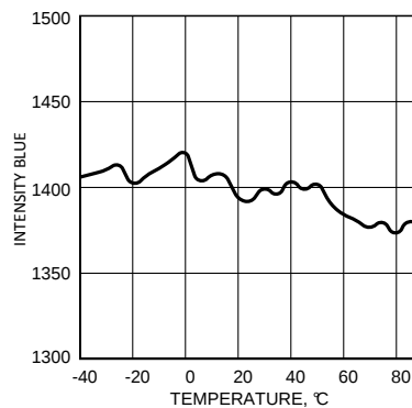
Figure 11. Compensated Blue LED Intensity vs. Temperature
