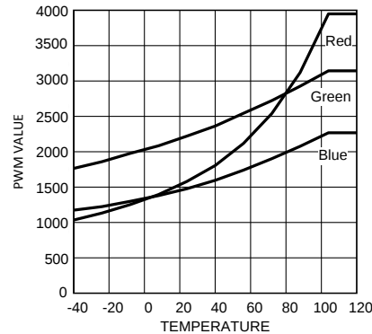
Figure 9. Compensation PWM Values
