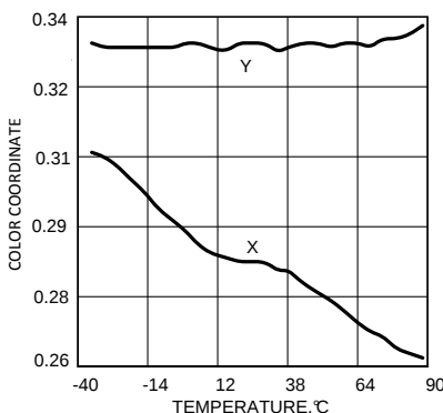
Figure 8. Typical Color Coordinates vs. Temperature for uncompensated RGB LED
