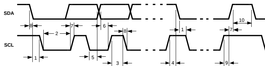
Figure 31. I²C Timing Diagram
