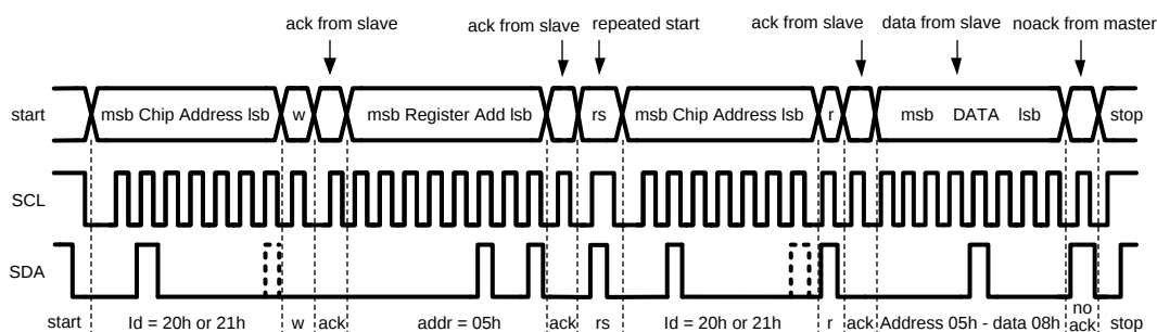
Figure 30. I²C Read Cycle
