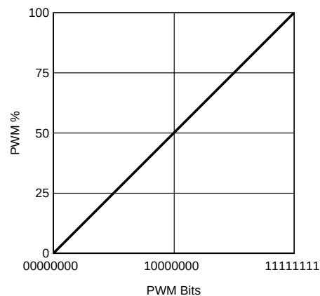
Figure 24. Direct PWM Control Bits vs. PWM Duty Cycle
