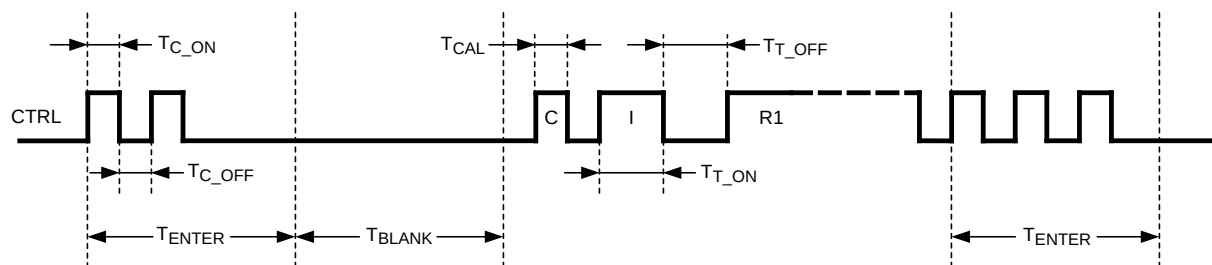
Figure 2. Interface Timing
