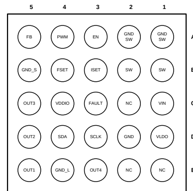
Figure 2. DSBGA-25 Package Bottom View Package Number YZR002511A
