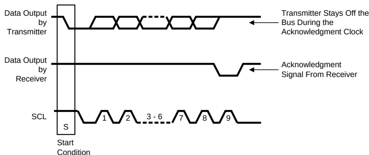
Figure 18. Start and Stop
