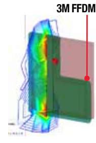
Antenna with 3M FFDM between the antenna and metal/battery parts. EM field strength increased significantly with 3M FFDM use.
