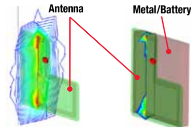
Antenna on polyimide carrier. EM field along Y-Axis in free space
