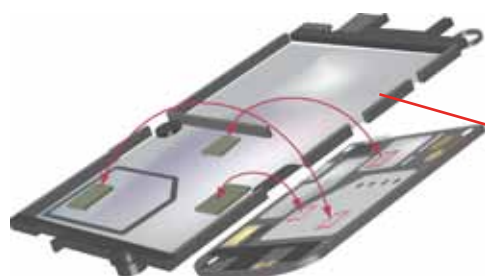
3M™ Electrically Conductive Gaskets ECG-7050/ECG-8055
