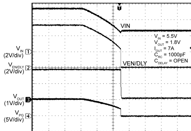
V_{IN} Turn-Off
