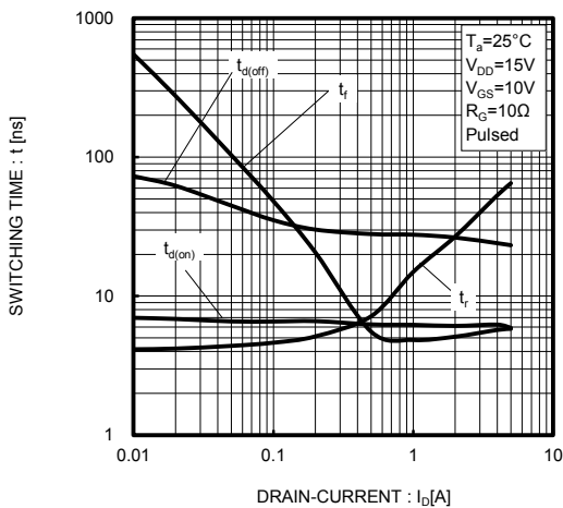
Fig.11 Switching Characteristics
