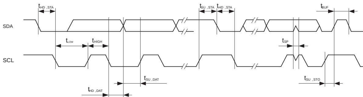
Figure 32. I2C Mode Timing
