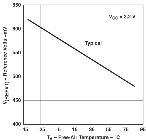
Figure 37. V_{(REFVT)} vs Temperature, V_{CC} = 2.2\text{ V}
