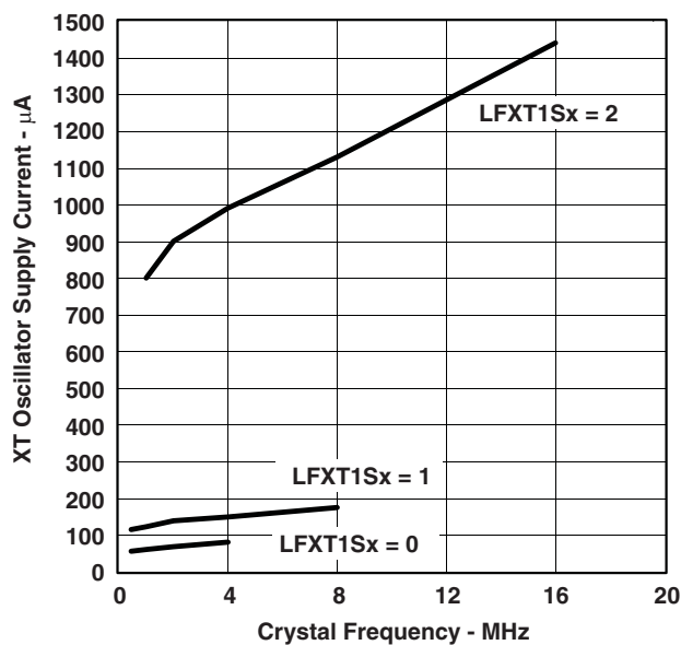
Figure 25. XT Oscillator Supply Current vs Crystal Frequency, C_{L,eff} = 15 pF, T_A = 25^\circ\text{C}
