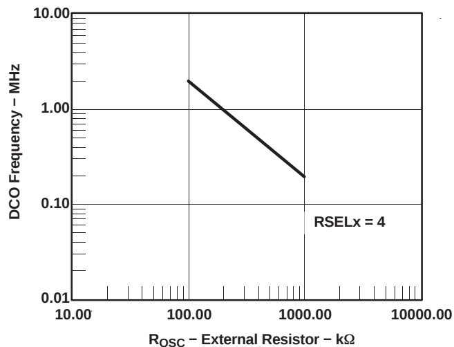
Figure 21. DCO Frequency vs R_{OSC} , V_{CC} = 3.0 V, T_A = 25^\circ\text{C}
