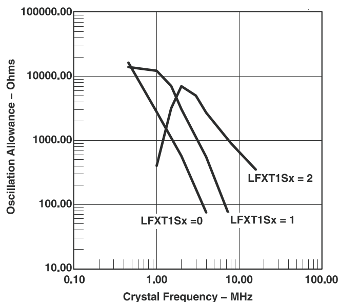
Figure 24. Oscillation Allowance vs Crystal Frequency, C_{L,eff} = 15 pF, T_A = 25^\circ\text{C}
