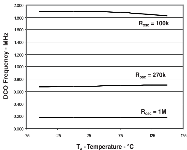
Figure 22. DCO Frequency vs Temperature, V_{CC} = 3.0 V
