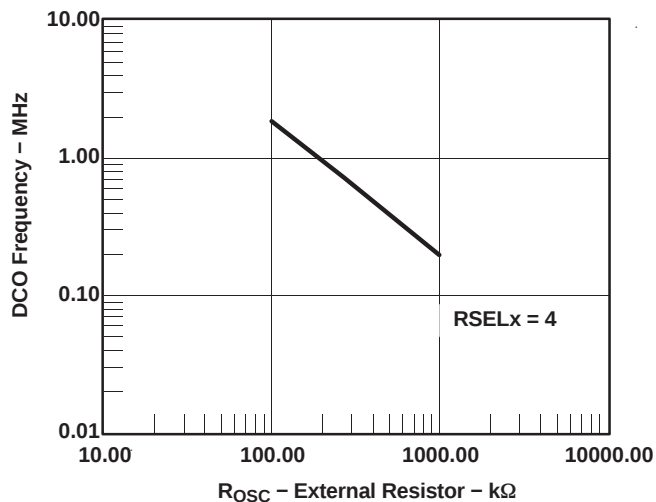
Figure 20. DCO Frequency vs R_{OSC} , V_{CC} = 2.2 V, T_A = 25^\circ\text{C}
