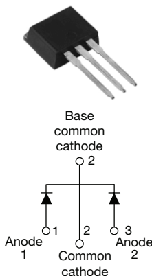
TO-262
