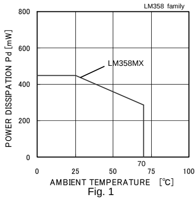
Derating Curve
