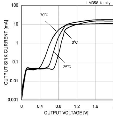
Output Sink Current – Output Voltage ( V_{CC}=5[V] )
