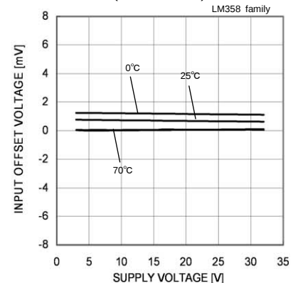
Input Offset Voltage – Supply Voltage ( V_{in}=0[V] , V_{OUT}=1.4[V] )
