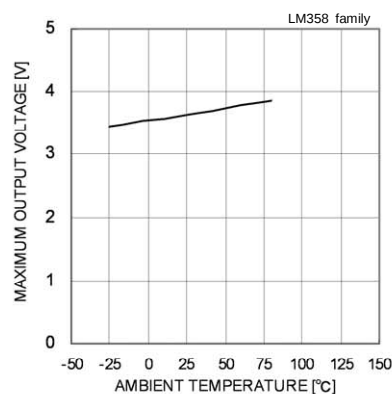
Maximum Output Voltage – Ambient Temperature ( V_{CC}=5[V] , R_L=2[k\Omega] )
