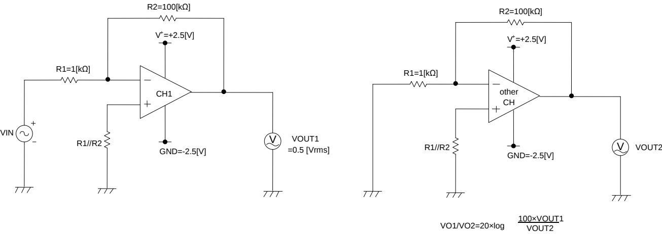
Fig.101 Measurement Circuit3
