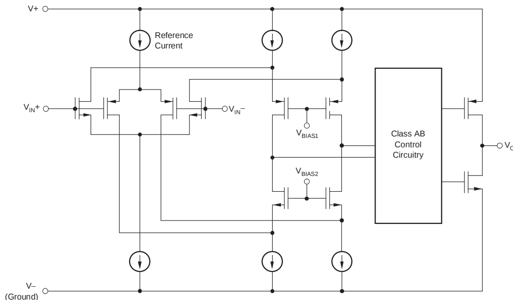
Figure 1. Simplified Schematic
