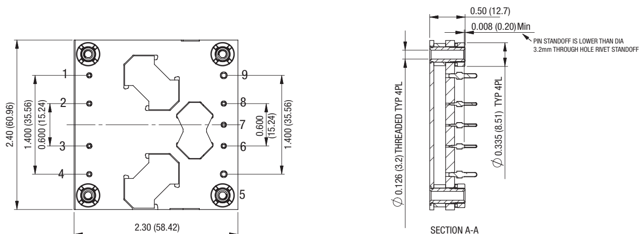
Bottom Pin Side View
