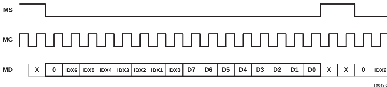
Figure 26. Write Operation Timing
