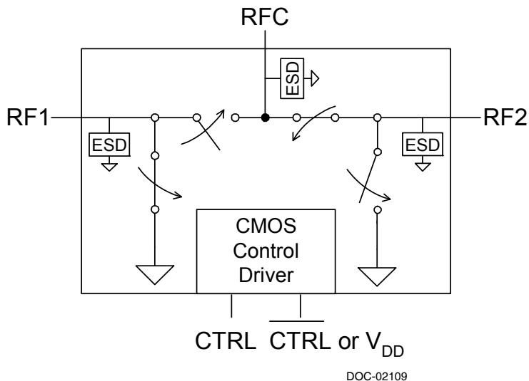
Figure 1. Functional Diagram
