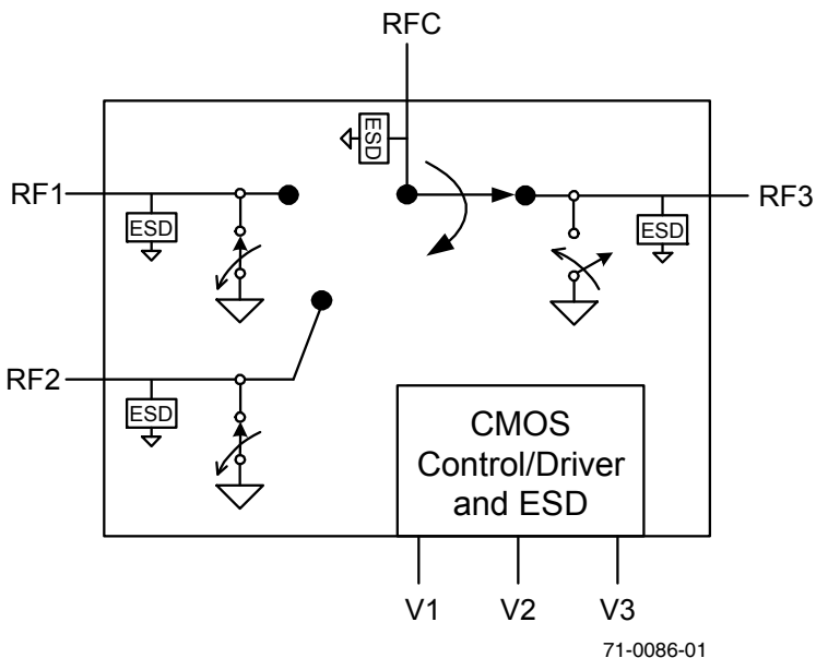
Figure 1. Functional Diagram
