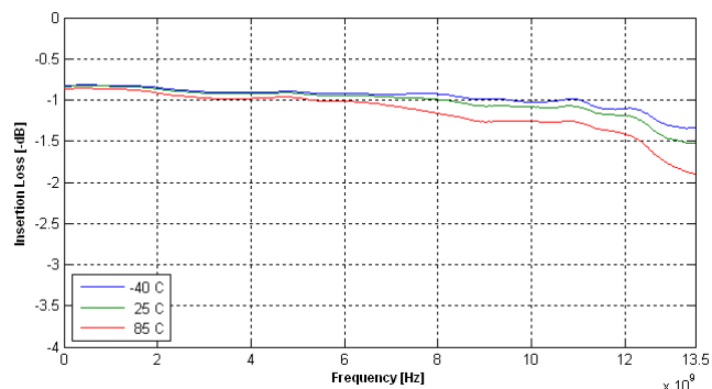
Figure 9. Insertion Loss: RFX @ 3.3V
