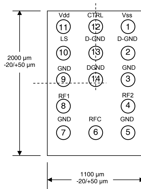
Figure 18. Pad Layout (Bumps Up)
