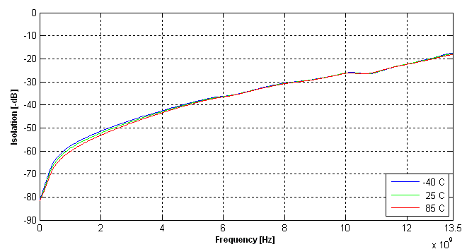
Figure 11. Isolation: Active Port to Isolated Port @ 3.3V
