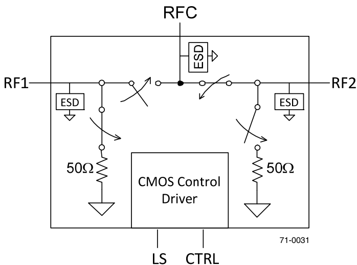
Figure 1. Functional Diagram
