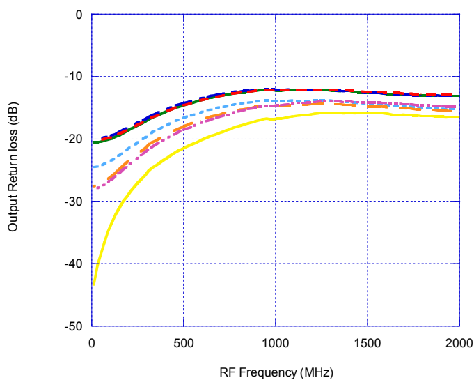
Figure 9. Output Return Loss at Major Attenuation Steps ( Z_o = 75\text{ ohms} )
