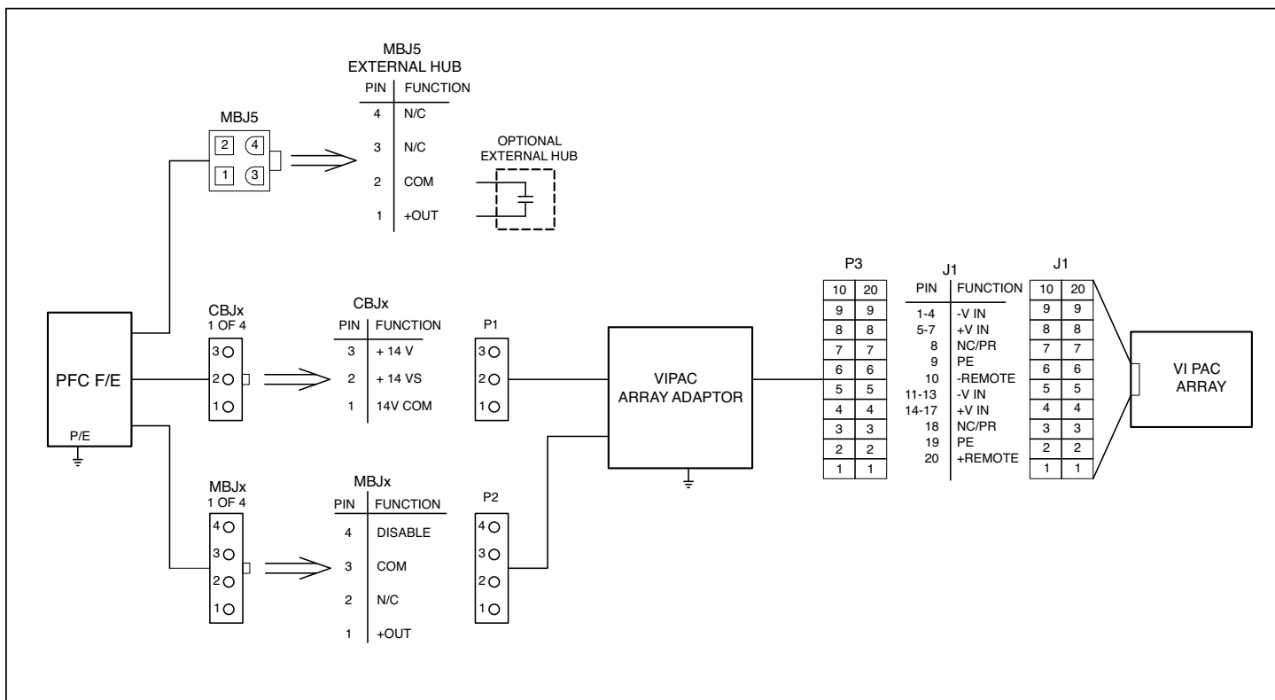
Figure 2 —Connection diagram using PFC FrontEnd with Vicor ViPAC Array.
