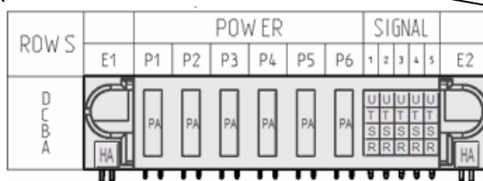
Female Connector: FCI (51732-020 LF)
