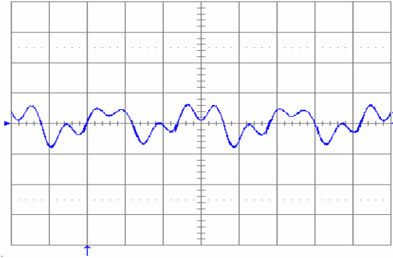
Fig. 22: Output voltage ripple (20 mV/div.) at full rated load current into a resistive load with C_o = 10 \mu\text{F} tantalum + 1\mu\text{F} ceramic and V_{in} = 24 \text{ V} . Time scale: 1 \mu\text{s}/\text{div} .
