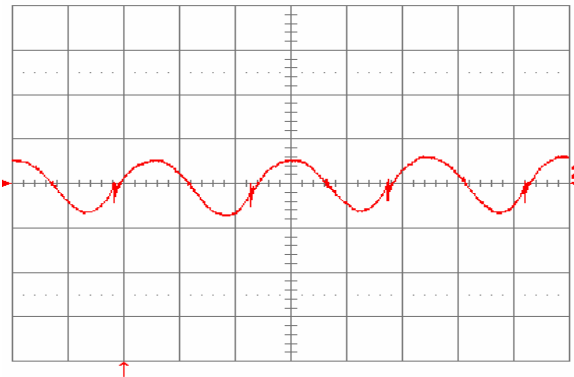
Fig. 24: Input reflected ripple current, i_c (100 mA/div), measured at input terminals at full rated load current and V_{in} = 24 \text{ V} . Refer to Fig. 23 for test setup. Time scale: 1 \mu\text{s}/\text{div} .
