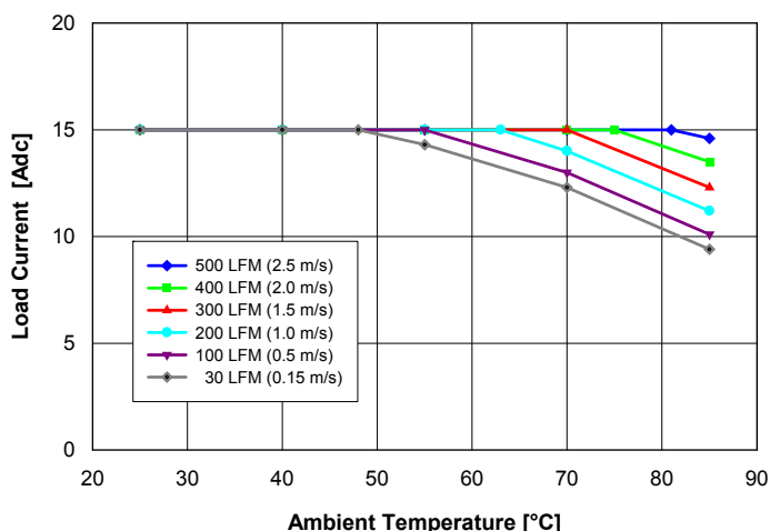
Fig. 1: Available load current vs. ambient air temperature and air-flow rates for Q24S15050 converter mounted vertically with air flowing from pin 3 to pin 1, MOSFET temperature \leq 120^{\circ}\text{C} , V_{in} = 27\text{ V} .
