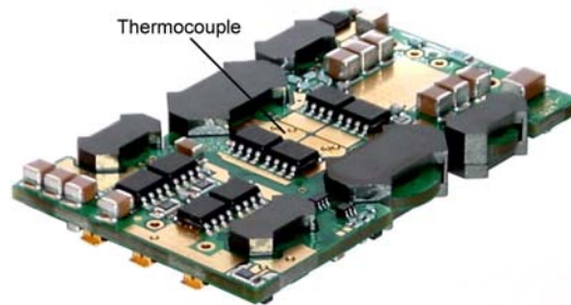
Fig. 28: Location of the thermocouple for thermal testing.
