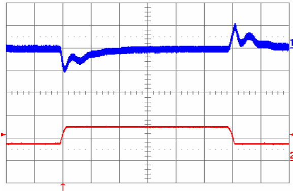
Fig. 20: Output voltage response to load current step-change (3.75 A – 7.5 A – 3.75 A) at V_{in} = 24\text{ V} . Top trace: output voltage (100 mV/div.). Bottom trace: load current (5 A/div.). Current slew rate: 0.1 A/ \mu\text{s} . C_o = 1\text{ }\mu\text{F} ceramic. Time scale: 0.2 ms/div.
