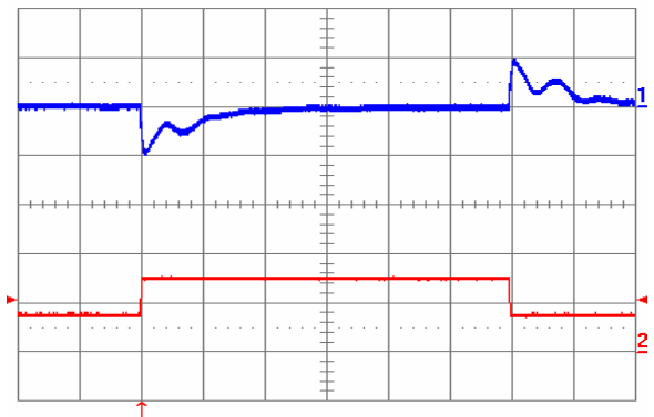
Fig. 21: Output voltage response to load current step-change (3.75 A – 7.5 A – 3.75 A) at V_{in} = 24\text{ V} . Top trace: output voltage (100 mV/div.). Bottom trace: load current (5 A/div.). Current slew rate: 5 A/ \mu\text{s} . C_o = 450\text{ }\mu\text{F} tantalum + 1 \mu\text{F} ceramic. Time scale: 0.2 ms/div.
