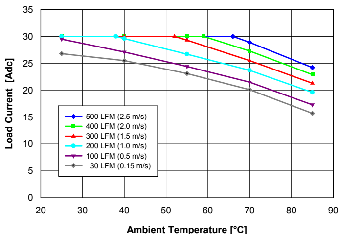
Fig. 1: Available load current vs. ambient air temperature and air-flow rates for Q24S30033 converter mounted vertically with air flowing from pin 3 to pin 1, MOSFET temperature \leq 120^{\circ}\text{C} , V_{in} = 27\text{ V} .
