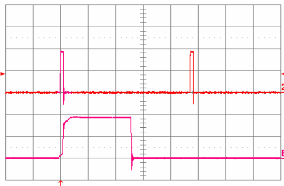
Fig. 27: Load current (top trace, 20 A/div, 20 ms/div) into a 10 mΩ short circuit during restart, at Vin = 24 V. Bottom trace (20 A/div, 1 ms/div) is an expansion of the on-time portion of the top trace.
