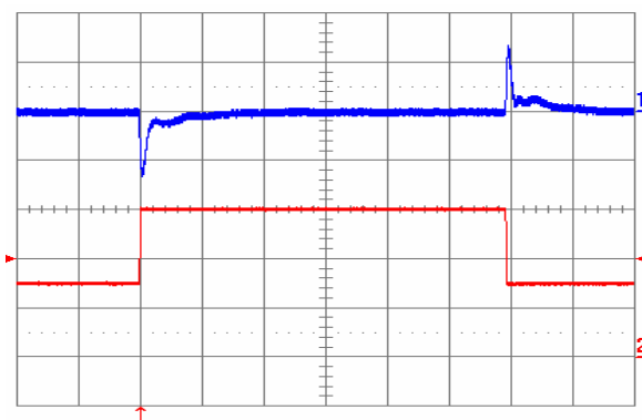
Fig. 21: Output voltage response to load current step-change (7.5 A – 15 A – 7.5 A) at V_{in} = 24\text{ V} . Top trace: output voltage (100 mV/div). Bottom trace: load current (5 A/div.). Current slew rate: 5 A/ \mu\text{s} . C_o = 450\text{ }\mu\text{F} tantalum + 1 \mu\text{F} ceramic. Time scale: 0.2 ms/div.
