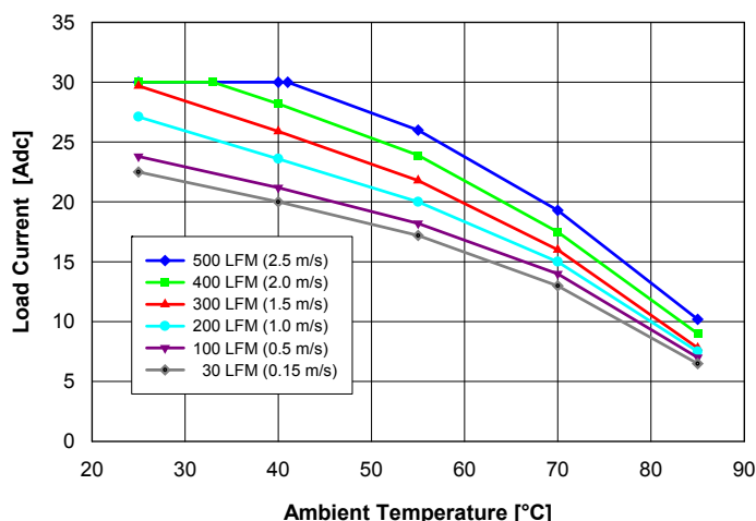
Fig. 13: Available load current vs. ambient temperature and airflow rates for converter mounted horizontally with V_{in} = 27 V, air flowing from pin 3 to pin 4 and maximum FET temperature \leq 105^{\circ}\text{C} .
