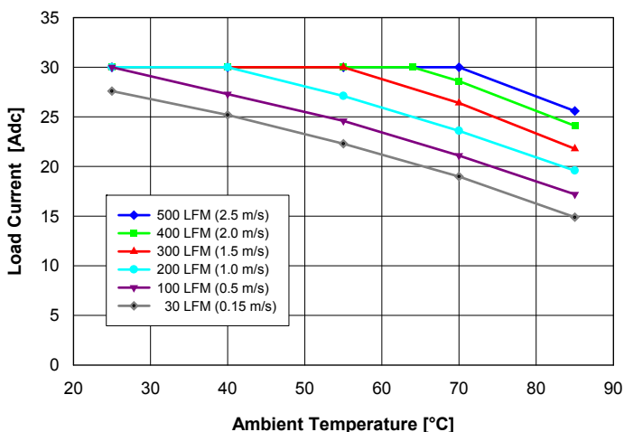
Fig. 1: Available load current vs. ambient air temperature and air-flow rates for Q24T30033 converter mounted vertically with air flowing from pin 3 to pin 1, MOSFET temperature \leq 120^{\circ}\text{C} , V_{in} = 27\text{ V} .
