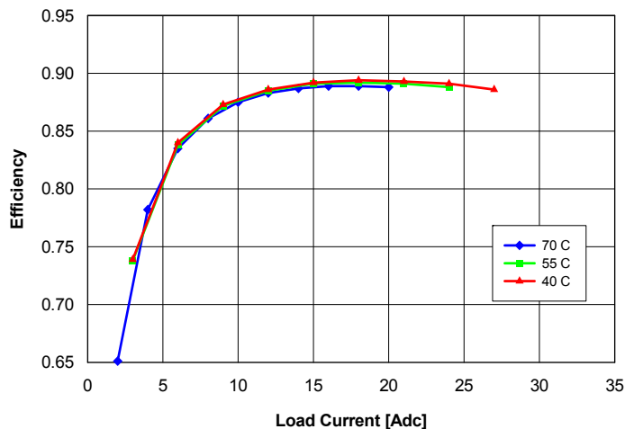
Fig. 17: Efficiency vs. load current and ambient temperature for converter mounted horizontally with V_{in} = 27\text{ V} and air flowing from pin 3 to pin 4 at a rate of 200 LFM (1.0 m/s).
