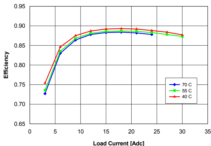
Fig. 15: Efficiency vs. load current and ambient temperature for converter mounted vertically with V_{in} = 27\text{ V} and air flowing from pin 3 to pin 1 at a rate of 200 LFM (1.0 m/s).
