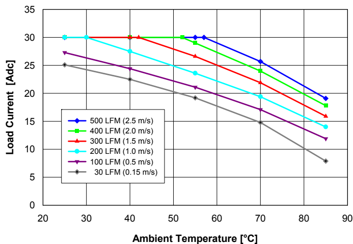
Fig. 11: Available load current vs. ambient air temperature and airflow rates for converter mounted vertically with V_{in} = 27 V, air flowing from pin 3 to pin 1 and maximum FET temperature \leq 105^{\circ}\text{C} .
