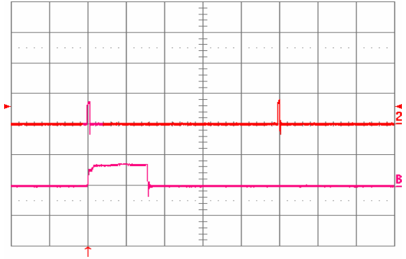
Fig. 29: Load current Iout2 into a 10 mΩ short circuit on Vout2 during restart, with Vout1 open (no load), at Vin = 48 V. Ch2 = Iout2 (20 A/div, 20 ms/div). ChB = Iout2 (20 A/div, 1 ms/div) is an expansion of the on-time portion of Iout2.
