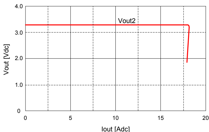
Fig. 27: Output voltage Vout2 vs. load current Iout2 showing current limit point and converter shutdown point. When Vout2 is in current limit, Vout1 is not affected until Vout2 reaches the shut-down threshold equal to Vout1 - 0.6 V. Input voltage has almost no effect on Vout2 current limit characteristic.
