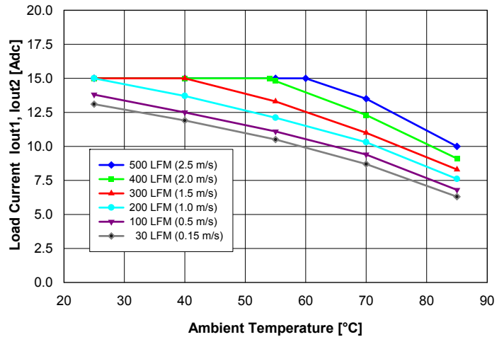
Fig. 11: Available balanced load current (Iout1 = Iout2) vs. ambient air temperature and airflow rates for converter mounted horizontally with Vin = 48 V, air flowing from pin 3 to pin 4 and maximum FET temperature ≤ 120°C.
