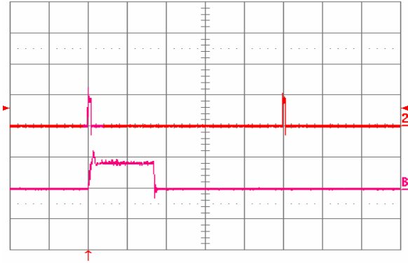
Fig. 28: Load current Iout1 into a 10 mΩ short circuit on Vout1 during restart, with Vout2 open (no load), at Vin = 48 V. Ch2 = Iout1 (20 A/div, 20 ms/div). ChB = Iout1 (20 A/div, 1 ms/div) is an expansion of the on-time portion of Iout1.
