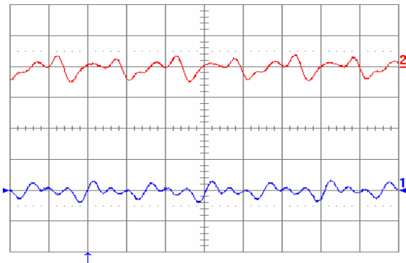
Fig. 30: Output voltage ripple at full rated load current into a resistive load on both outputs with Co = 1uF (ceramic) and Vin = 48 V. Ch2 = Vout2, Ch1 = Vout1 (both 20 mV/div). Time scale: 1 μs/div.
