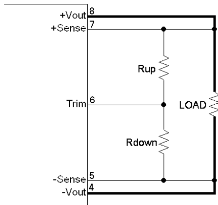
Figure 4. QLS08ZH Positive Trim Schematic
