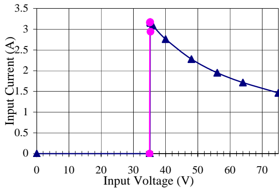
Figure 2. QLS08ZH Input Characteristics
