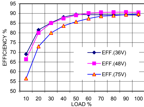
Figure 1. QLS08ZH Efficiency vs. Output Load
