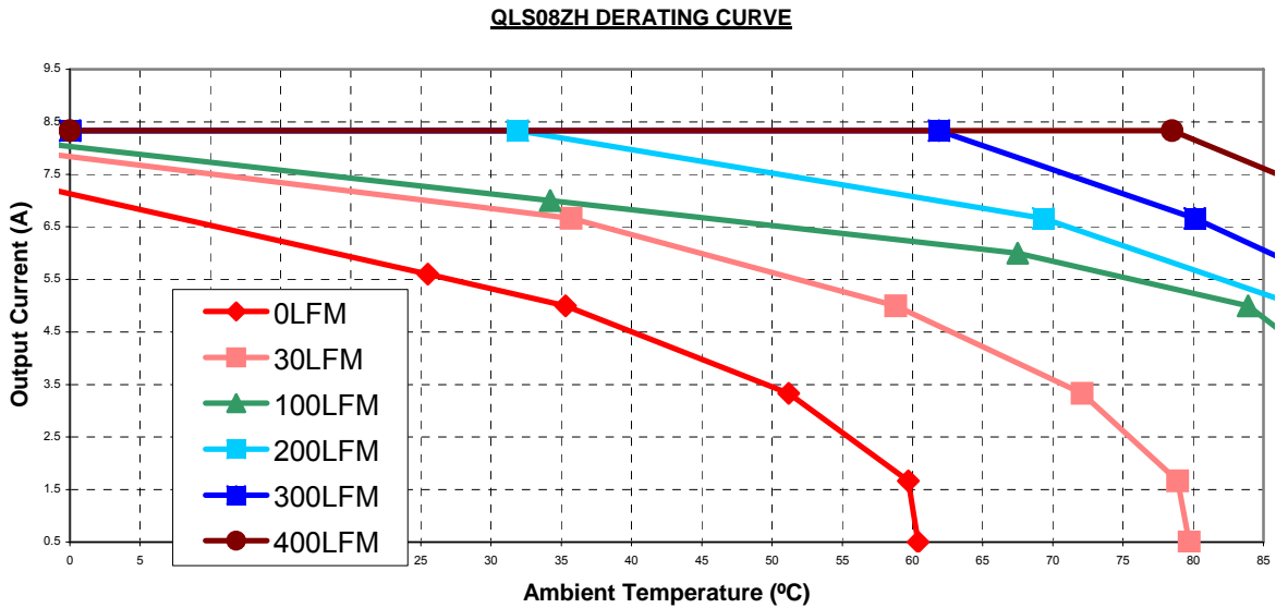
Figure 5. Derating Curves
