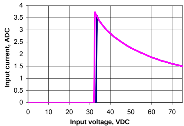
Figure 4. QLS20ZG Input Characteristic
