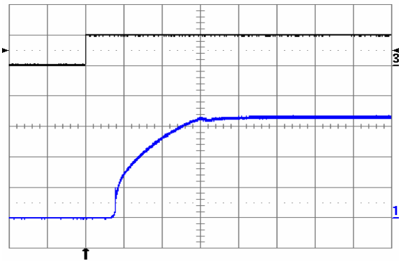
Fig. 8: Turn-on transient at full rated load current (resistive) plus 40,000\text{ }\mu\text{F} at V_{in} = 48\text{ V} , triggered via ON/OFF pin. Top trace: ON/OFF signal (5 V/div.). Bottom trace: output voltage (1 V/div.). Time scale: 2 ms/div.
