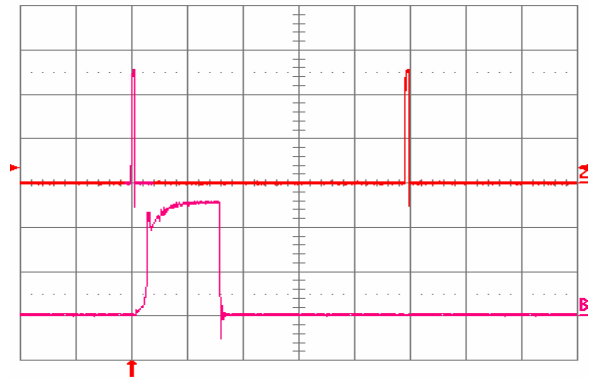
Fig. 15: Load current (top trace, 20 A/div, 20 ms/div) into a 10 m\Omega short circuit during restart, at V_{in} = 48 V. Bottom trace (20 A/div, 1 ms/div) is an expansion of the on-time portion of the top trace.
