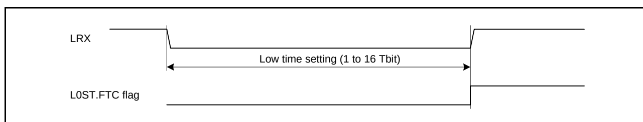
Figure 27.11 Wake-up Transmission Timing
