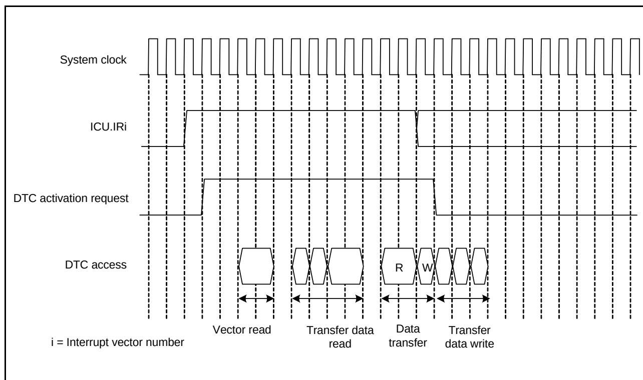
Figure 14.9 Example of DTC Operation Timing 1 (Short-Address Mode, Normal Transfer Mode, Repeat Transfer Mode)
