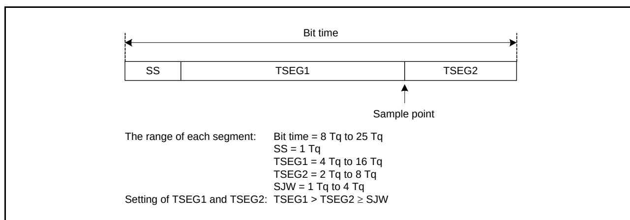
Figure 25.12 Bit Timing
