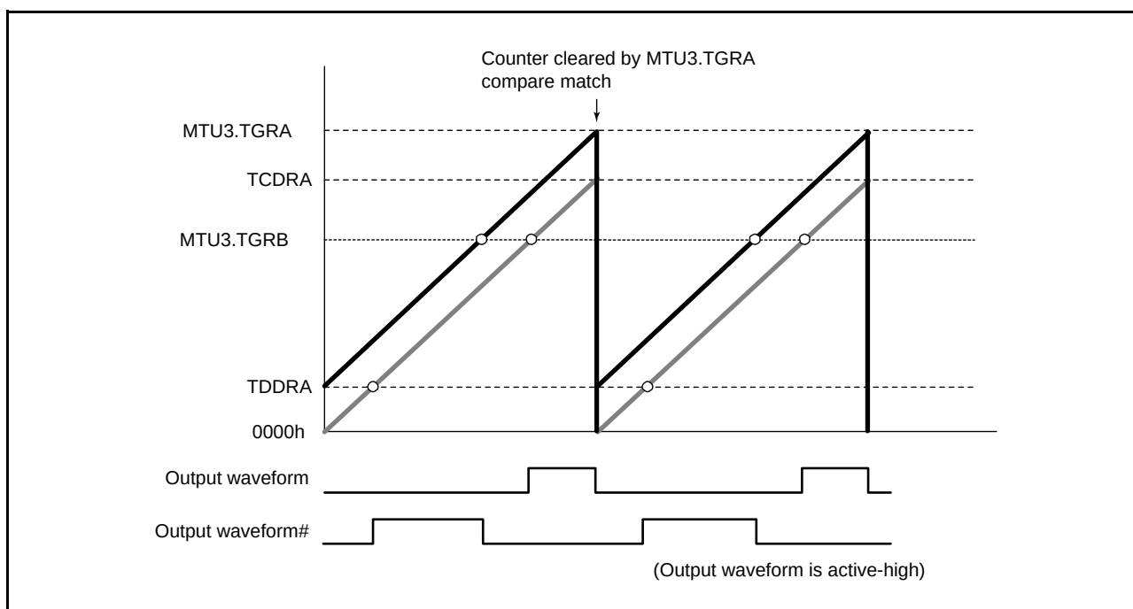
Figure 16.69 Example of Counter Clearing Operation by MTU3.TGRA Compare Match
