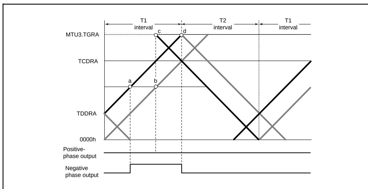
Figure 16.52 Example of 0% and 100% Waveform Output in Complementary PWM Mode (MTU3 and MTU4) (3)
