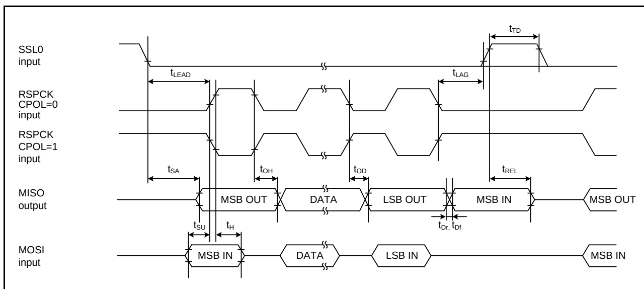
Figure 33.14 RSPI Timing (Slave, CPHA = 0)
