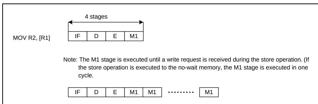
Figure 2.13 Store Operation
