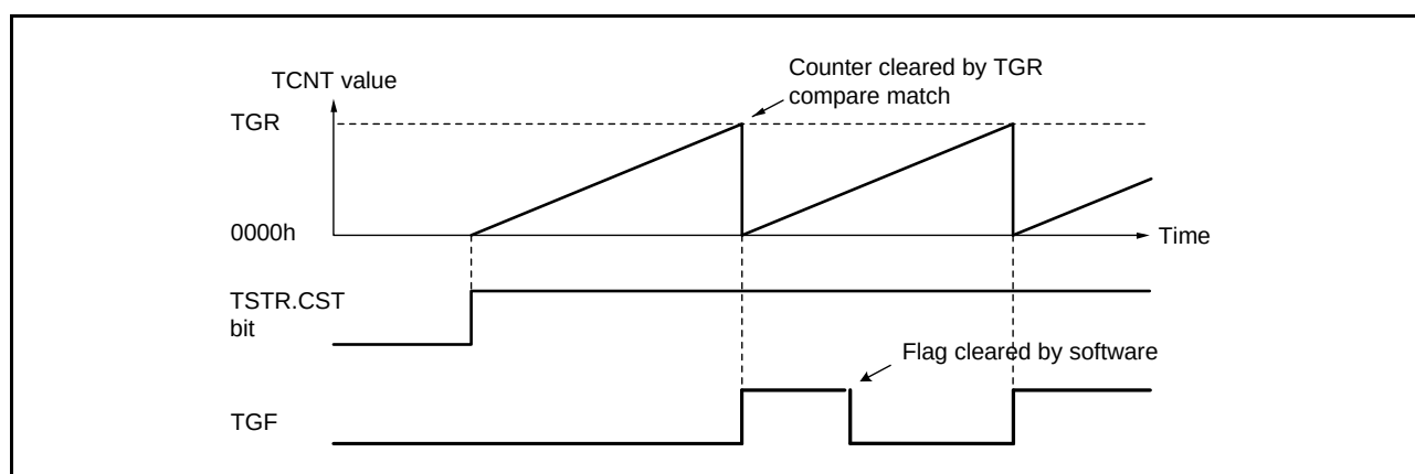
Figure 16.7 Periodic Counter Operation
