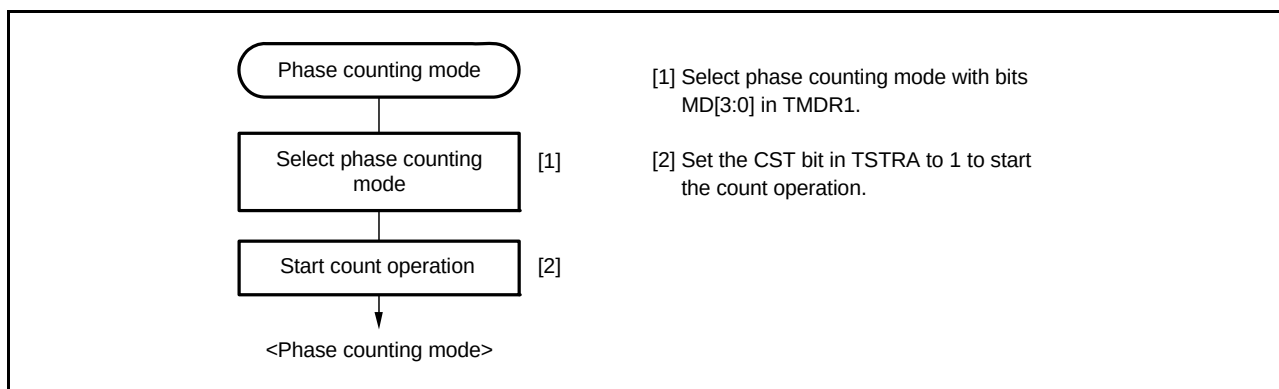
Figure 16.30 Example of Phase Counting Mode Setting Procedure
