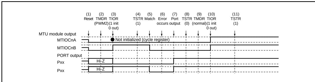
Figure 16.153 Error Occurrence in PWM Mode 2, Recovery in Normal Mode
