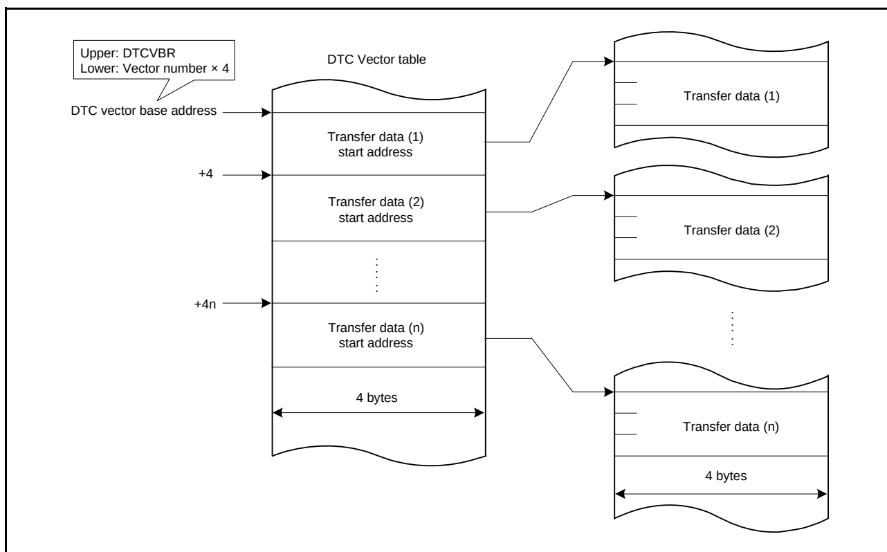
Figure 14.2 Correspondence between DTC Vector Table and Transfer Data
