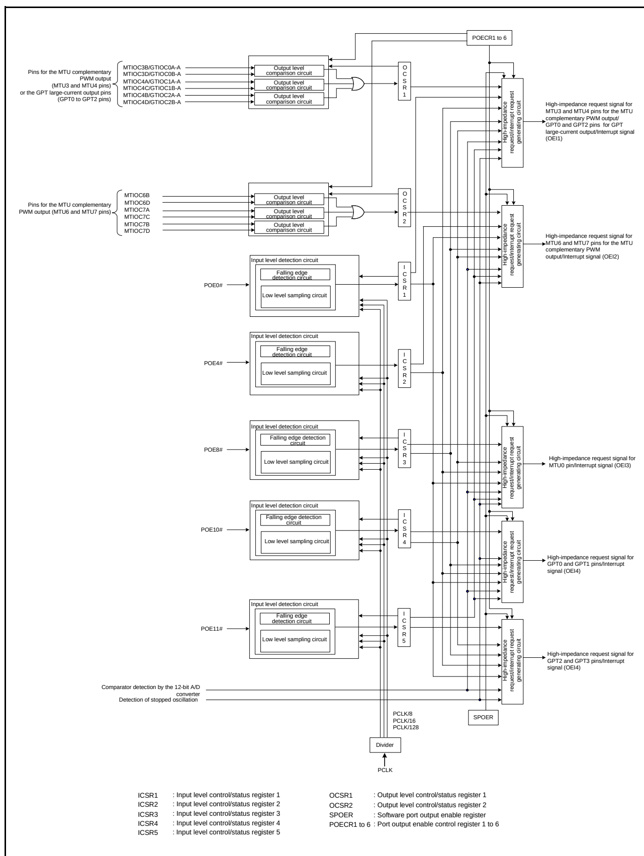
Figure 17.1 POE3 Block Diagram
