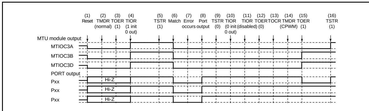
Figure 16.145 Error Occurrence in Normal Mode, Recovery in Complementary PWM Mode
