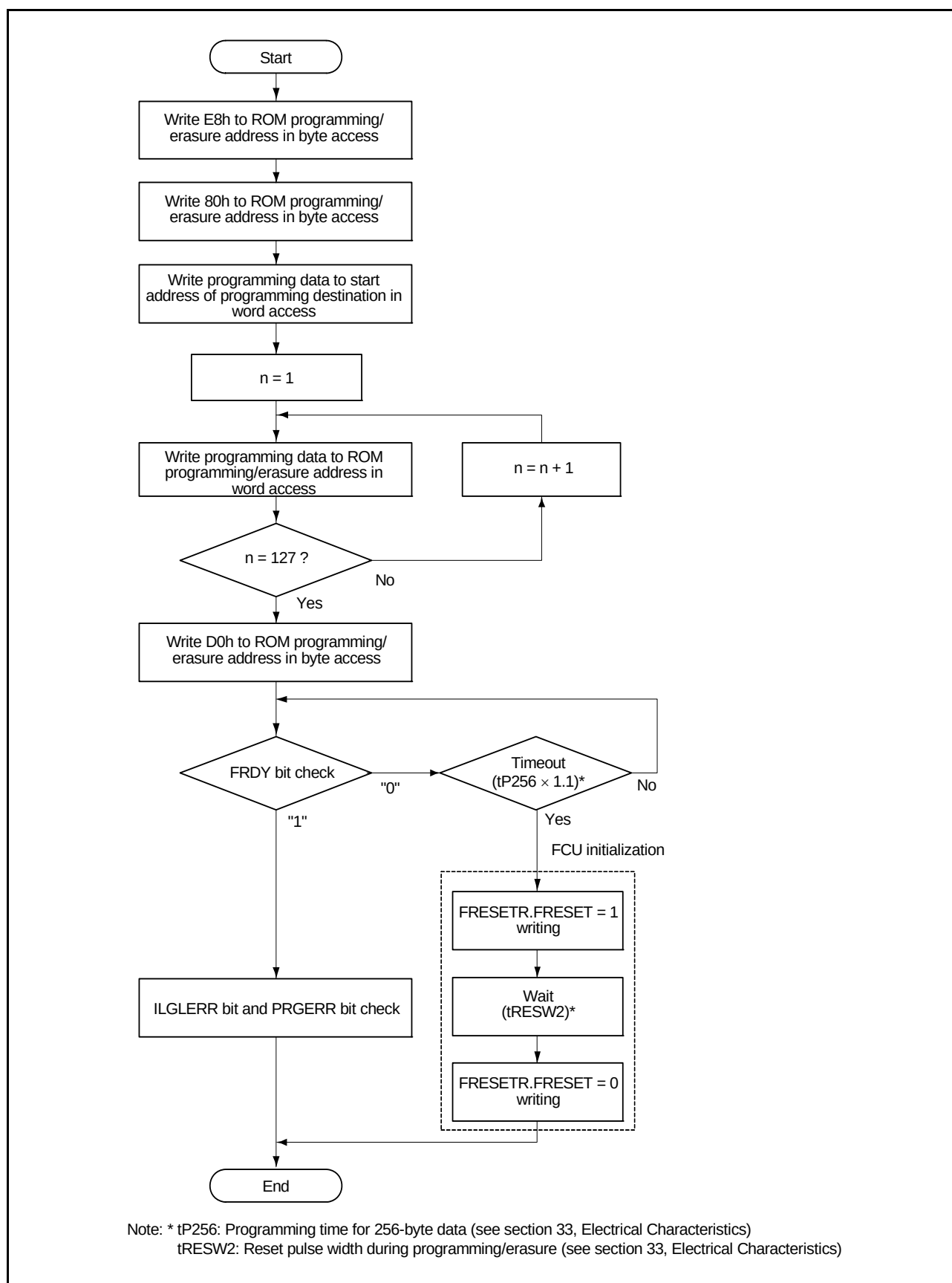
Figure 31.14 Procedure for ROM Programming
