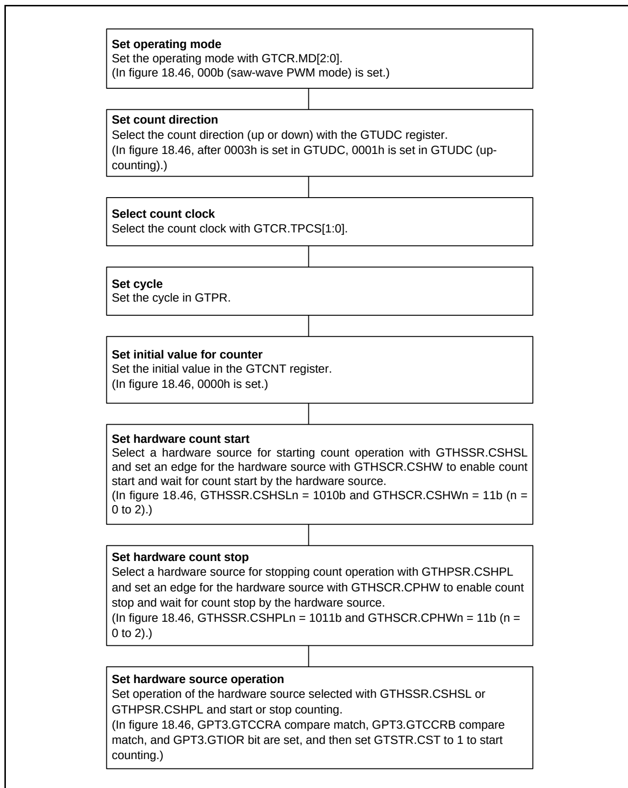
Figure 18.47 Example for Setting Count Stop Operation by Hardware Source
