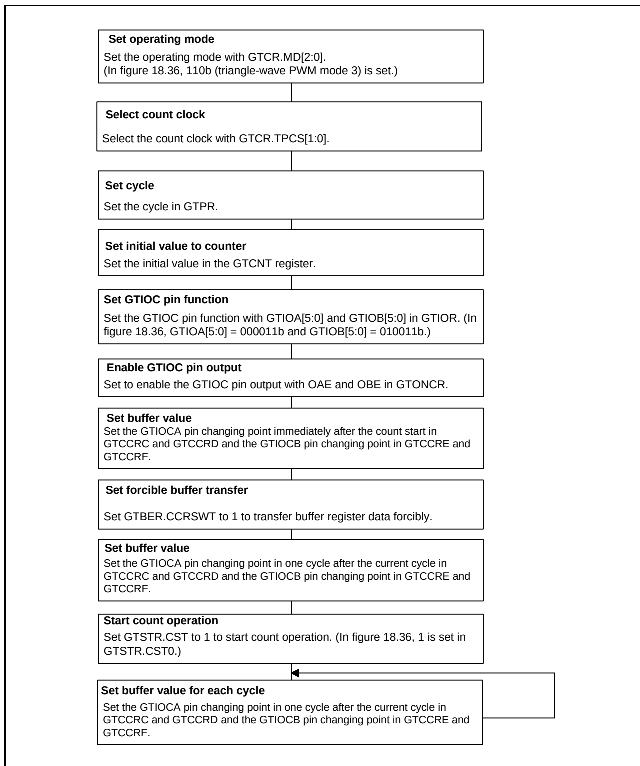
Figure 18.37 Example for Setting Triangle-Wave PWM Mode 3
