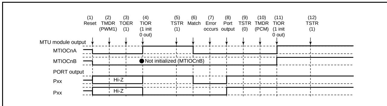
Figure 16.150 Error Occurrence in PWM Mode 1, Recovery in Phase Counting Mode
