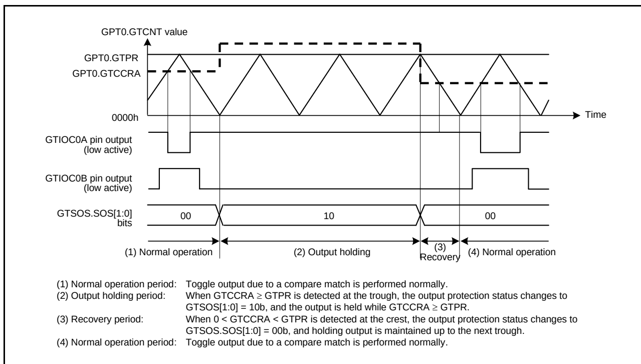
Figure 18.89 Example of Output Protection Function Operation When GTCCRA \geq GTPR is Set during Buffer Transfer at Troughs (Restored to 0 < GTCCRA < GTPR during Buffer Transfer at Crests, Active Level: Low)
