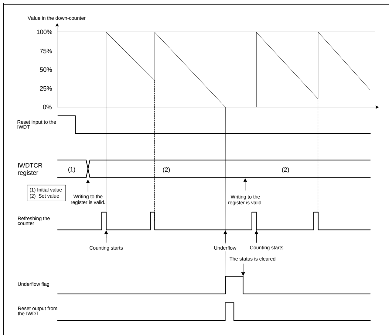
Figure 21.2 Example of Down-Counter Operation
