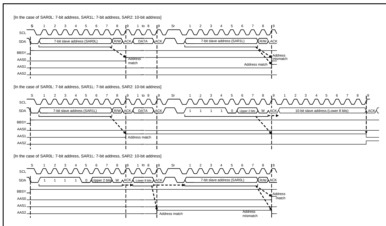
Figure 24.25 AASy Flag Set/Clear Timing with 7-Bit/10-Bit Address Formats Mixed
