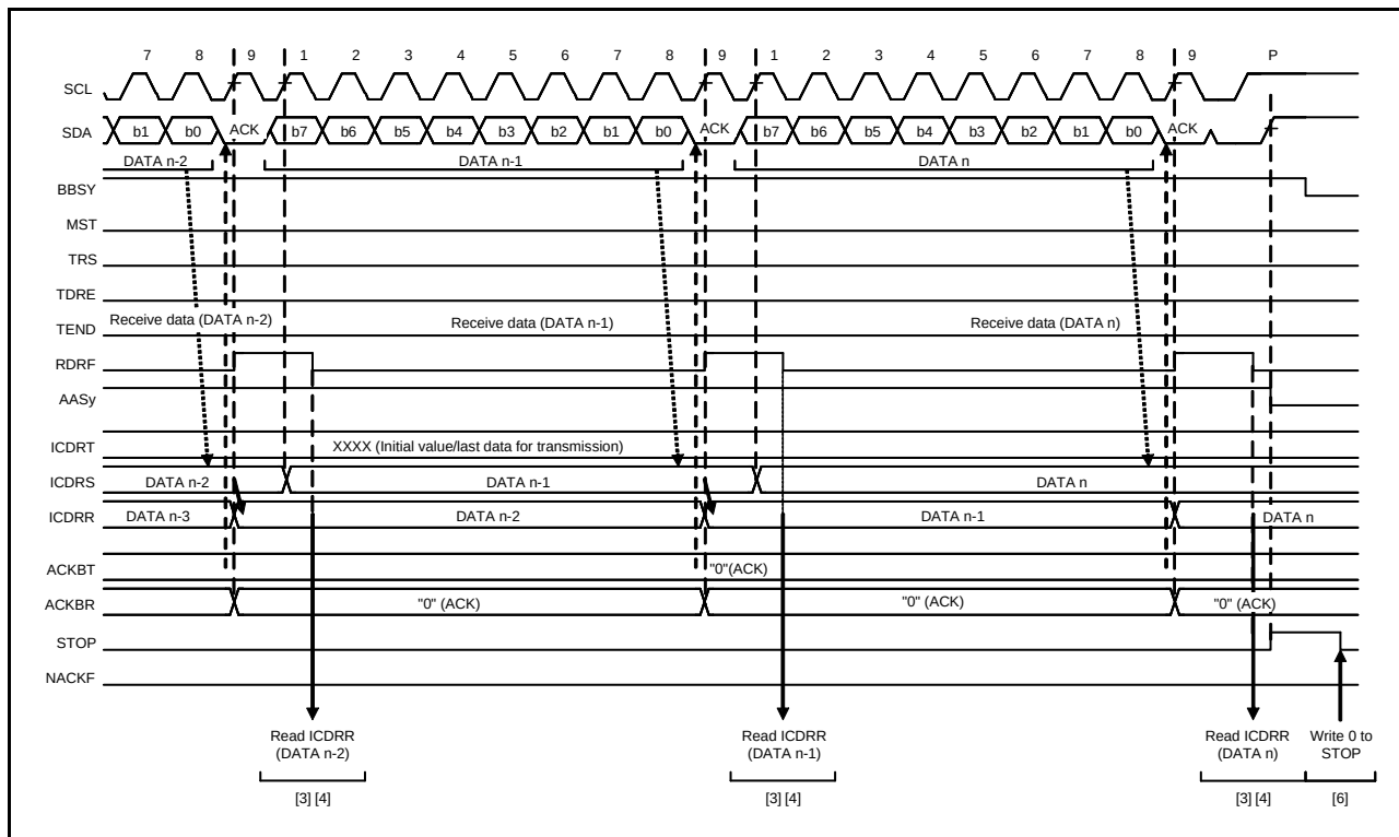
Figure 24.19 Slave Receive Operation Timing (2) (when RDRFS=0)
