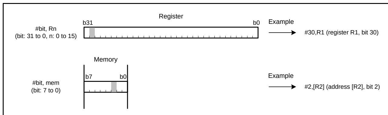
Figure 2.4 Bit
