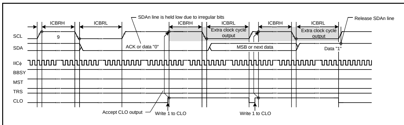
Figure 24.39 Extra SCL Clock Cycle Output Function (CLO Bit)
