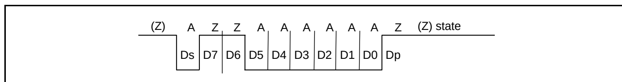
Figure 22.26 Inverse Convention (SDIR in SCMR = 1, SINV in SCMR = 1, PM in SMR = 1)
