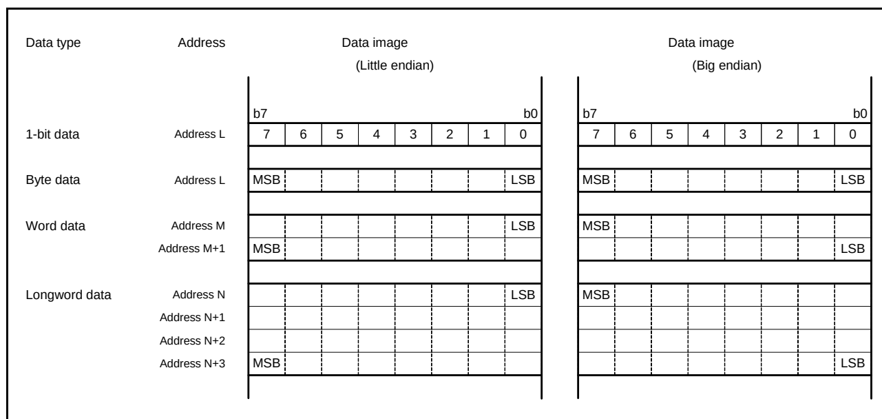
Figure 2.7 Data Arrangement in Memory
