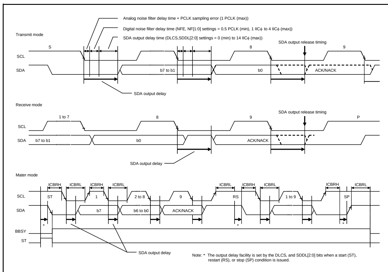
Figure 24.21 SDA Output Delay Facility
