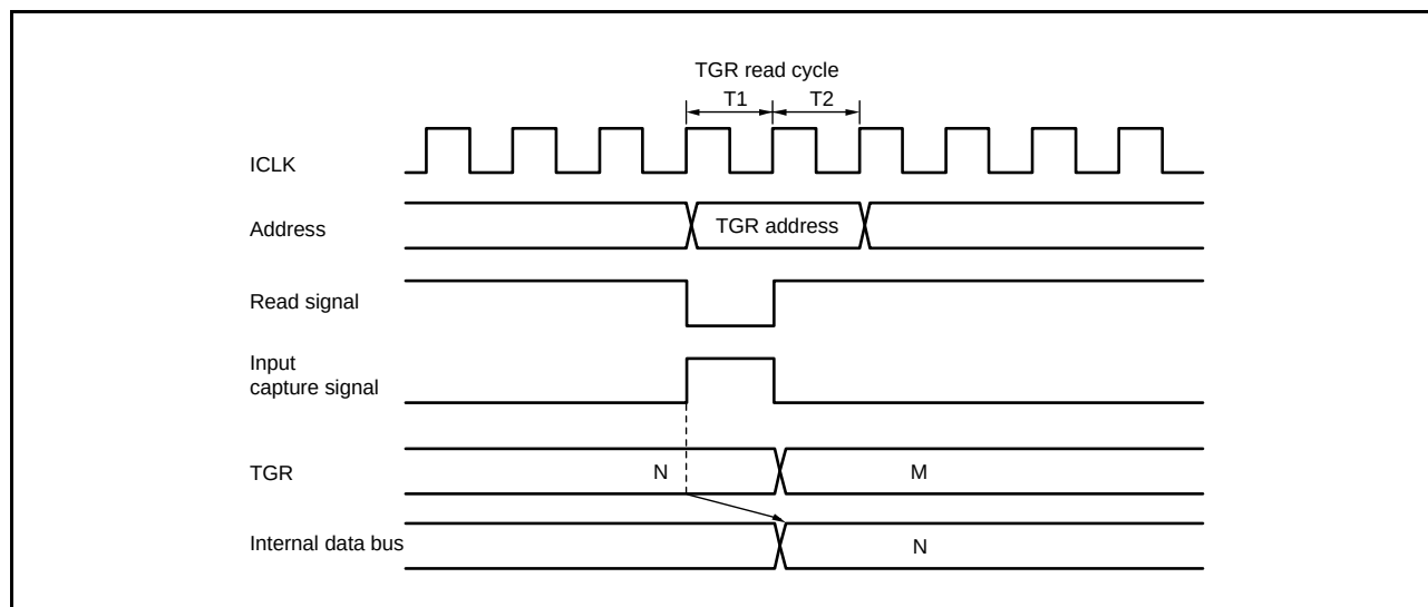
Figure 16.130 Contention between TGR Read Operation and Input Capture (MTU0 to MTU4, MTU6, and MTU7)
