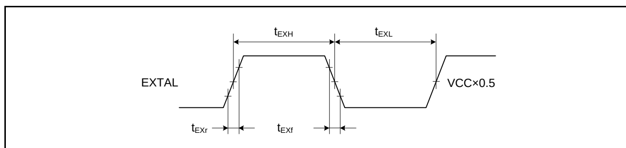
Figure 33.4 EXTAL External Input Clock Timing
