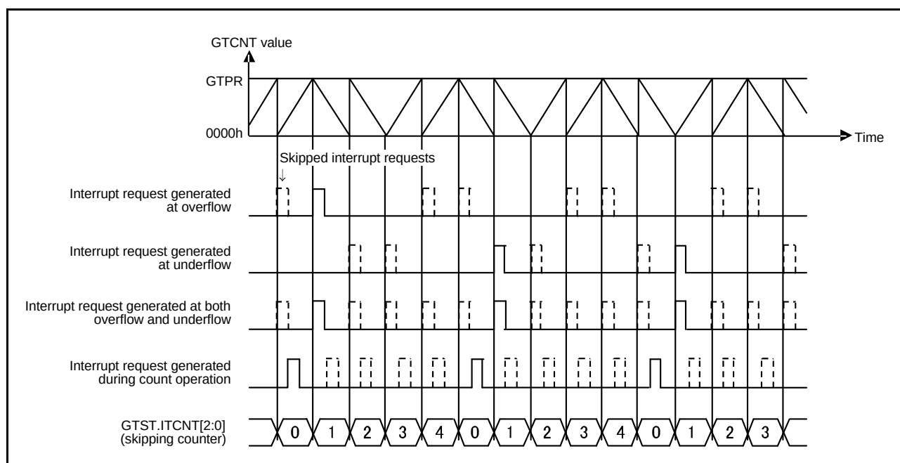
Figure 18.74 Example of Interrupt Skipping Function Operation (Saw Waves, Operation with Count Direction Changed, Counting and Skipping Both Overflows and Underflows, Skipping Count: 4)
