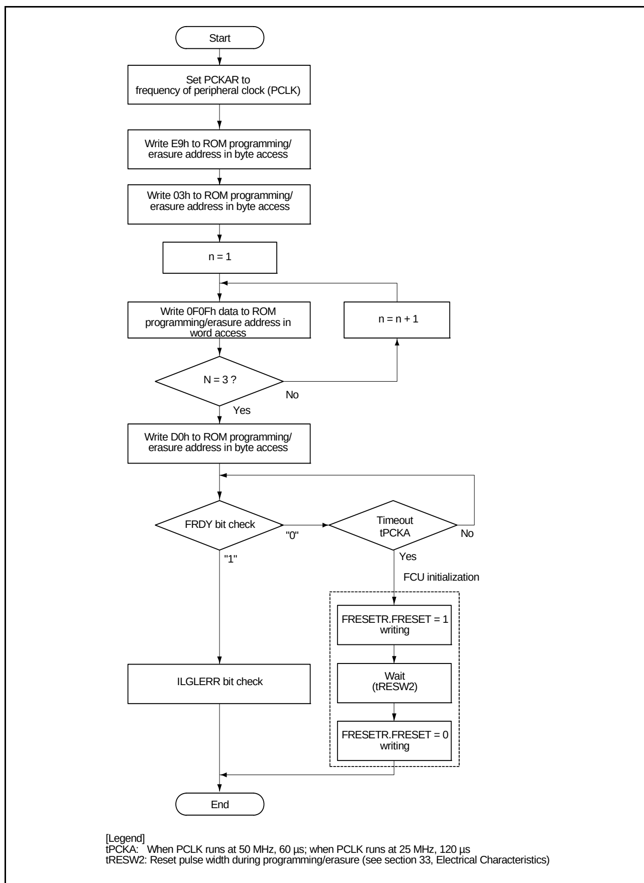
Figure 31.13 Using the Peripheral Clock Notification Command
