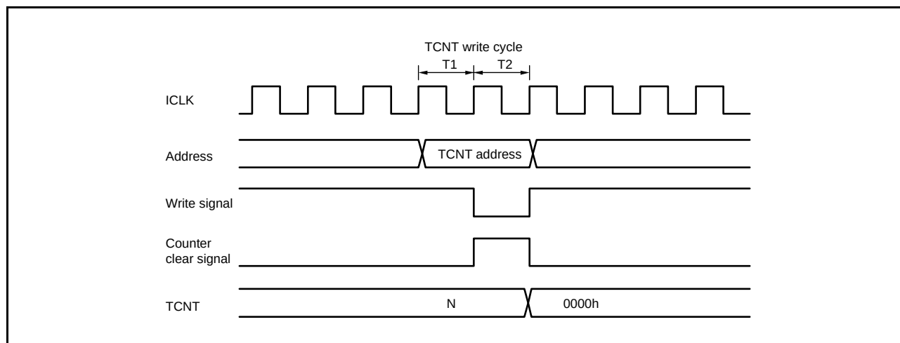
Figure 16.125 Contention between TCNT Write and Clear Operations
