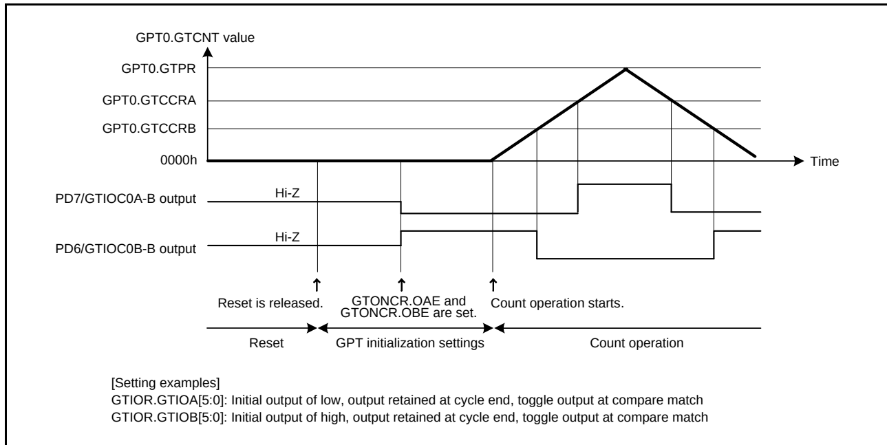
Figure 18.92 Example of Pin Settings after Reset
