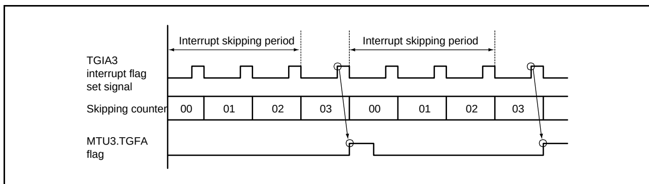
Figure 16.79 Example of Interrupt Skipping Function 1
