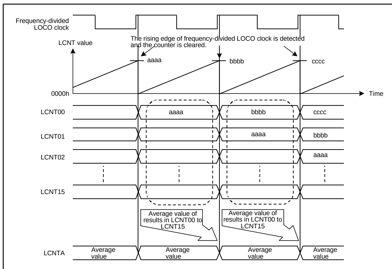
Figure 18.77 Example of LOCO Count Function Operation
