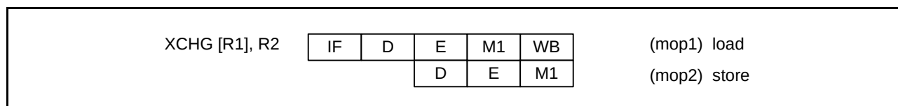
Figure 2.18 XCHG Instruction (Memory Source Operand)
