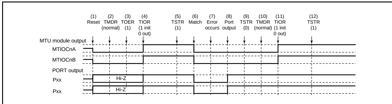
Figure 16.141 Error Occurrence in Normal Mode, Recovery in Normal Mode
