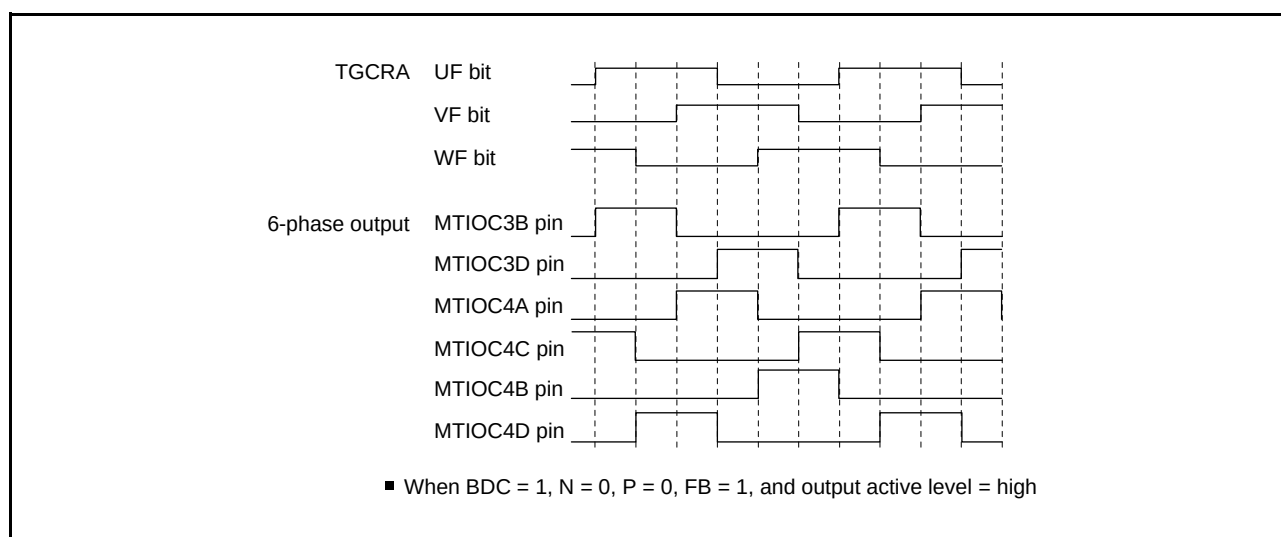
Figure 16.72 Example of Output Phase Switching through UF, VF, and WF Bit Settings (1)
