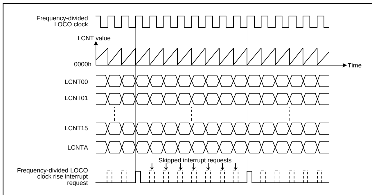
Figure 18.79 Example of LOCO Count Skipping Function Operation (Skipping Count: 7, Count Result not Skipped)
