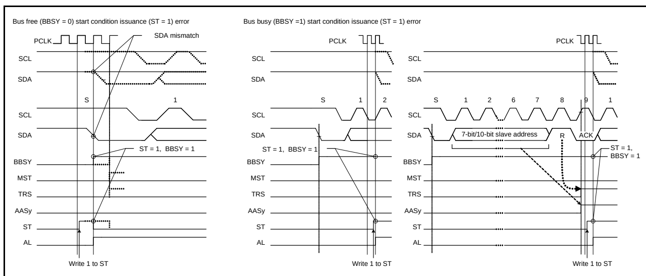
Figure 24.33 Arbitration Lost when a Start Condition is Issued (MALE = 1)
