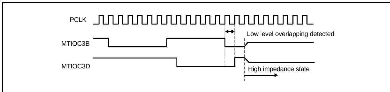
Figure 17.5 Output-Level Compare Operation
