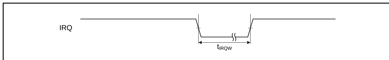
Figure 33.7 IRQ Interrupt Input Timing
