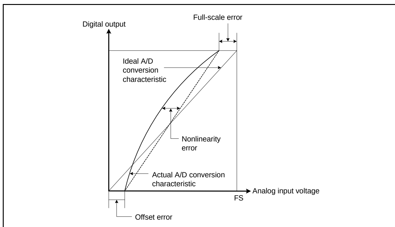
Figure 29.8 A/D Conversion Accuracy Definitions (2)
