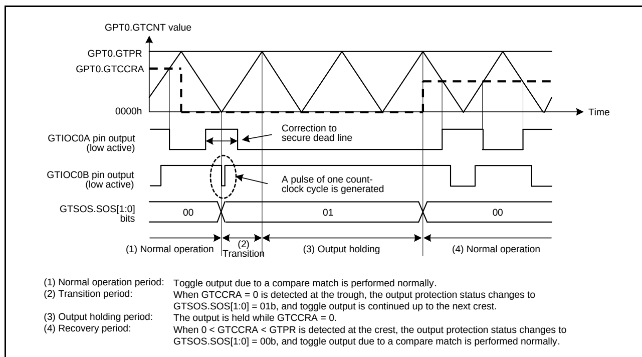
Figure 18.87 Example of Output Protection Function Operation When GTCCRA is Set to 0 during Buffer Transfer at Crests (Restored to 0 < GTCCRA < GTPR during Buffer Transfer at Crests, Active Level: Low)
