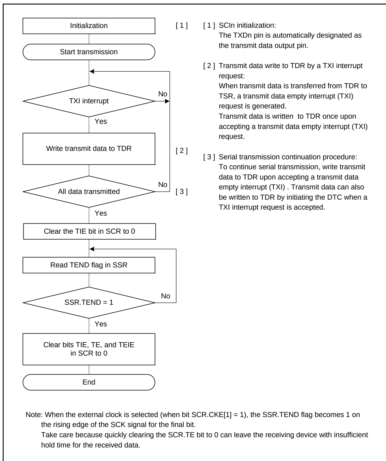
Figure 22.19 Example of Serial Transmission Flowchart (Clock Synchronous Mode)
