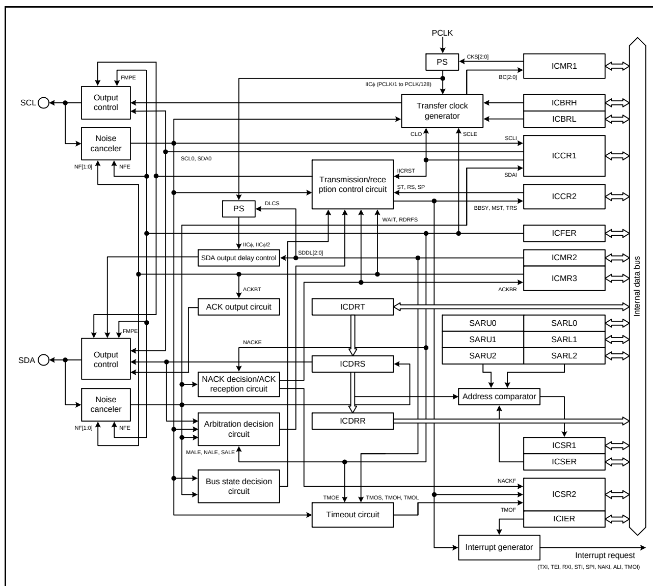
Figure 24.1 Block Diagram of RIIC
