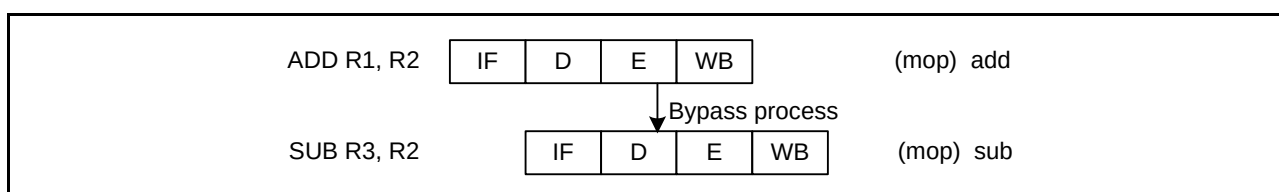
Figure 2.24 Bypass Process
