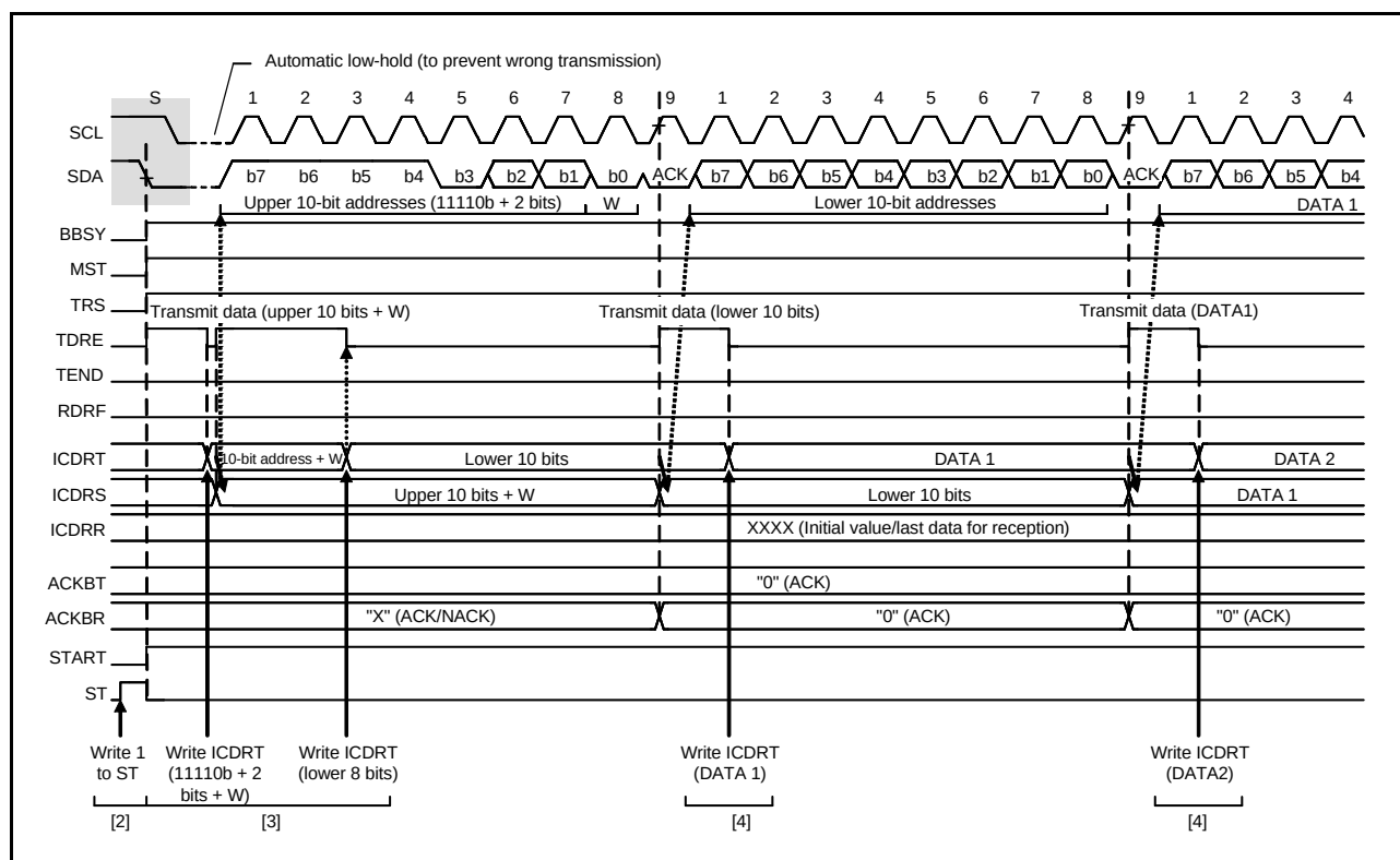
Figure 24.8 Master Transmit Operation Timing (2) (10-Bit Address Format)
