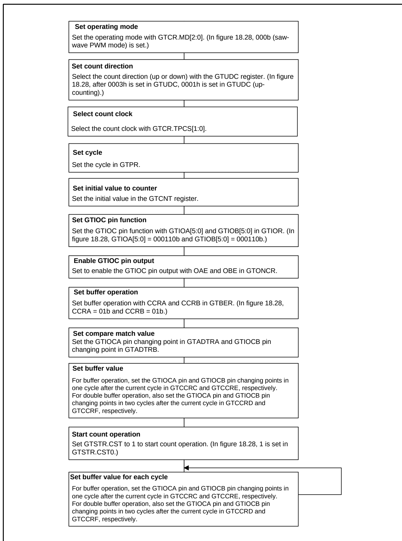
Figure 18.29 Example for Setting Saw-Wave PWM Mode
