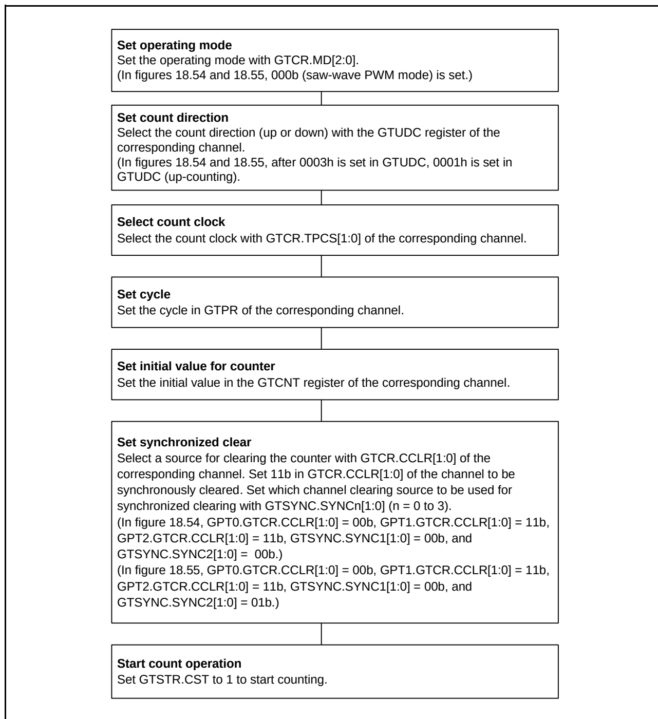
Figure 18.56 Example for Setting Synchronized Clear Operation
