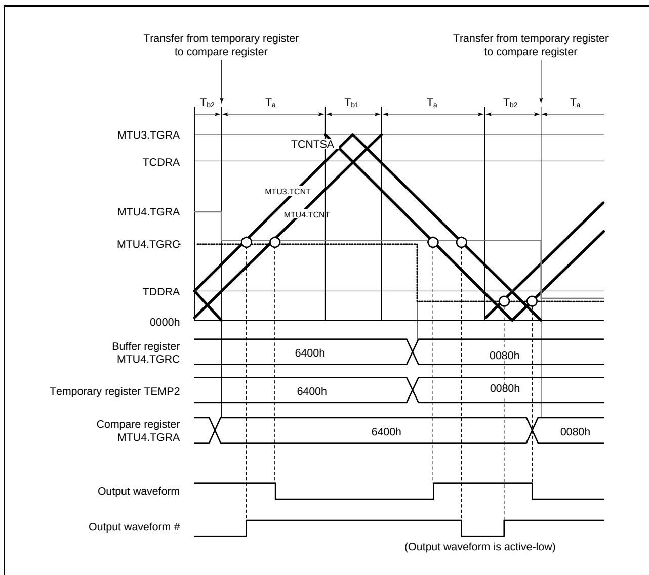
Figure 16.41 Example of Operation in Complementary PWM Mode (MTU3 and MTU4)
