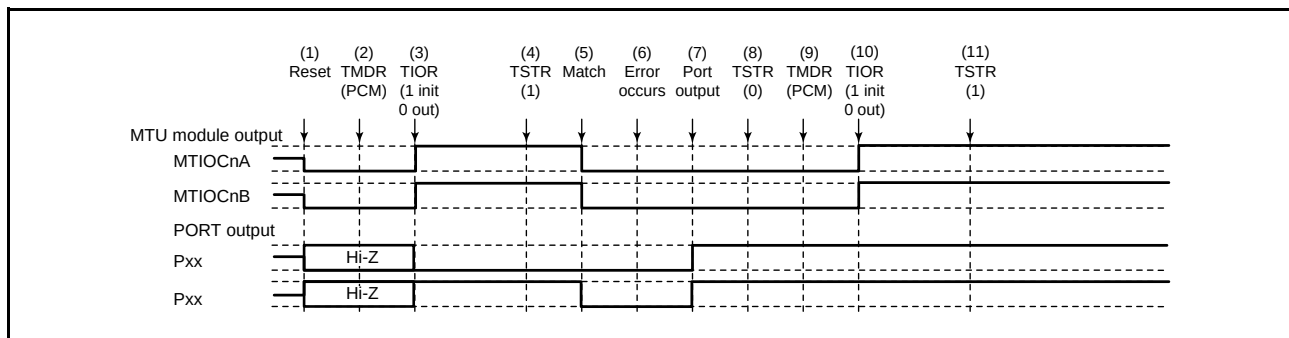
Figure 16.160 Error Occurrence in Phase Counting Mode, Recovery in Phase Counting Mode
