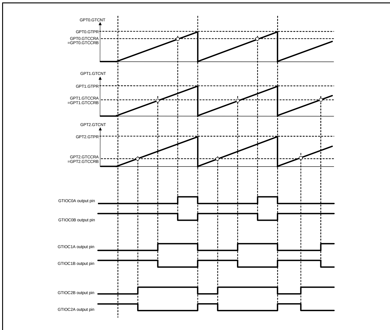
Figure 18.64 Example of Three-Phase Saw-Wave Complementary PWM Output
