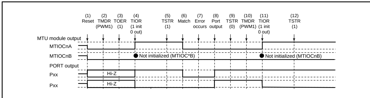
Figure 16.148 Error Occurrence in PWM Mode 1, Recovery in PWM Mode 1
