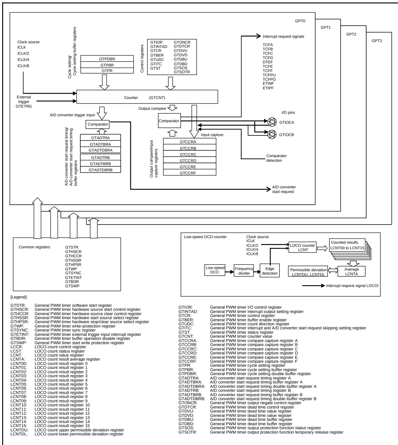
Figure 18.1 Block Diagram of GPT
