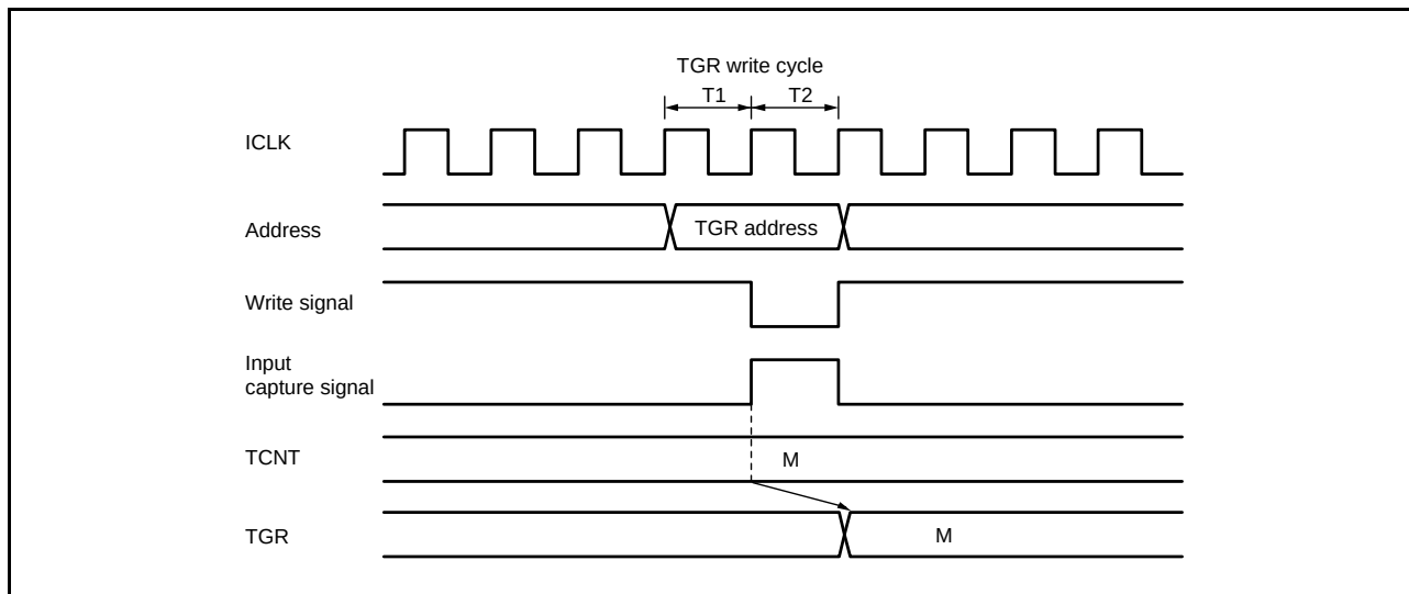
Figure 16.132 Contention between TGR Write Operation and Input Capture (MTU0 to MTU4, MTU6, and MTU7)
