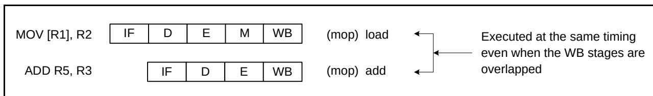
Figure 2.25 When WB Stages for the Memory Load and for the Operation are Overlapped
