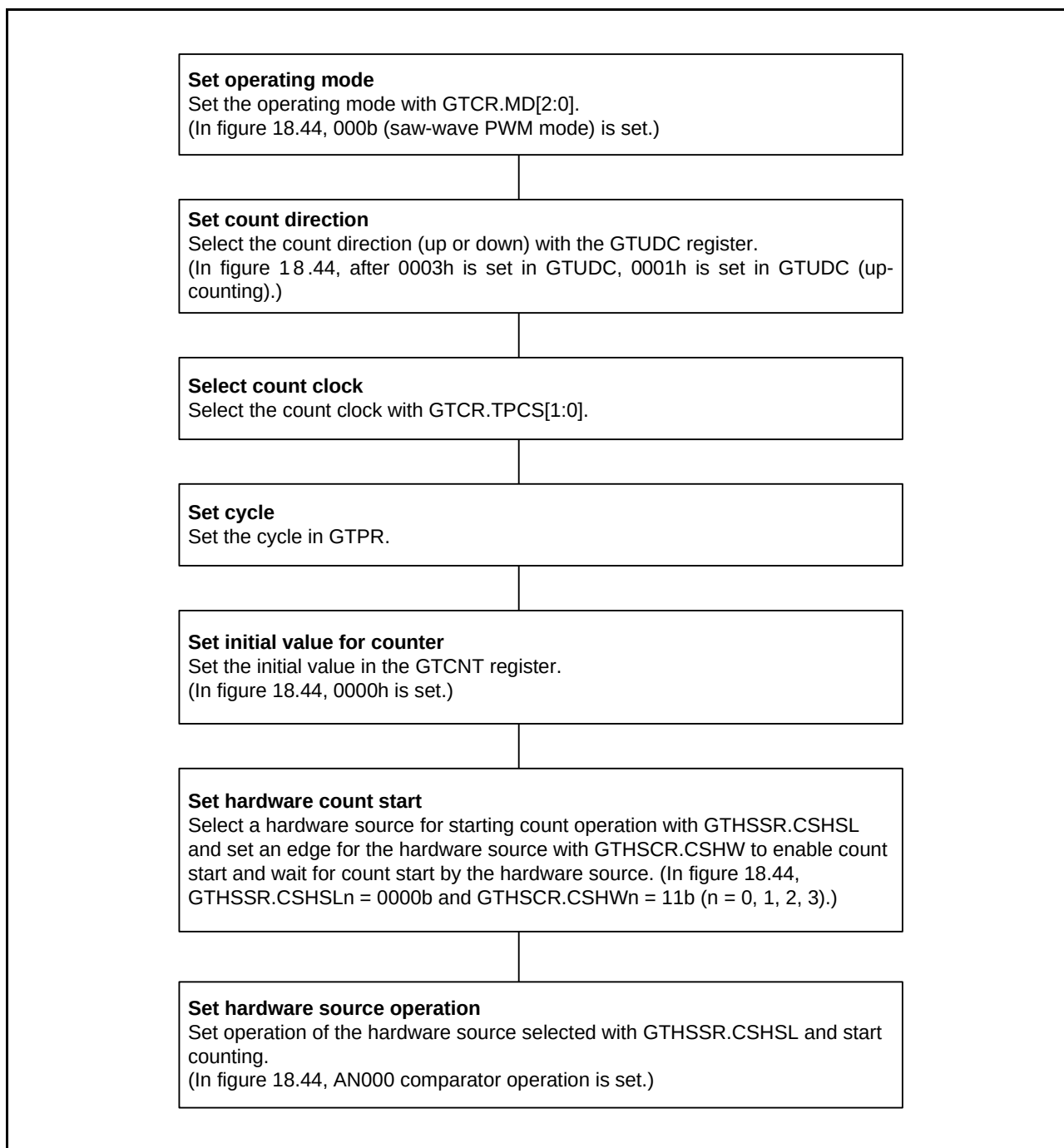
Figure 18.45 Example for Setting Count Start Operation by Hardware Source
