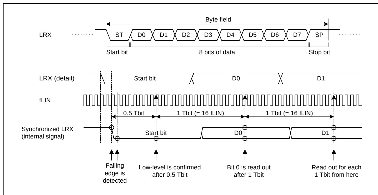
Figure 27.8 Data Reception Timing
