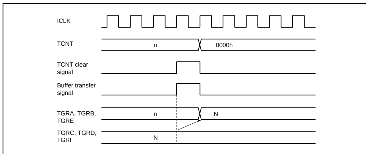
Figure 16.113 Buffer Operation Timing (when TCNT Cleared)
