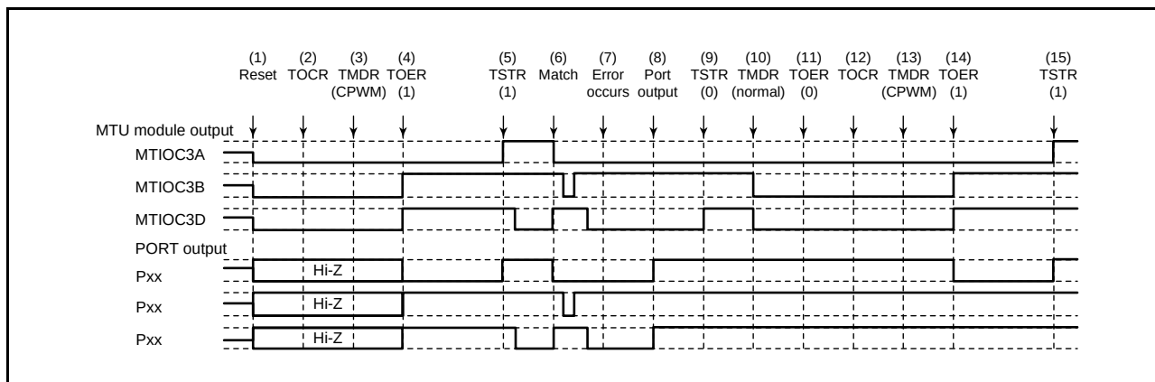
Figure 16.164 Error Occurrence in Complementary PWM Mode, Recovery in Complementary PWM Mode (2)
