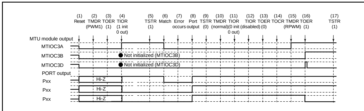
Figure 16.152 Error Occurrence in PWM Mode 1, Recovery in Reset-Synchronized PWM Mode
