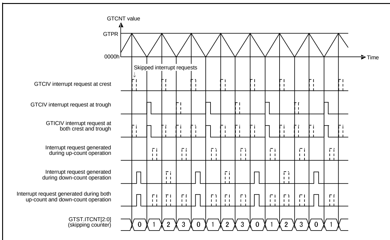
Figure 18.72 Example of Interrupt Skipping Function Operation (Triangle Waves, Counting and Skipping Both Troughs and Crests, Skipping Count: 3, Skipping Started at Up-Counting)
