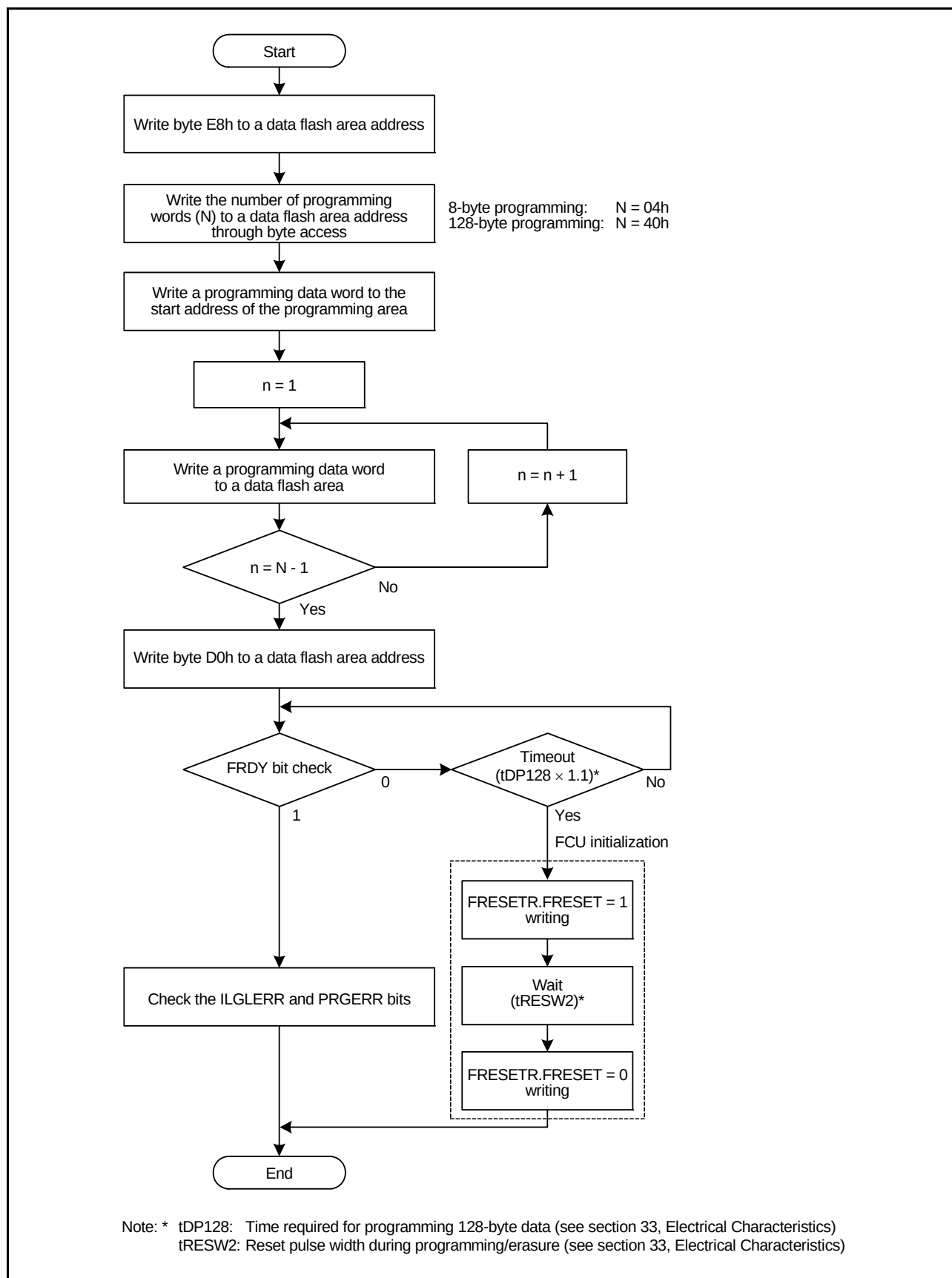
Figure 32.5 Procedure for Data Flash Programming
