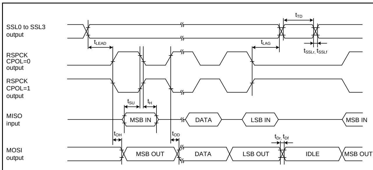
Figure 33.13 RSPI Timing (Master, CPHA = 1)
