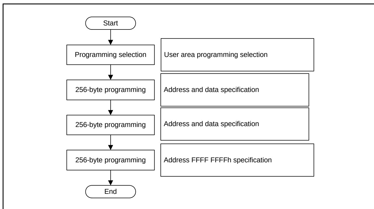
Figure 31.31 Procedure for ROM Programming in Boot Mode
