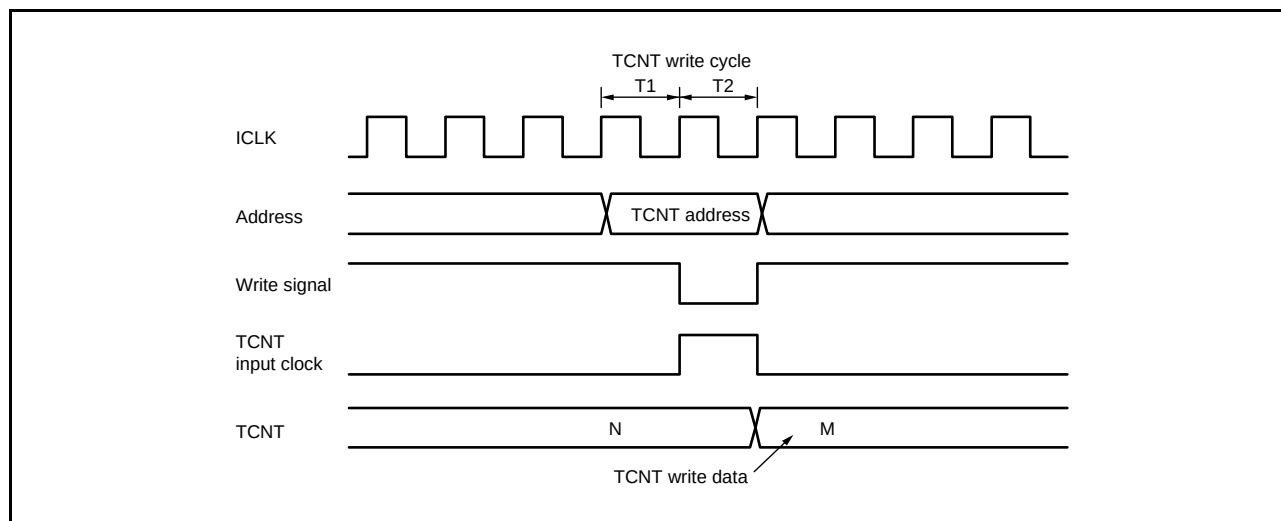
Figure 16.126 Contention between TCNT Write and Increment Operations
