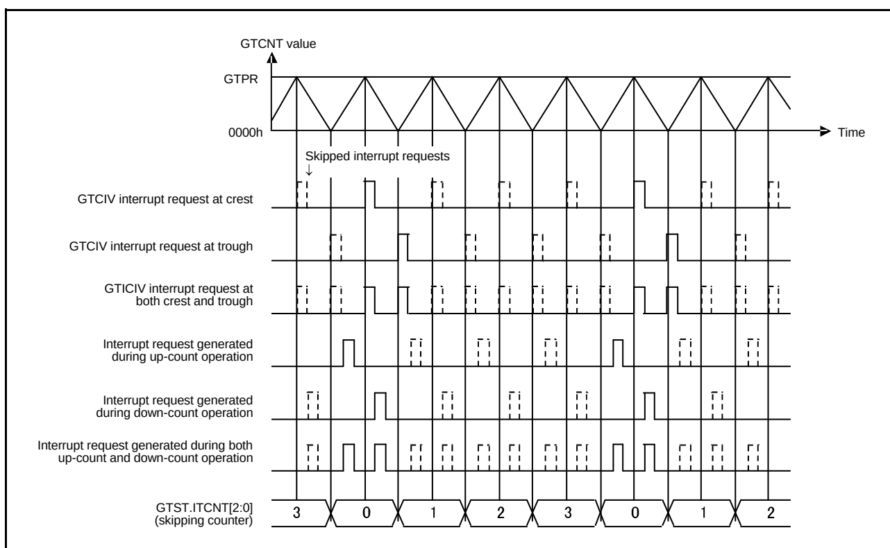
Figure 18.70 Example of Interrupt Skipping Function Operation (Triangle Waves, Counting and Skipping Troughs, Skipping Count: 3)
