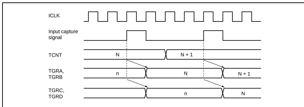
Figure 16.112 Buffer Operation Timing (Input Capture)
