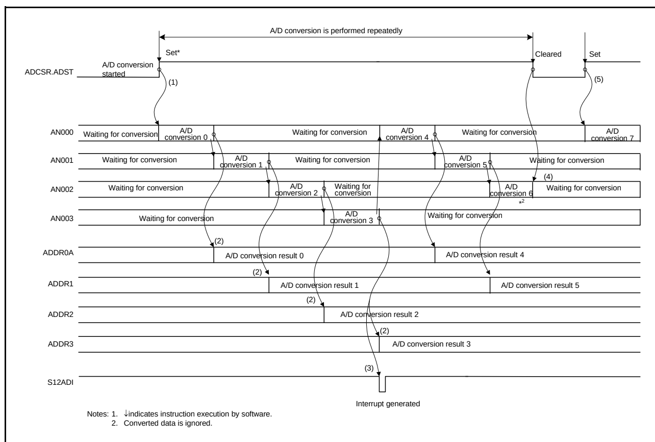
Figure 28.6 Example of Operation in Continuous Scan Mode (ADCER.SHBY = 1: Sample-and-Hold Circuit Dedicated for Channel is Not Used)
