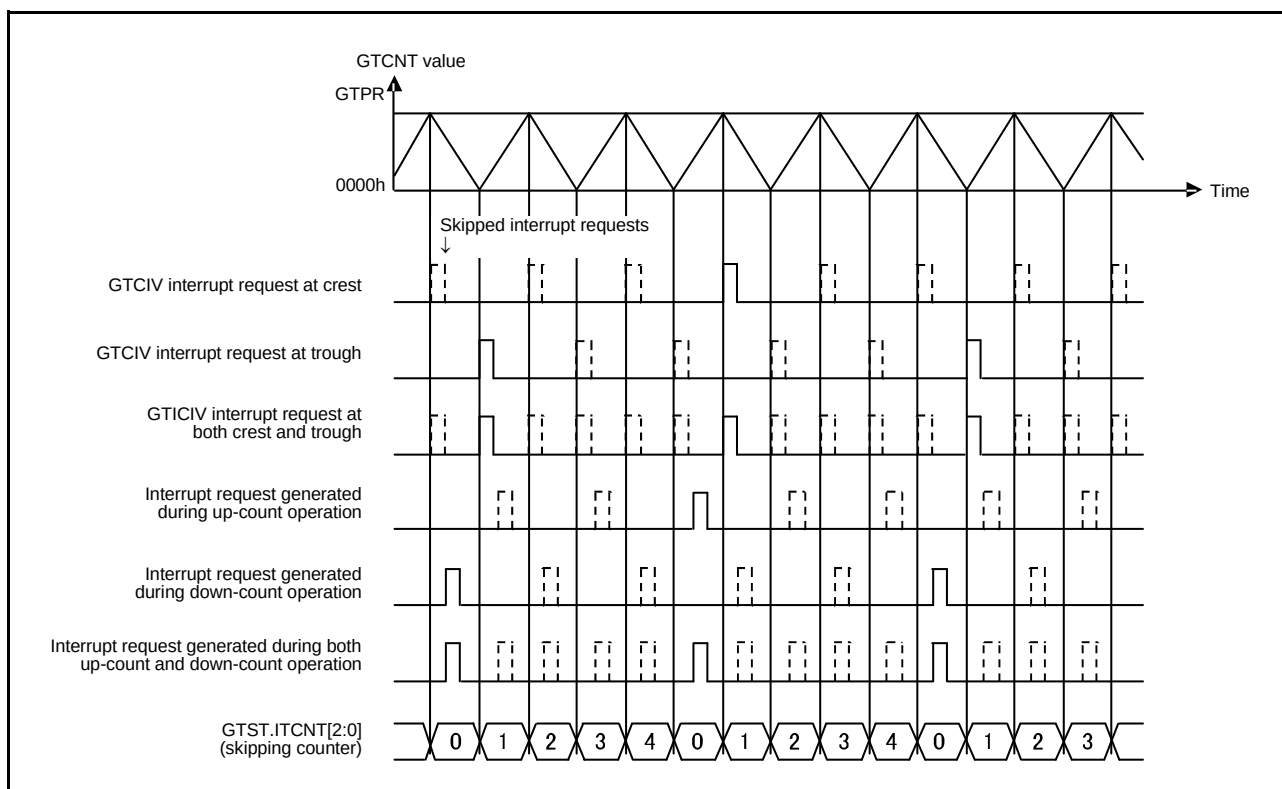
Figure 18.71 Example of Interrupt Skipping Function Operation (Triangle Waves, Counting and Skipping Both Troughs and Crests, Skipping Count: 4)
