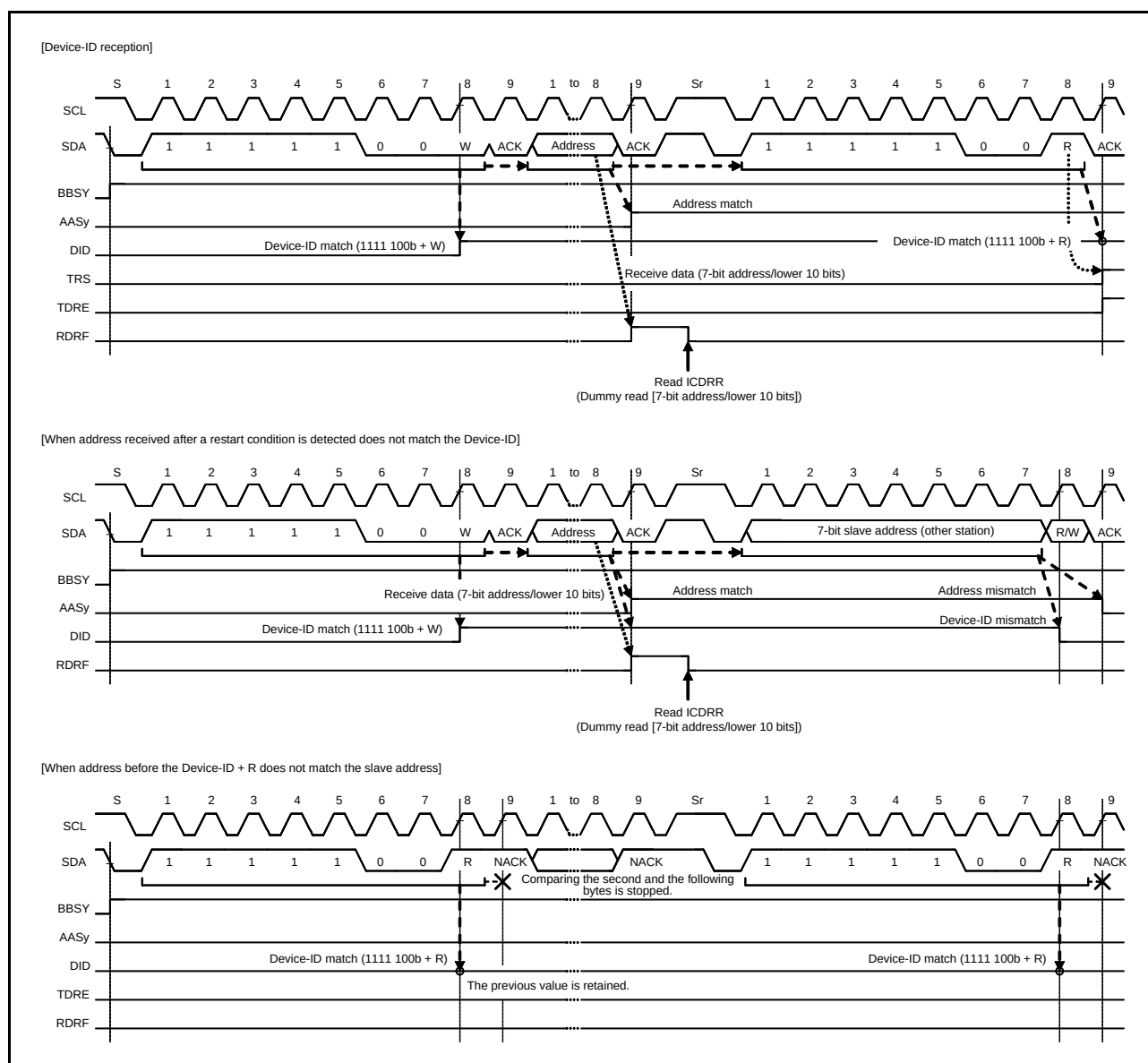
Figure 24.27 AASy/DID Flag Set/Clear Timing during Reception of Device-ID
