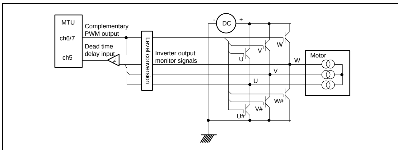
Figure 16.99 Example of Motor Control Circuit Configuration
