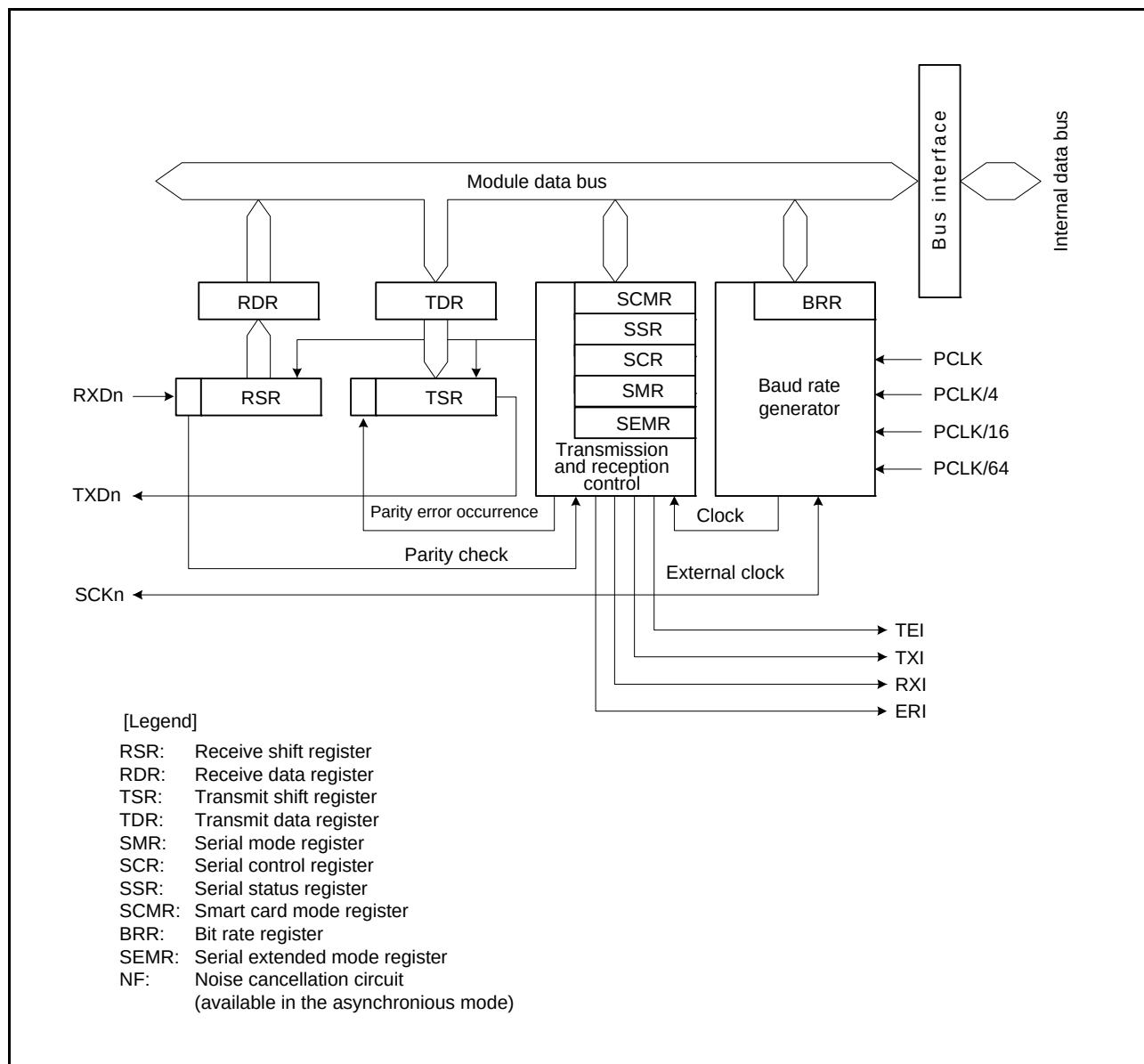
Figure 22.1 Block Diagram of SCI0 to SCI2
