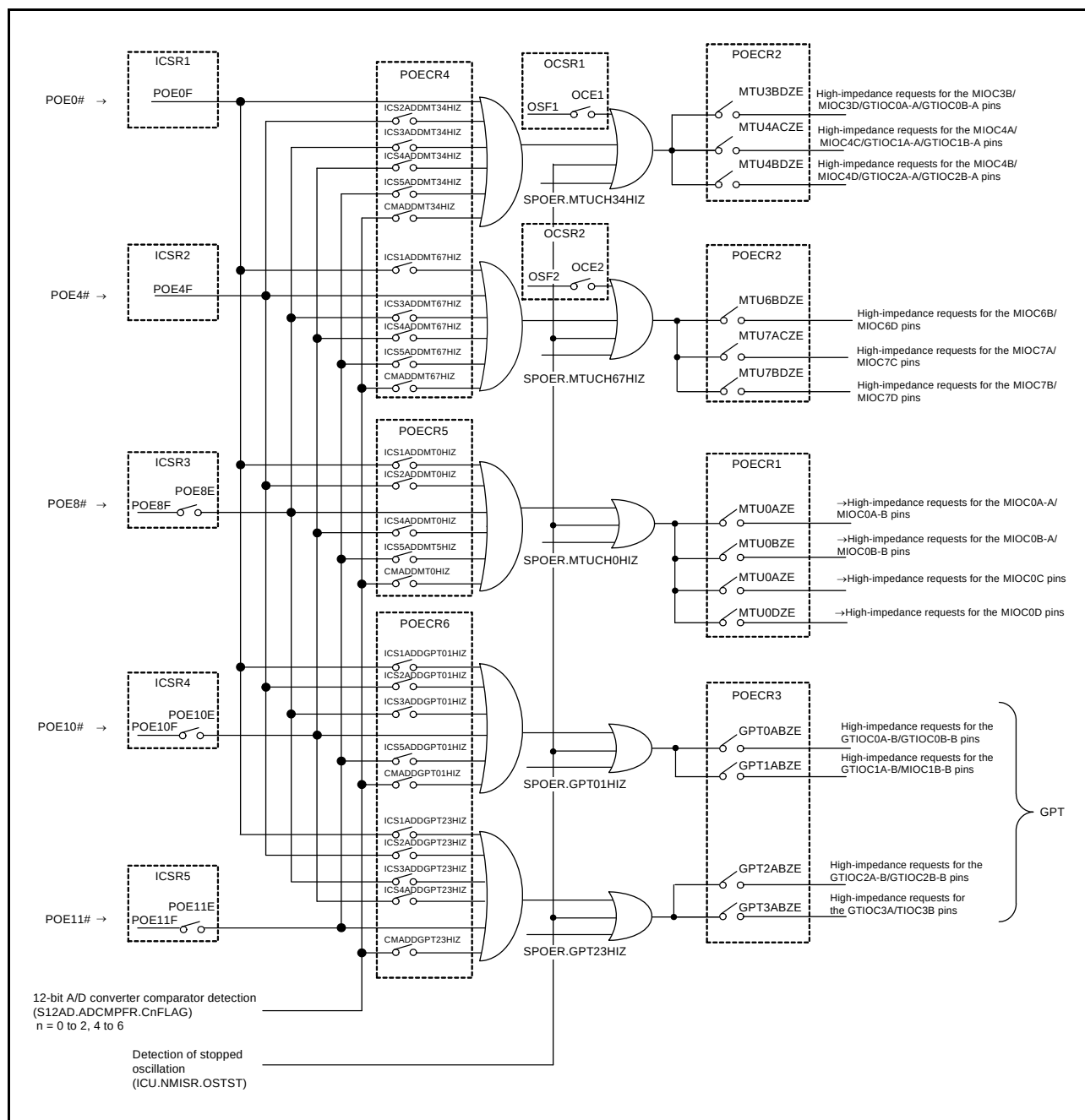
Figure 17.2 Target Pins and Conditions for High-Impedance Control
