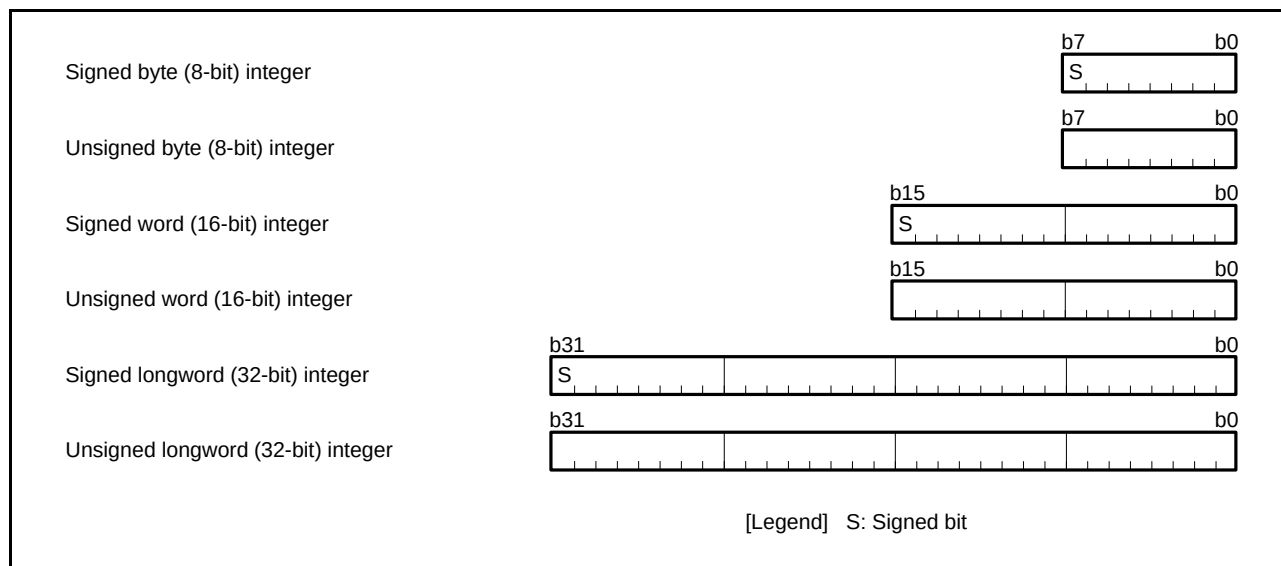
Figure 2.2 Integer
