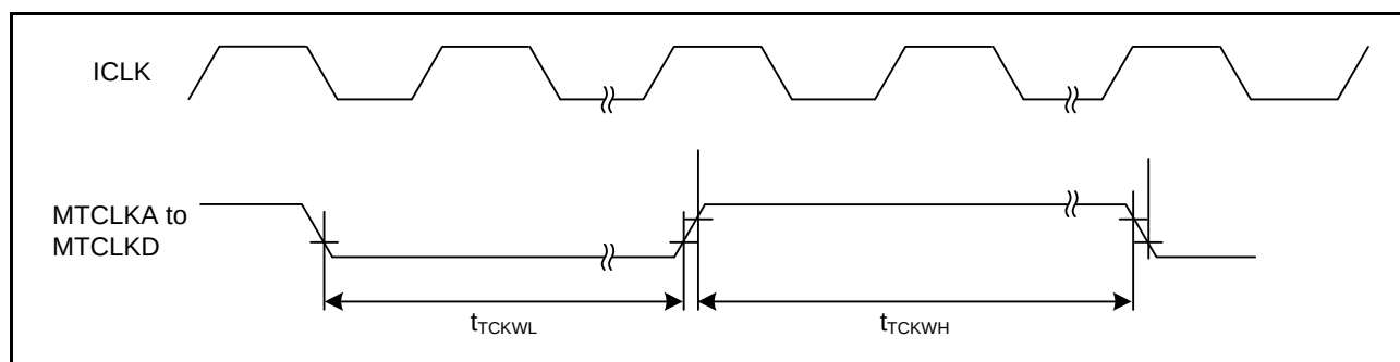
Figure 33.17 MTU3 Clock Input Timing
