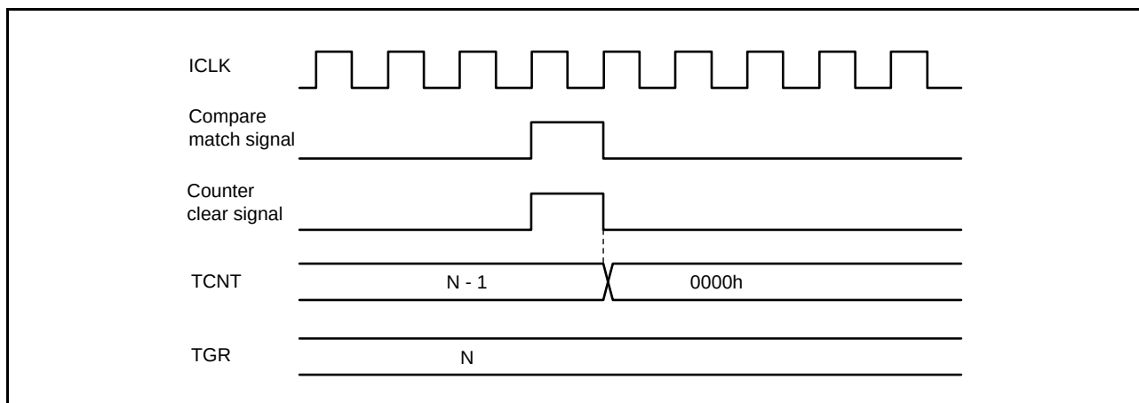
Figure 16.109 Counter Clear Timing (Compare Match) (MTU5)
