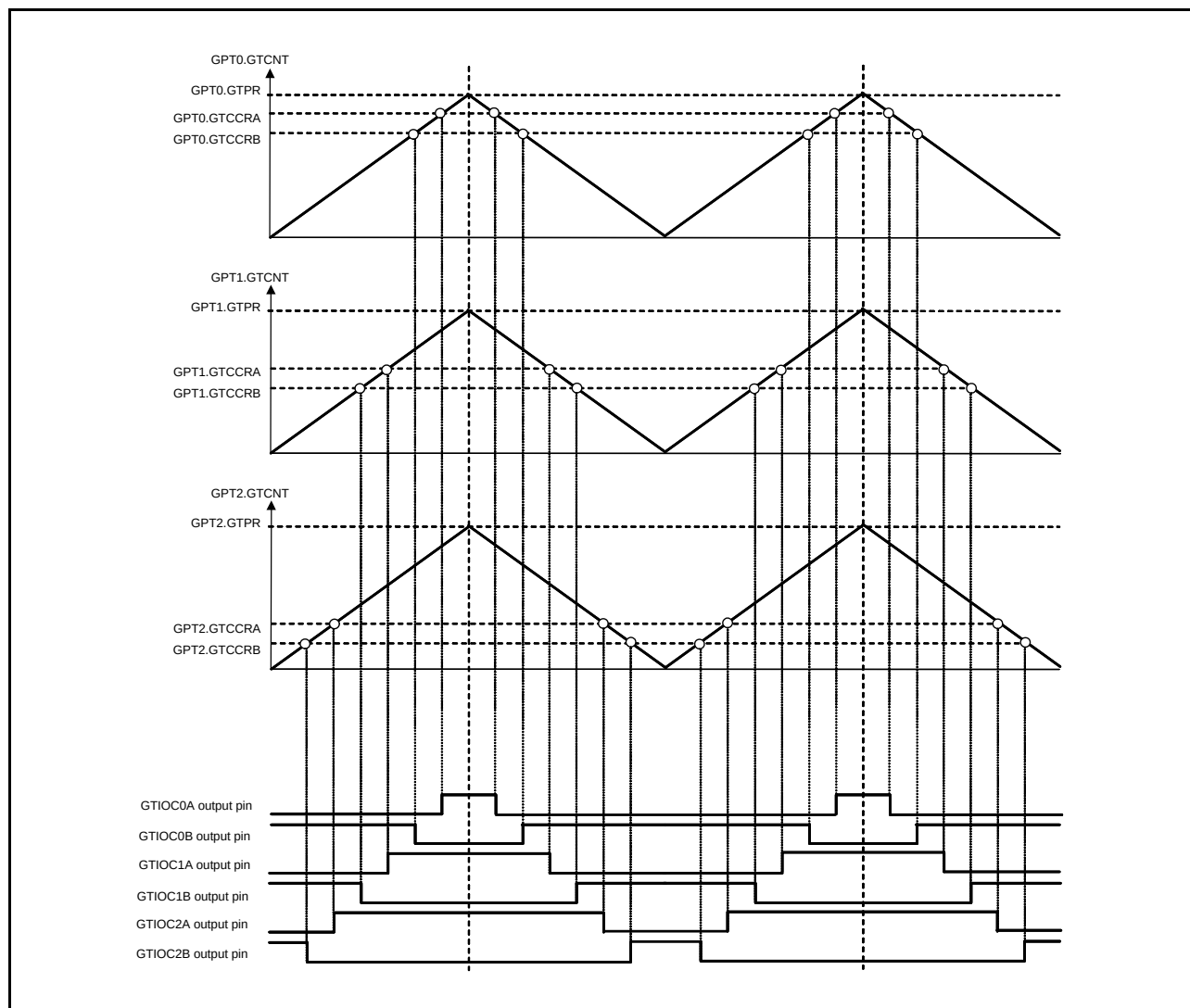
Figure 18.66 Example of Three-Phase Triangle-Wave Complementary PWM Output
