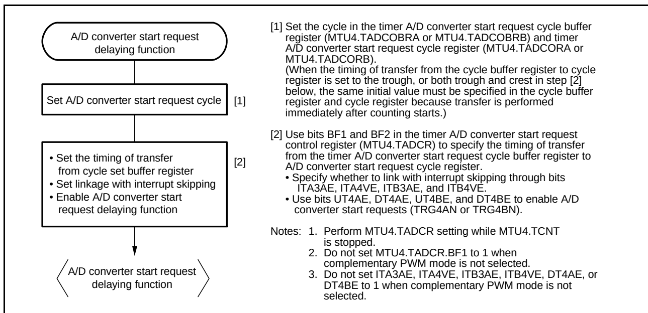
Figure 16.83 Example of Procedure for Specifying A/D Converter Start Request Delaying Function
