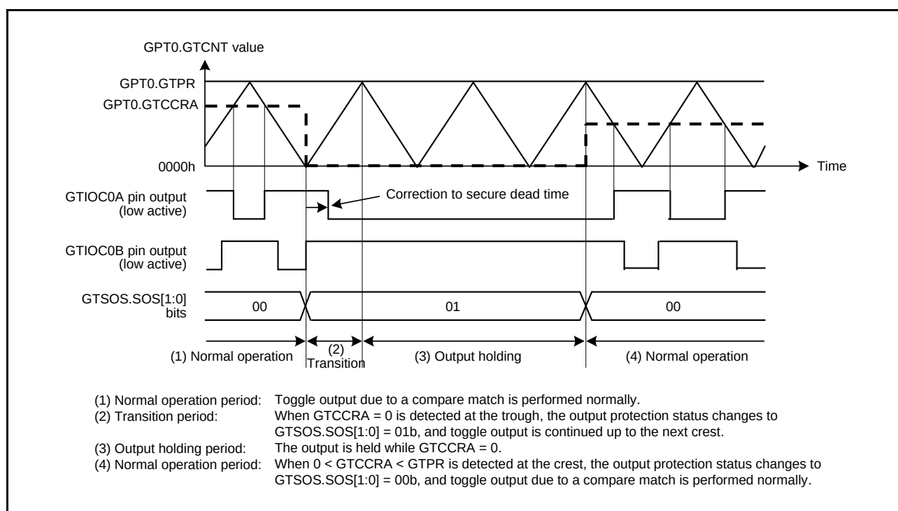
Figure 18.85 Example of Output Protection Function Operation When GTCCRA is Set to 0 during Buffer Transfer at Troughs (Restored to 0 < GTCCRA < GTPR during Buffer Transfer at Crests, Active Level: Low)
