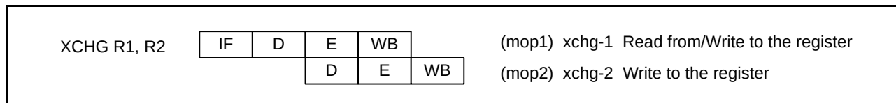
Figure 2.17 XCHG Instruction (Registers)
