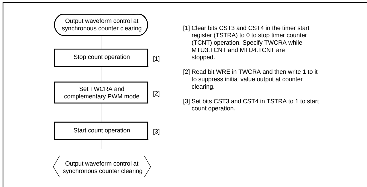
Figure 16.58 Example of Procedure for Setting Output Waveform Control at Synchronous Counter Clearing in Complementary PWM Mode (MTU3 and MTU4)
