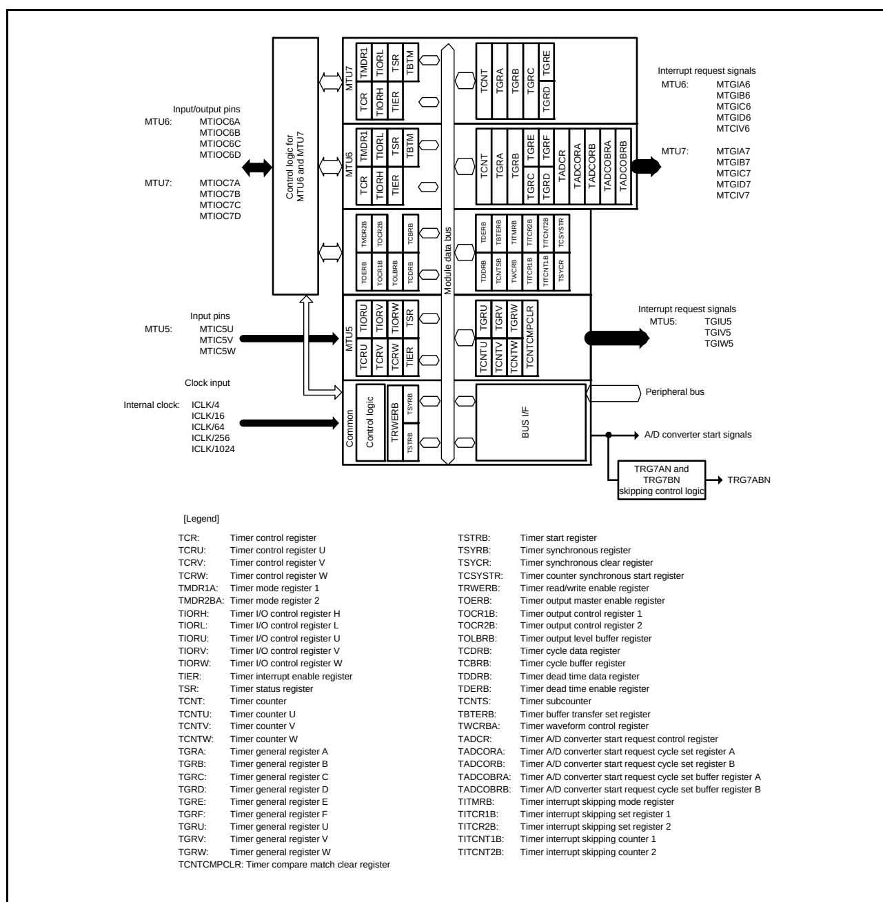
Figure 16.2 Block Diagram of MTU (MTU5 to MTU7)
