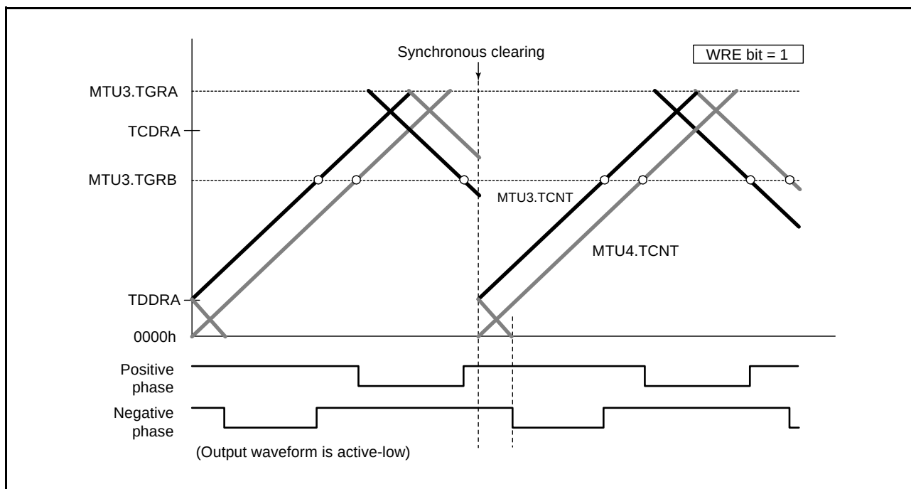
Figure 16.61 Example of Synchronous Clearing in Dead Time during Down-Counting (Timing (8) in Figure 16.57; Bit WRE of TWCRB is 1)
