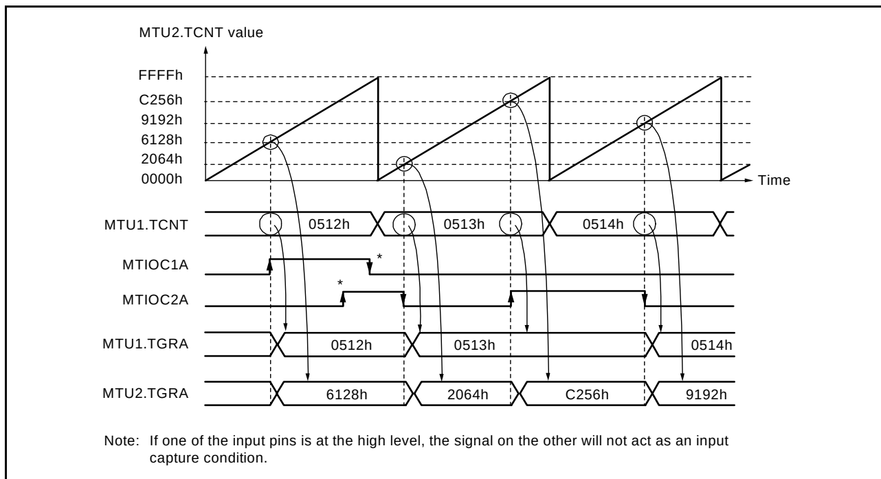
Figure 16.24 Cascaded Operation Example (c)
