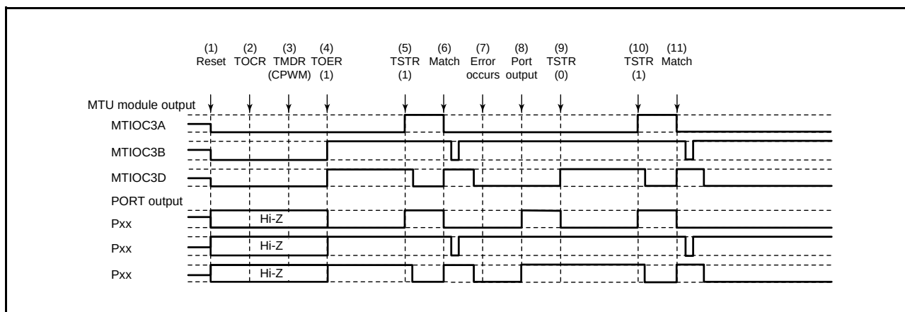
Figure 16.163 Error Occurrence in Complementary PWM Mode, Recovery in Complementary PWM Mode (1)
