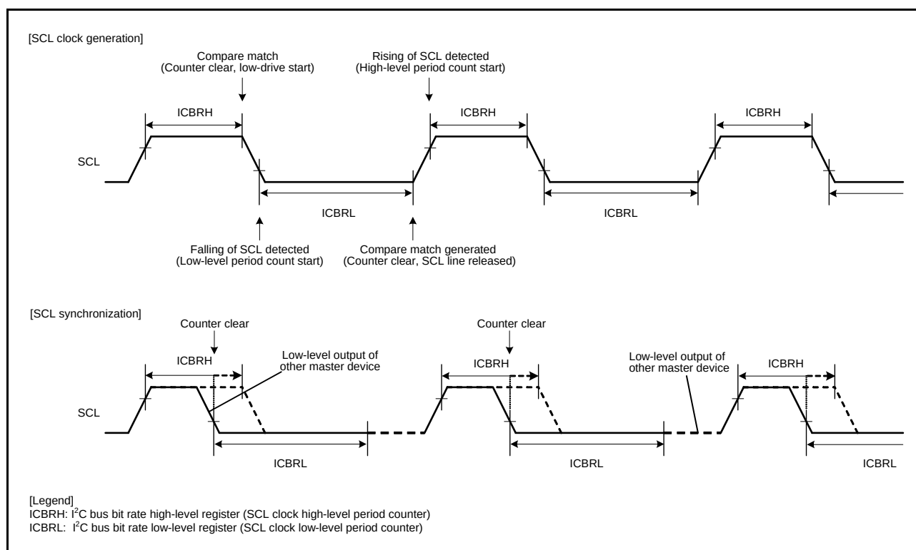
Figure 24.20 Generation and Synchronization of the SCL Signal from the RIIC
