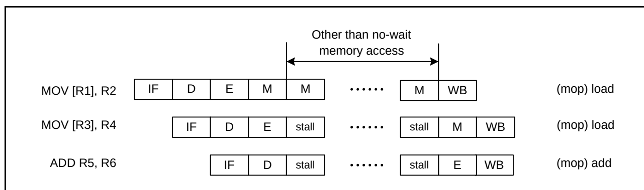
Figure 2.21 When an Instruction which Requires more than One Cycle for its Operand Access is Executed
