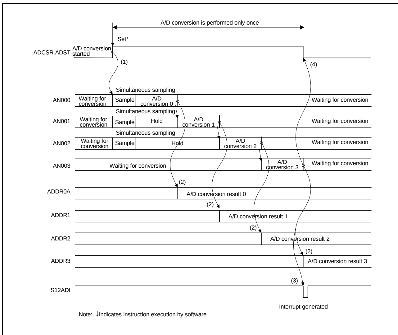
Figure 28.3 Example of Operation in Single-Cycle Scan Mode (ADCER.SHBYP = 0: Sample-and-Hold Circuit Dedicated for Channel is Used)
