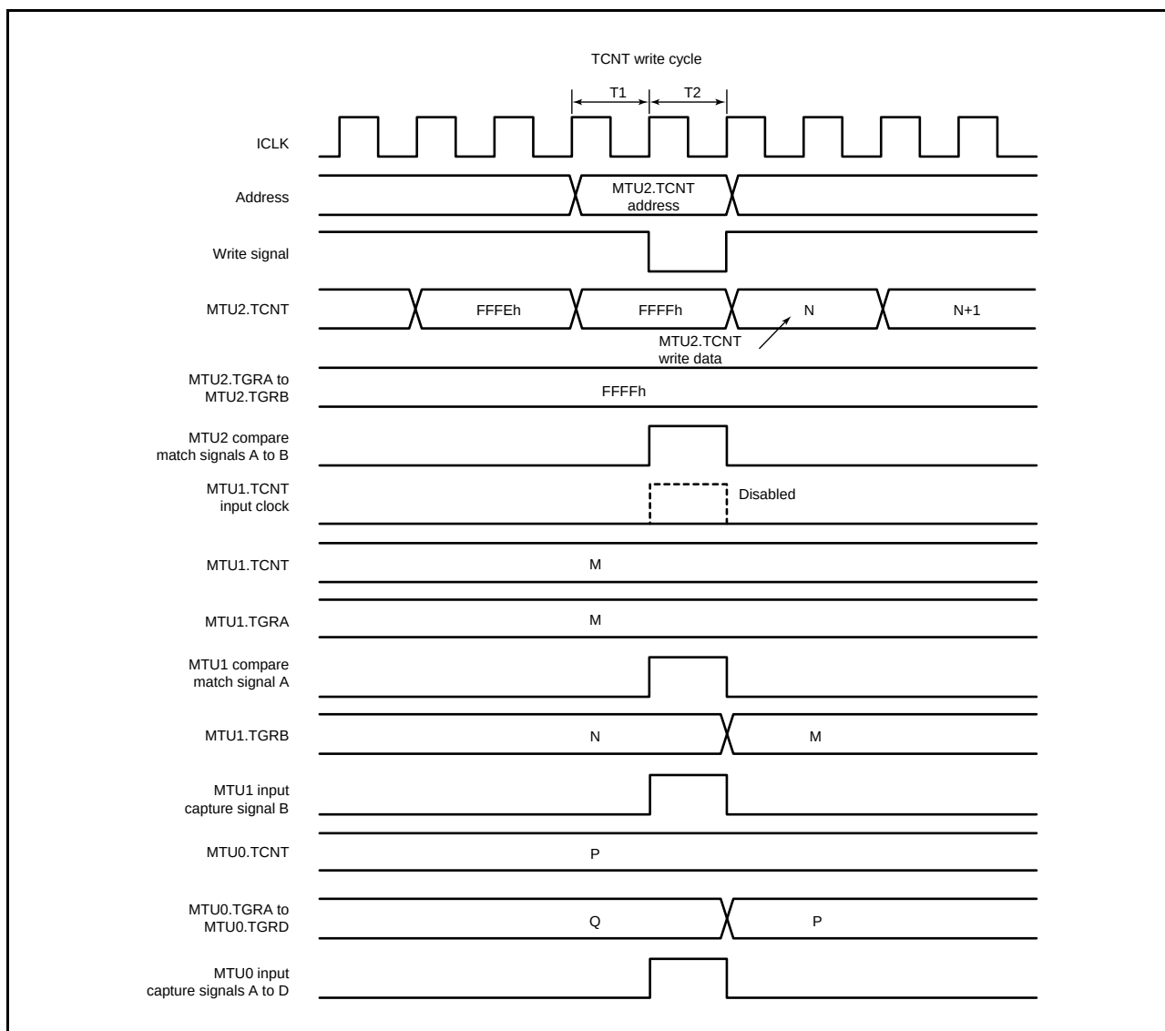
Figure 16.135 Contention between MTU2.TCNT Write Operation and Overflow/Underflow in Cascaded Operation
