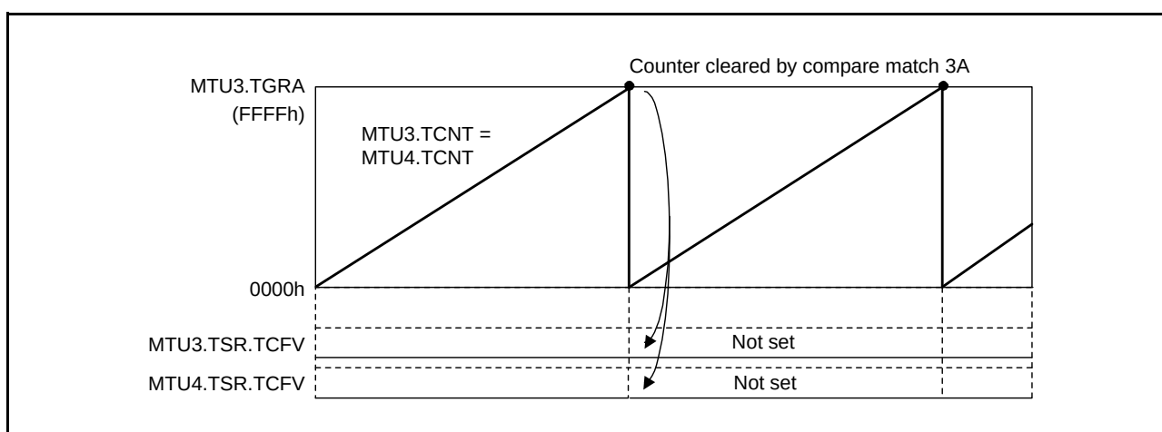
Figure 16.138 Overflow Flags in Reset-Synchronized PWM Mode
