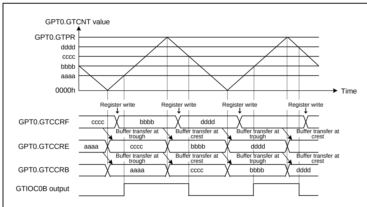
Figure 18.19 Example of GTCCRA and GTCCRB Double Buffer Operation (Output Compare, Triangle Waves, Buffer Operation at Both Troughs and Crests, Toggle Output at GTCCRB Compare Match, Output Retained at Cycle End)
