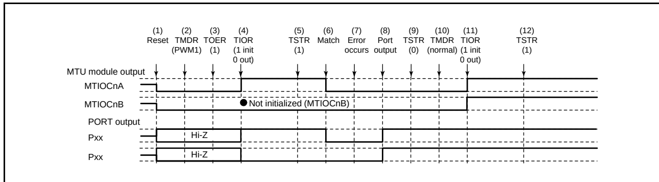
Figure 16.147 Error Occurrence in PWM Mode 1, Recovery in Normal Mode
