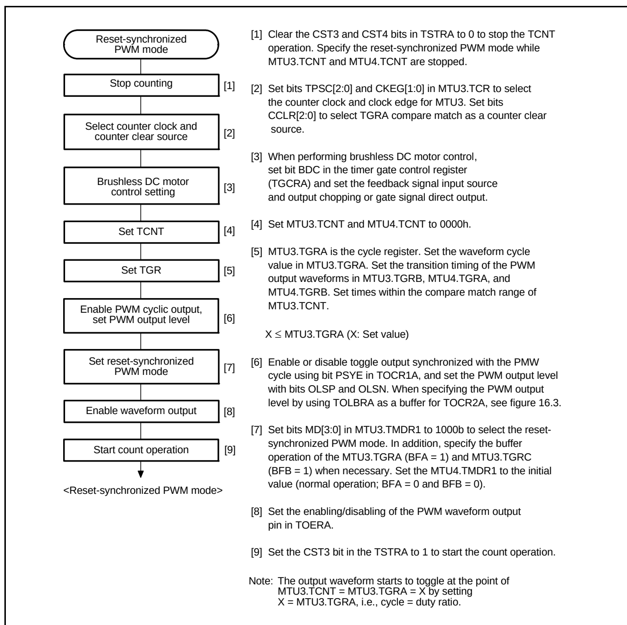
Figure 16.36 Procedure for Selecting Reset-Synchronized PWM Mode
