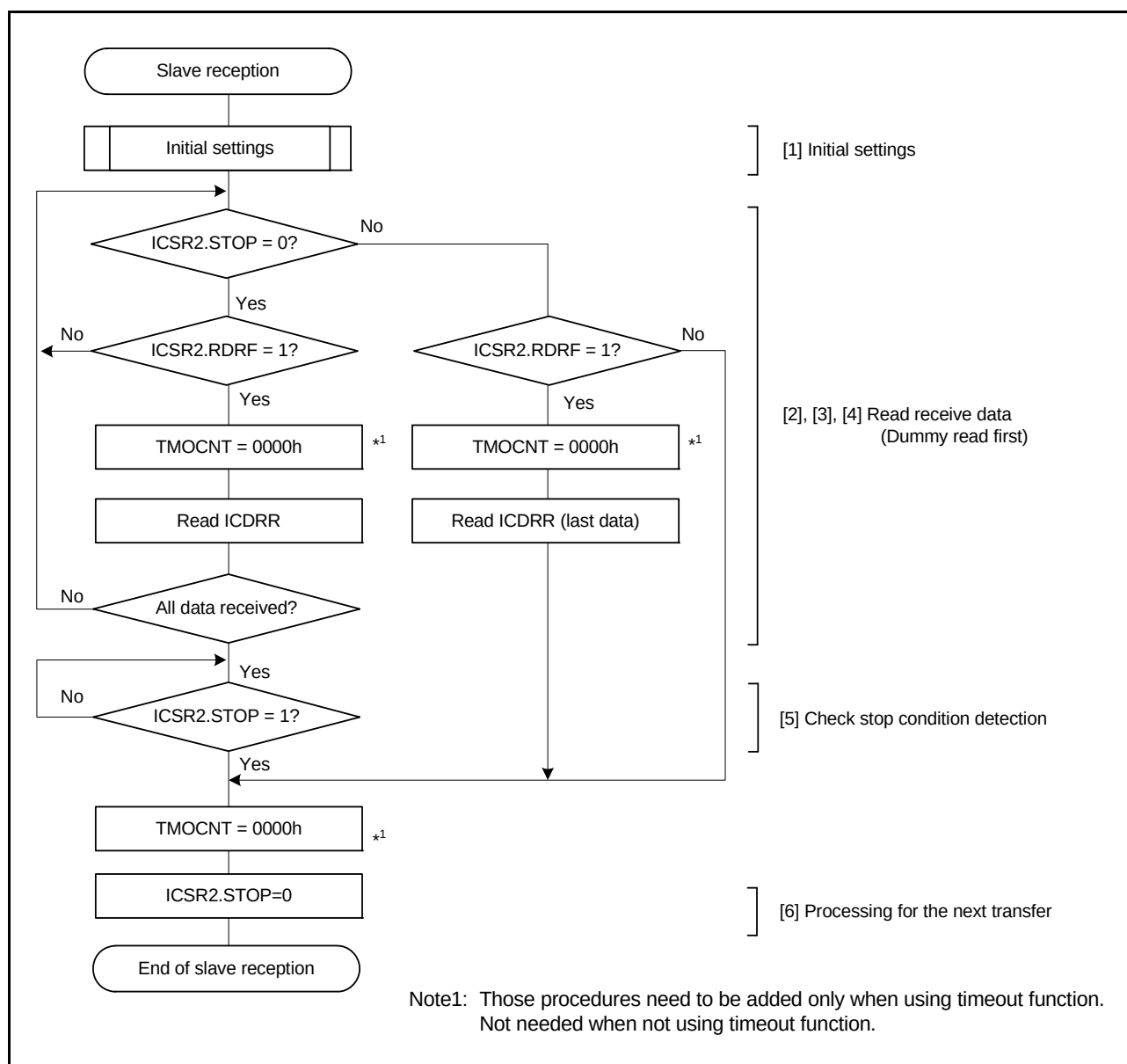
Figure 24.17 Example of Slave Reception Flowchart
