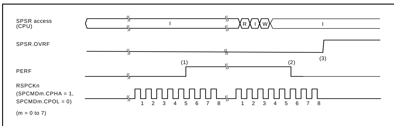
Figure 26.25 Operation Example of SPSR.PERF Flag
