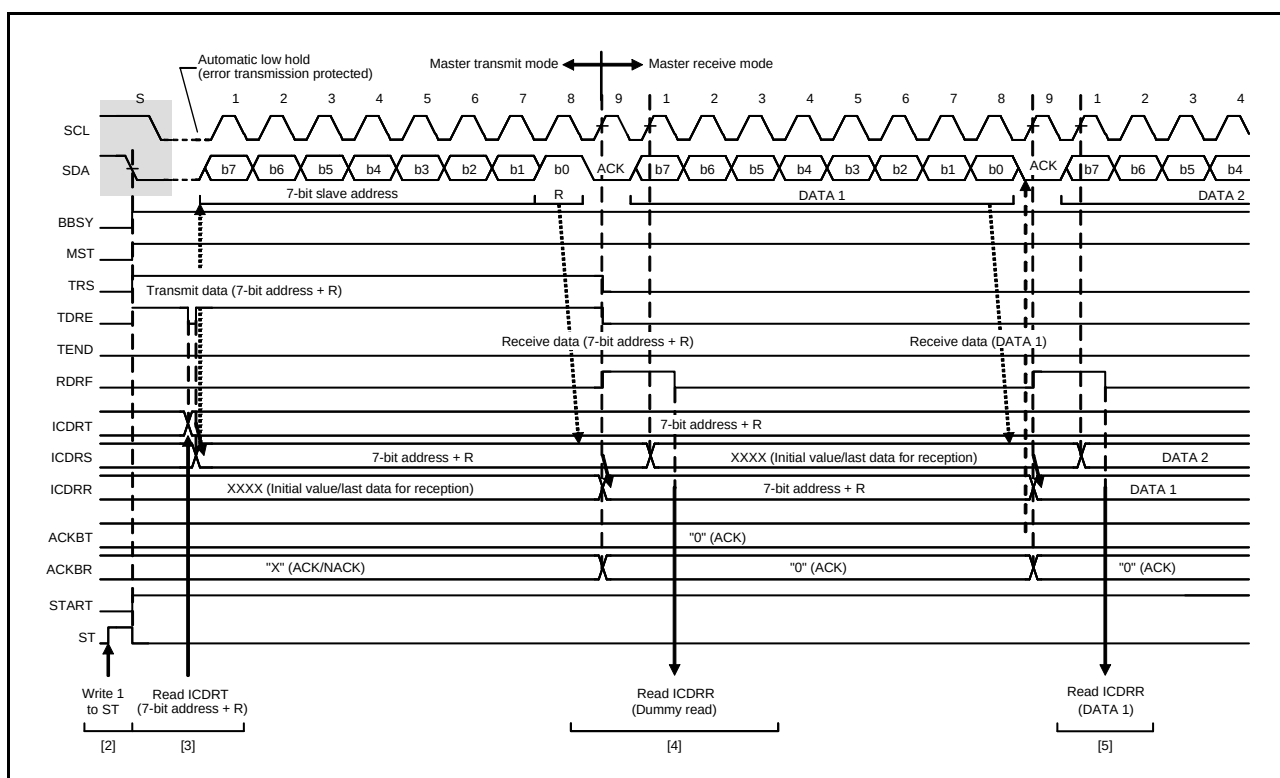
Figure 24.11 Master Receive Operation Timing (1) (7-Bit Address Format, when RDRFS=0)
