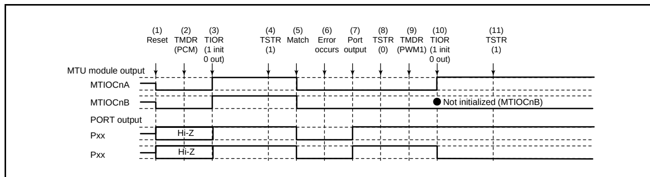
Figure 16.158 Error Occurrence in Phase Counting Mode, Recovery in PWM Mode 1
