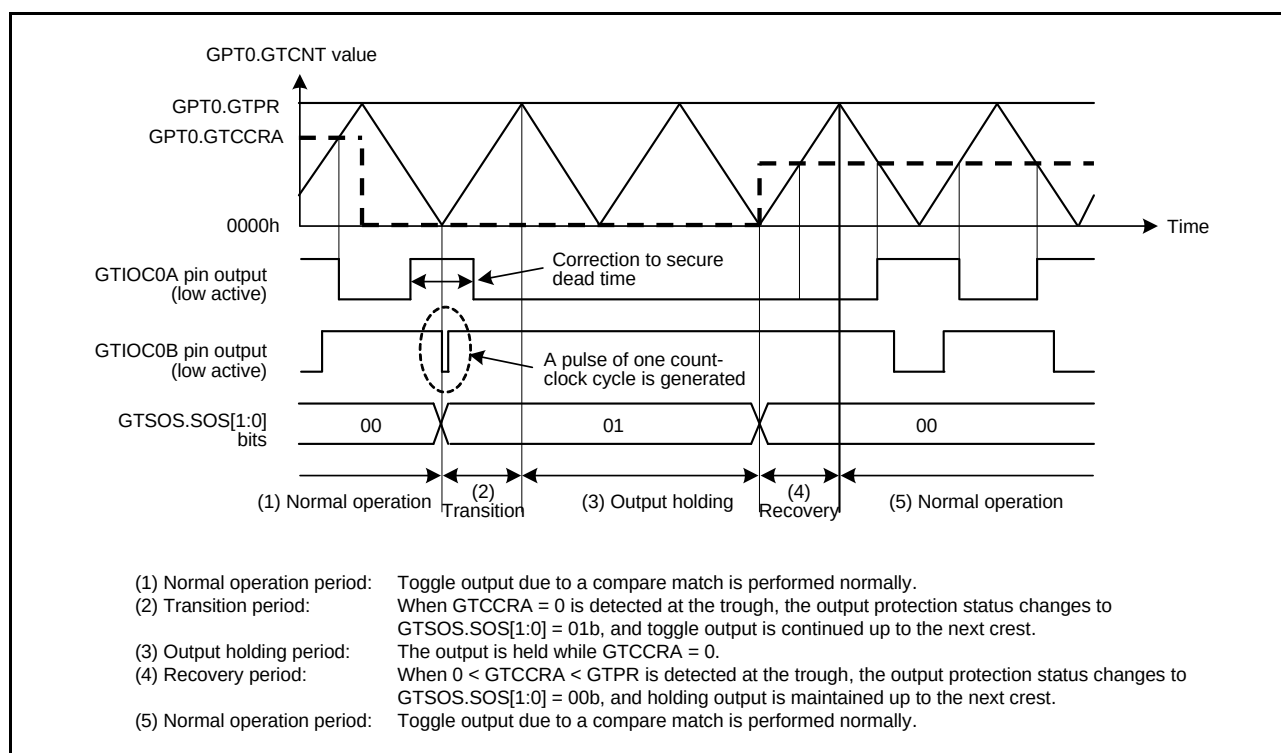
Figure 18.86 Example of Output Protection Function Operation When GTCCRA is Set to 0 during Buffer Transfer at Crests (Restored to 0 < GTCCRA < GTPR during Buffer Transfer at Troughs, Active Level: Low)
