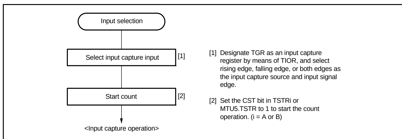
Figure 16.11 Example of Input Capture Operation Setting Procedure
