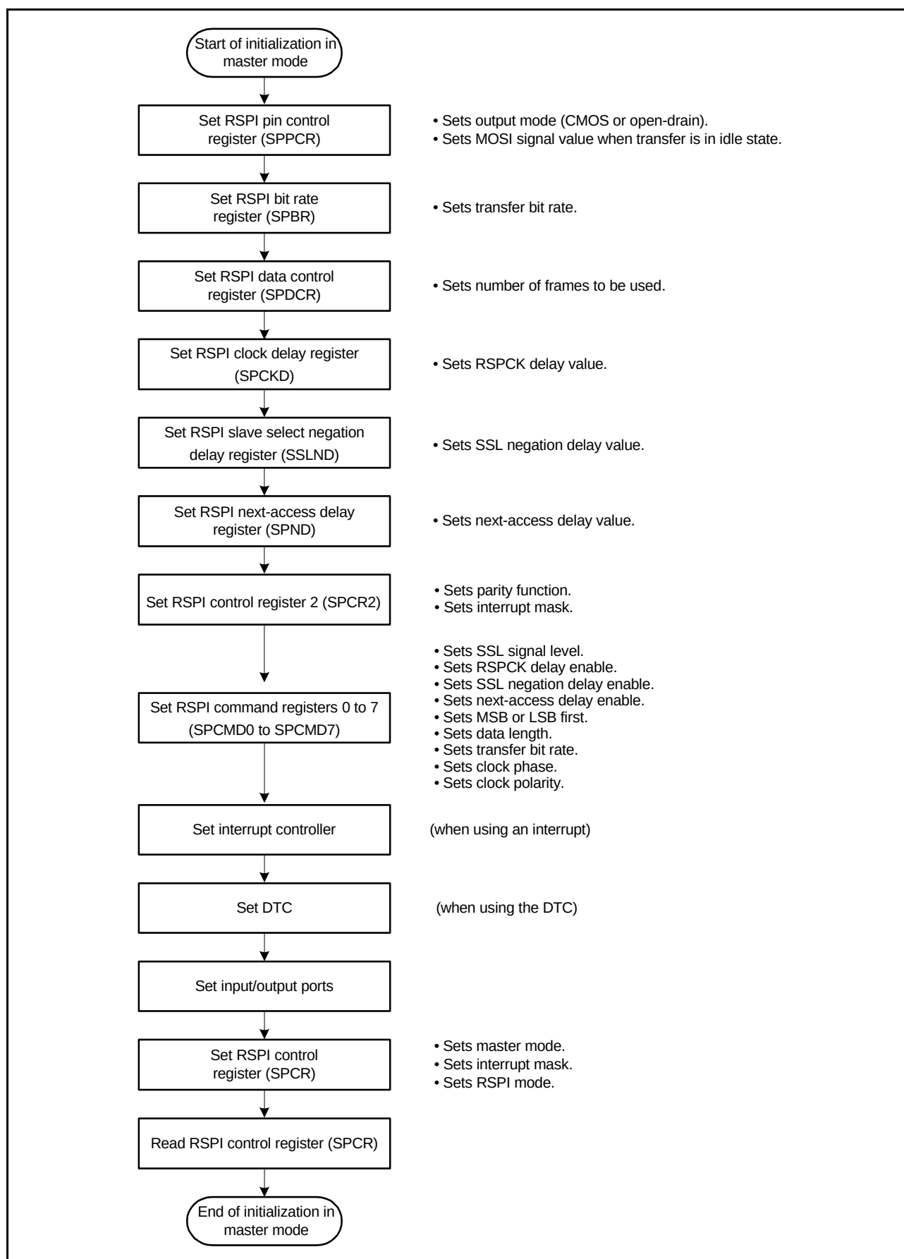
Figure 26.28 Example of Initialization Flowchart in Master Mode (SPI Operation)
