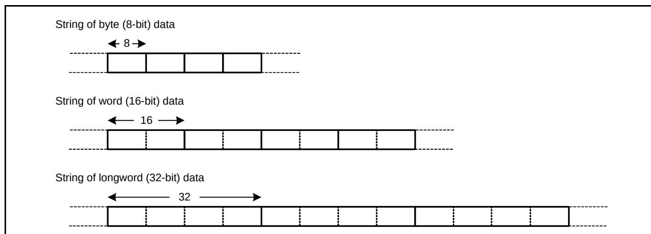
Figure 2.5 String
