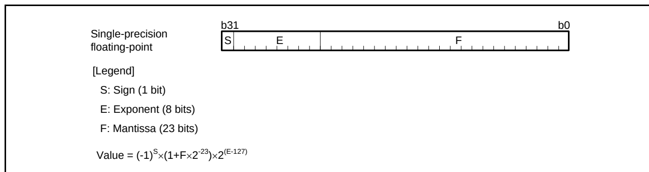
Figure 2.3 Floating-Point
