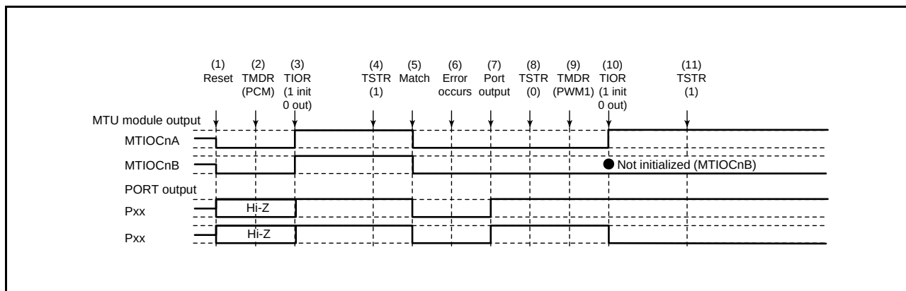
Figure 16.168 Error Occurrence in Reset-Synchronized PWM Mode, Recovery in Complementary PWM Mode
