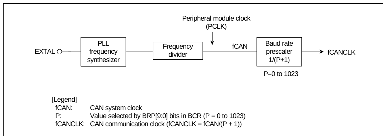
Figure 25.11 Block Diagram of CAN Clock Generator
