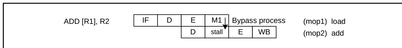
Figure 2.14 Arithmetic/Logic Instruction (Memory Source Operand)
