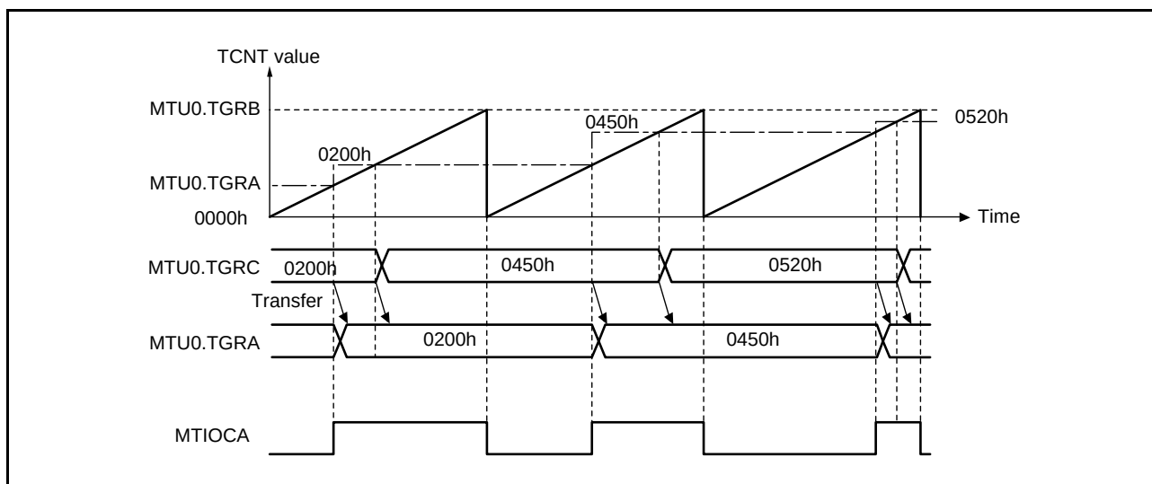
Figure 16.18 Example of Buffer Operation (1)
