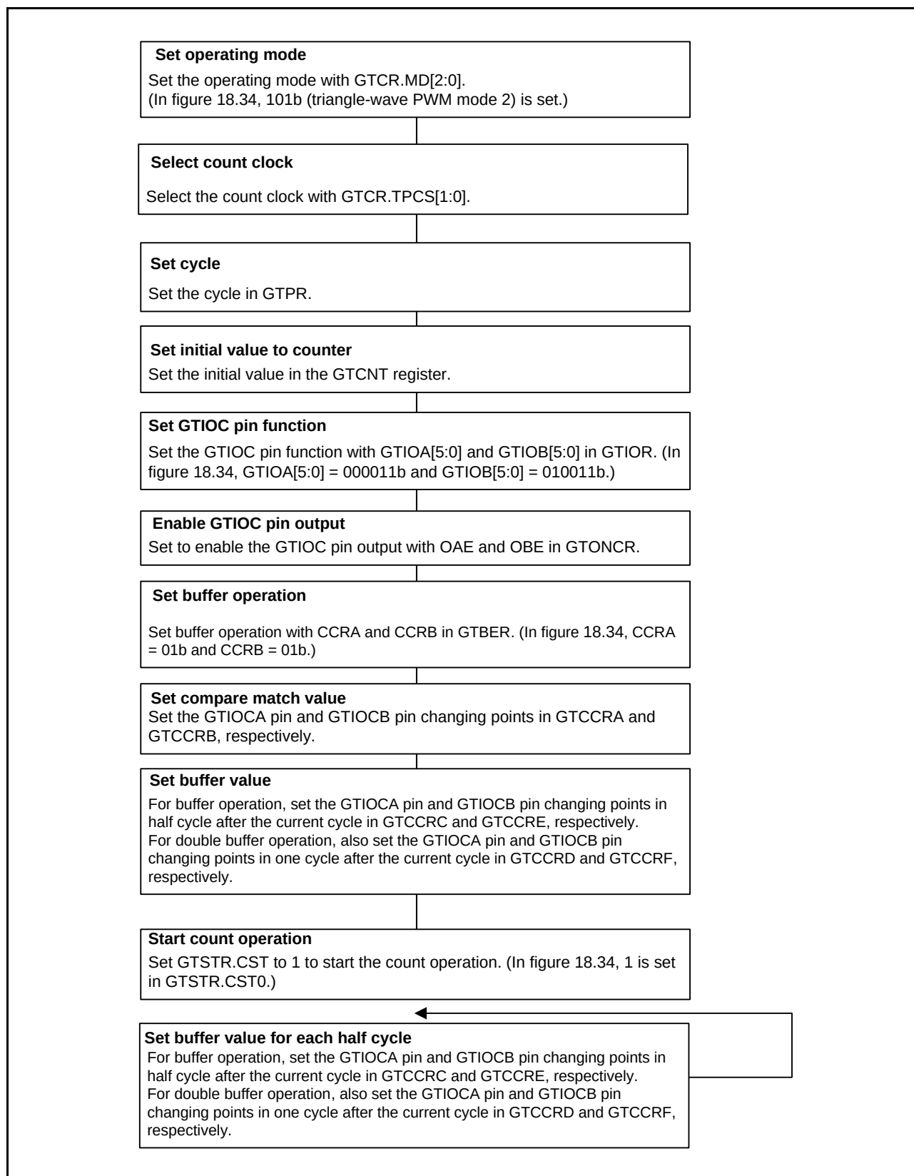
Figure 18.35 Example for Setting Triangle-Wave PWM Mode 2
