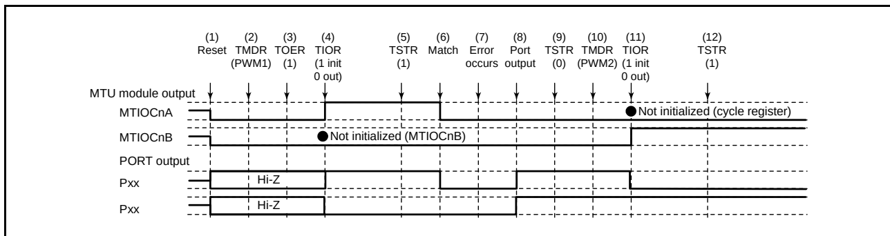
Figure 16.149 Error Occurrence in PWM Mode 1, Recovery in PWM Mode 2
