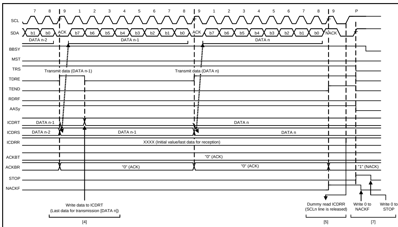
Figure 24.16 Slave Transmit Operation Timing (2)
