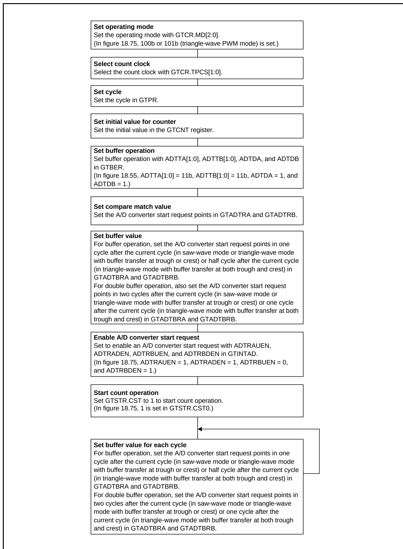
Figure 18.76 Example for Setting A/D Converter Start Request Timing Operation
