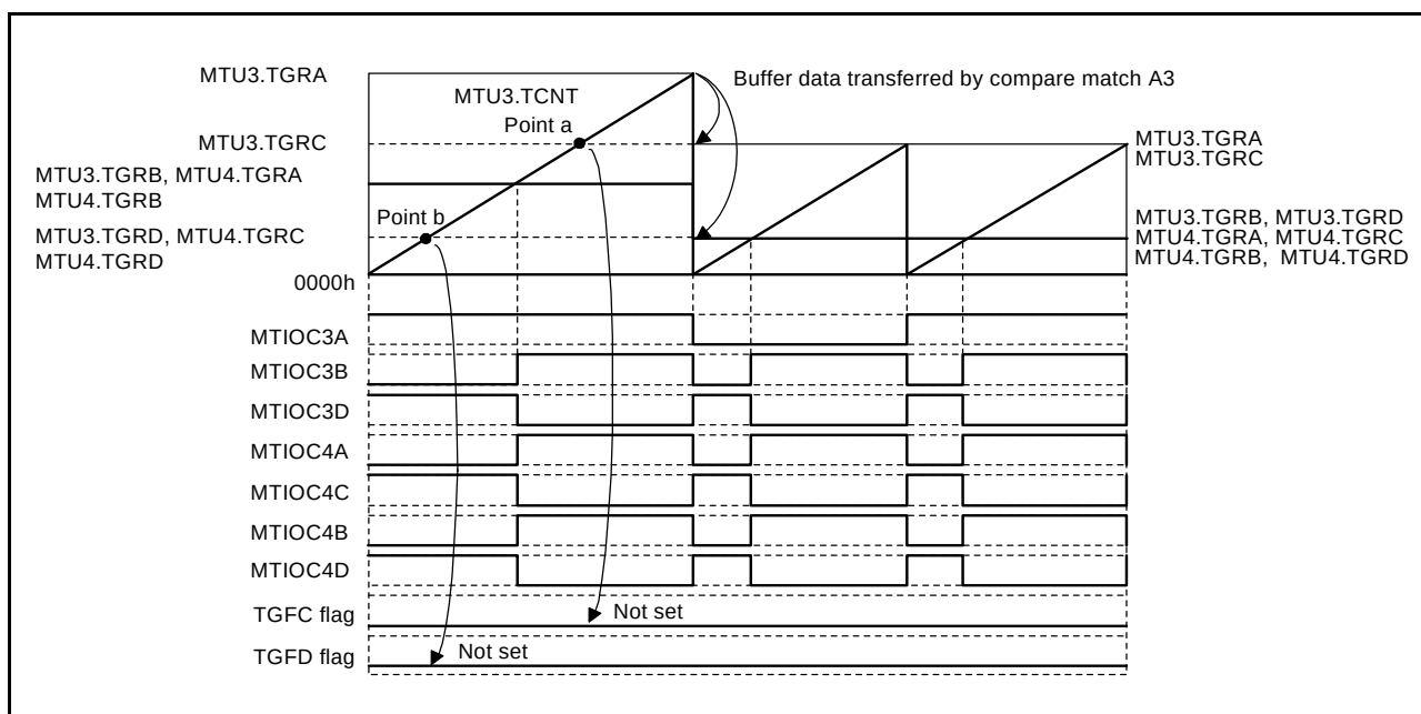
Figure 16.137 Buffer Operation and Compare Match Flags in Reset-Synchronized PWM Mode
