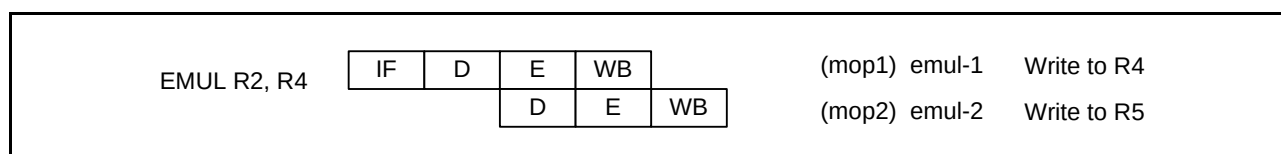
Figure 2.16 EMUL, EMULU Instructions (Register- Register, Register-Immediate)
