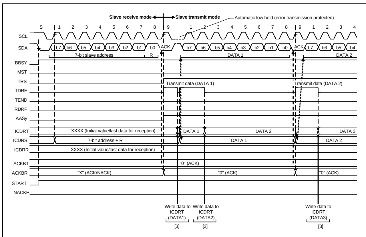
Figure 24.15 Slave Transmit Operation Timing (1) (7-Bit Address Format)
