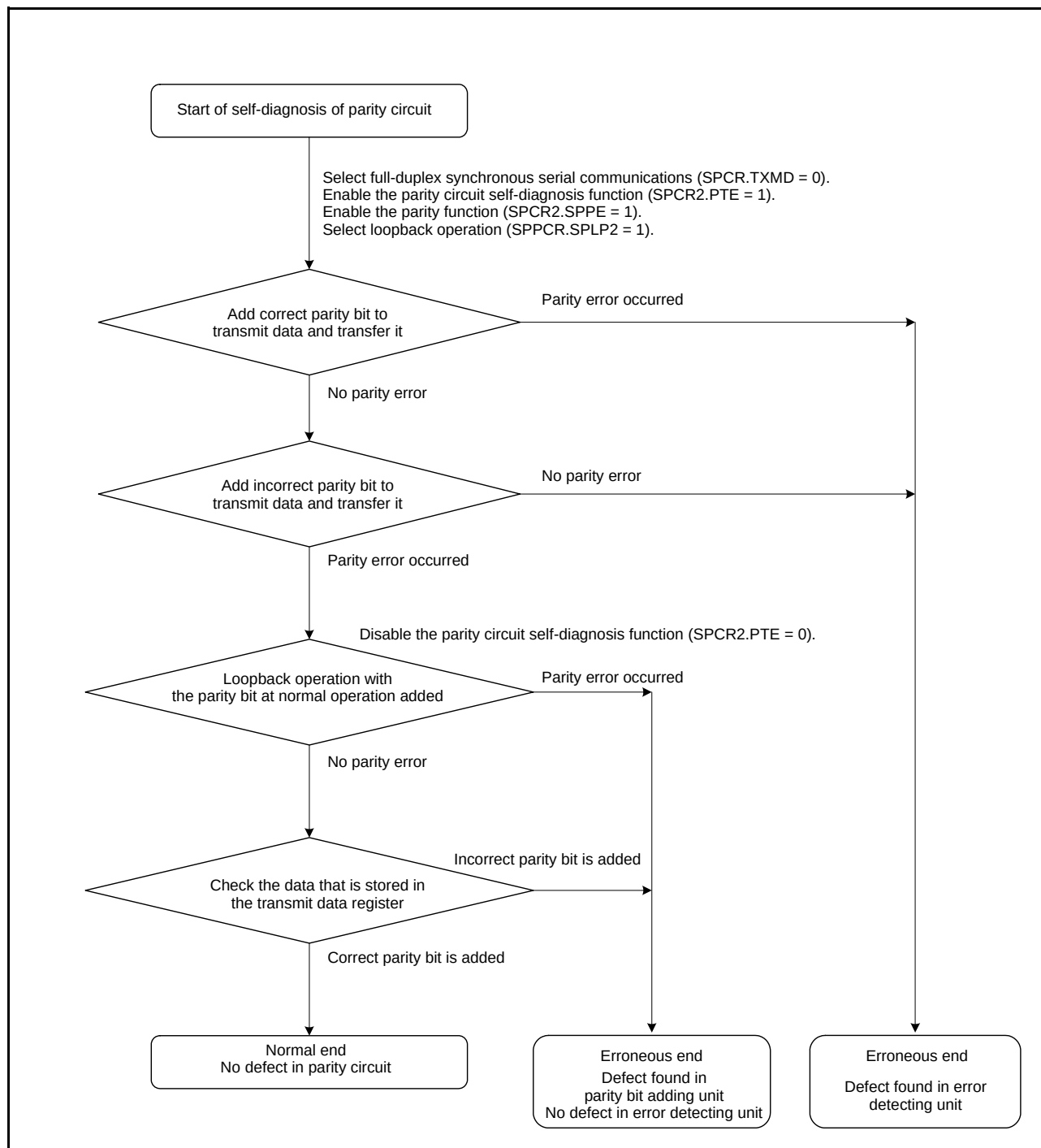
Figure 26.42 Flowchart for Self-Diagnosis of Parity Circuit
