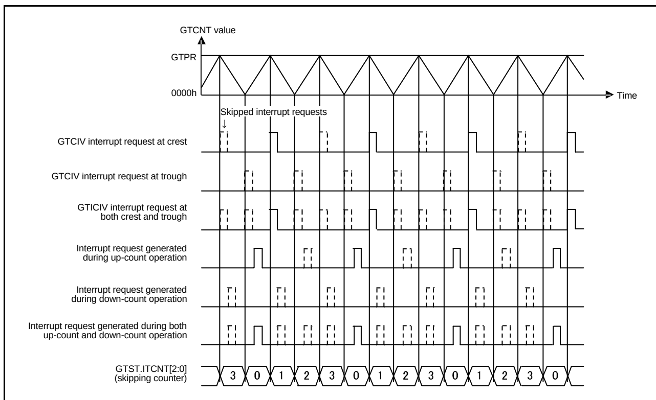
Figure 18.73 Example of Interrupt Skipping Function Operation (Triangle Waves, Counting and Skipping Both Troughs and Crests, Skipping Count: 3, Skipping Started at Down-Counting)
