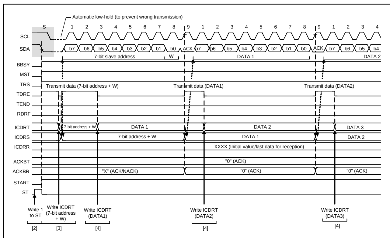
Figure 24.7 Master Transmit Operation Timing (1) (7-Bit Address Format)
