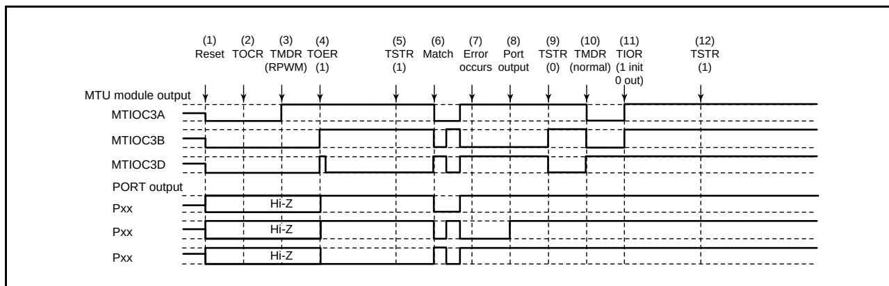
Figure 16.166 Error Occurrence in Reset-Synchronized PWM Mode, Recovery in Normal Mode
