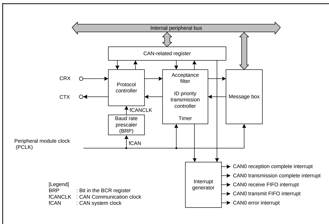
Figure 25.1 Block Diagram of CAN Module
