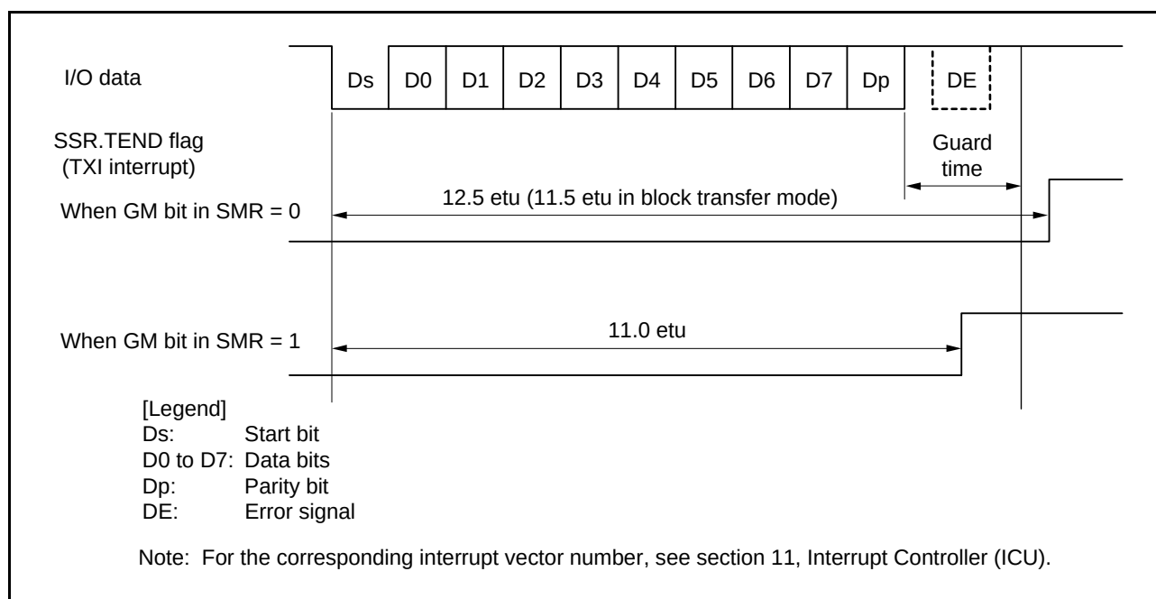
Figure 22.29 SSR.TEND Flag Generation Timing during Transmission
