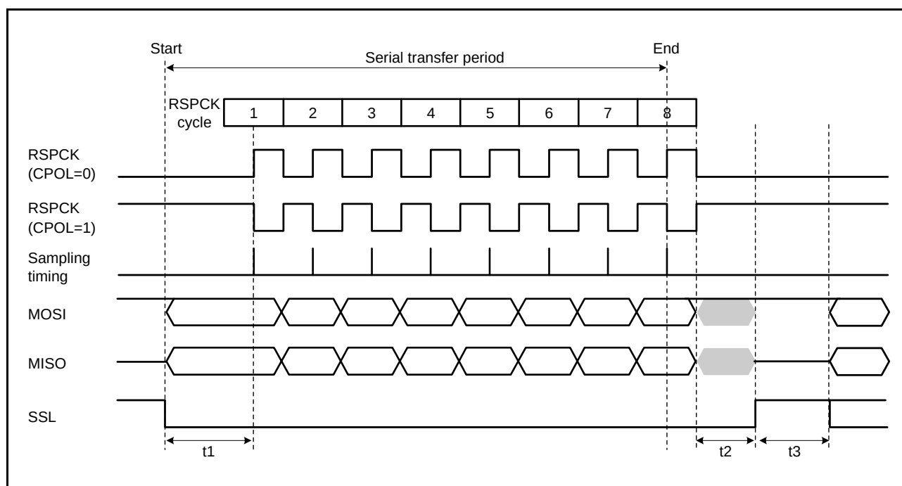
Figure 26.11 RSPI Transfer Format (CPHA = 0)
