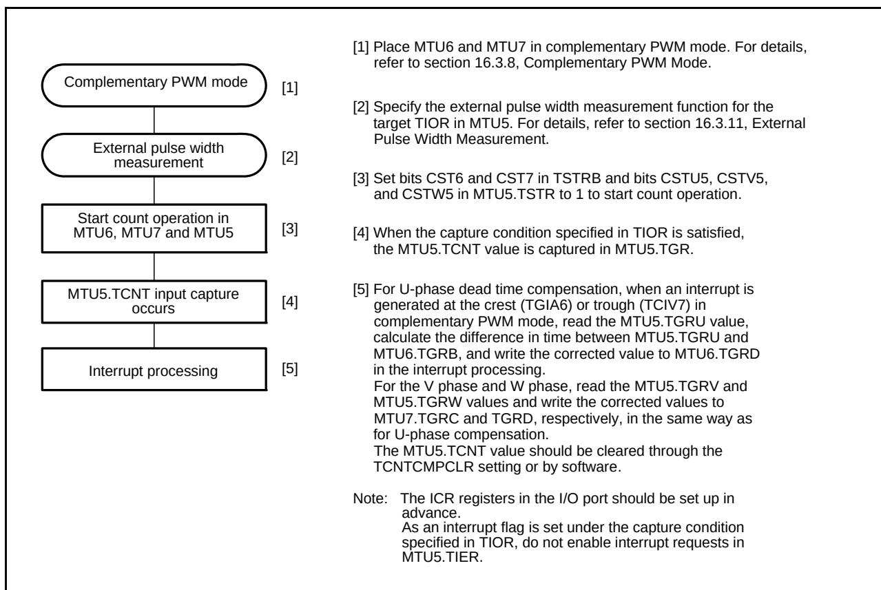
Figure 16.98 Example of Dead Time Compensation Setting Procedure
