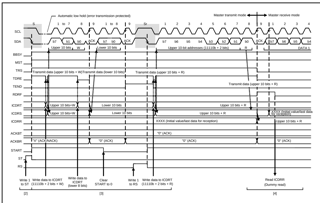
Figure 24.12 Master Receive Operation Timing (2) (10-Bit Address Format, when RDRFS=0)
