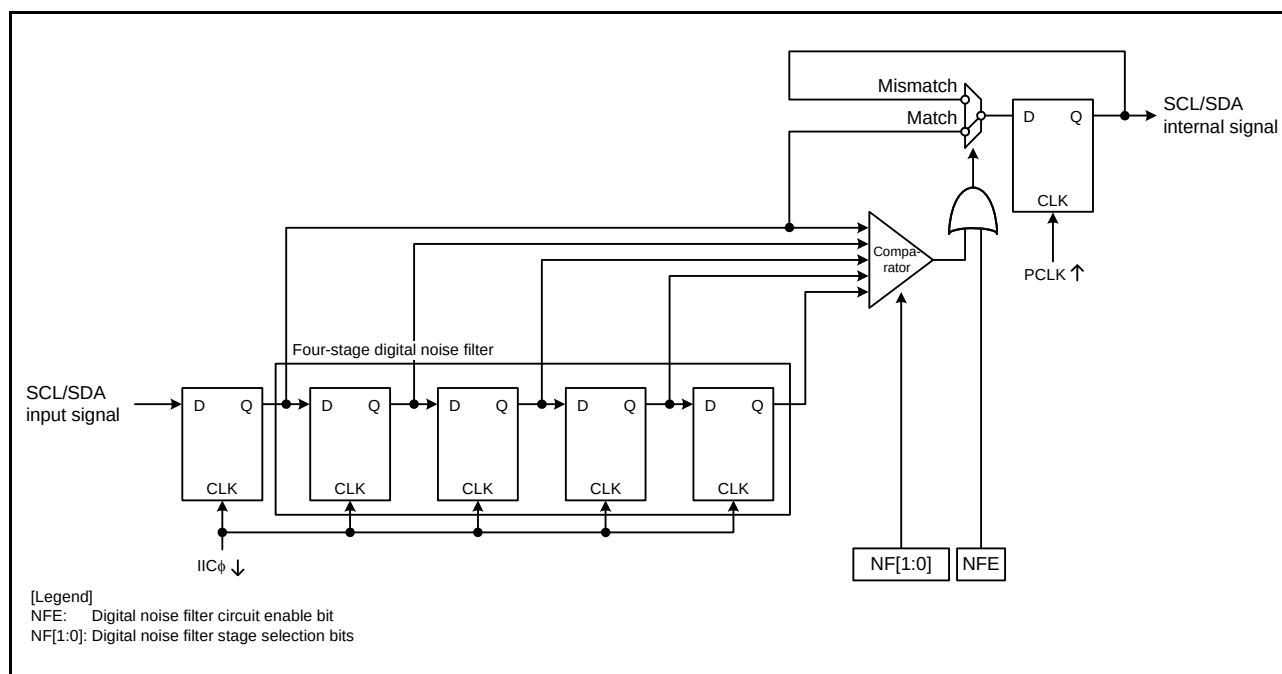
Figure 24.22 Block Diagram of Digital Noise Filter Circuit
