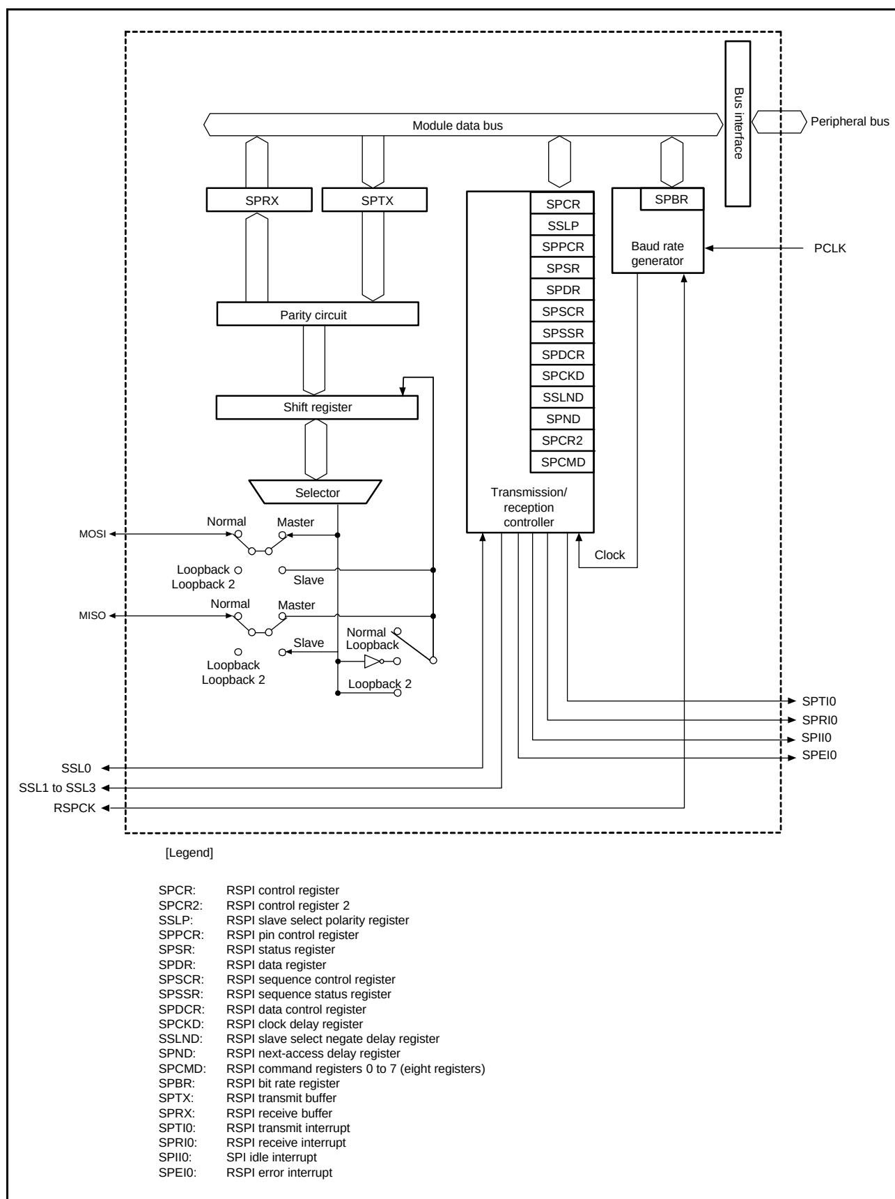
Figure 26.1 Block Diagram of RSPI
