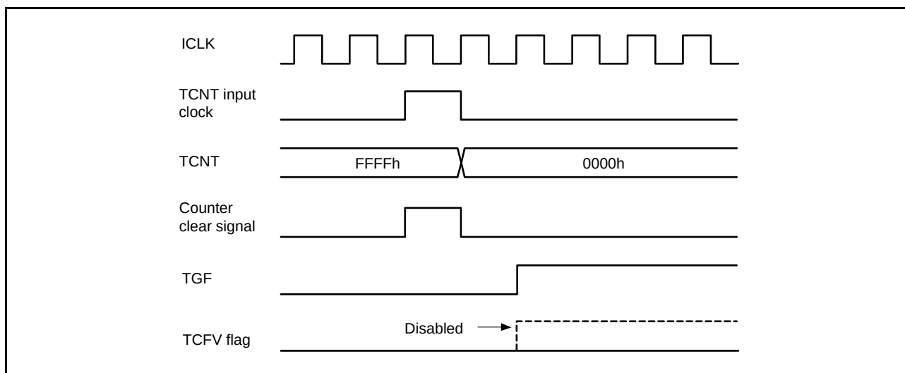
Figure 16.139 Contention between Overflow and Counter Clearing
