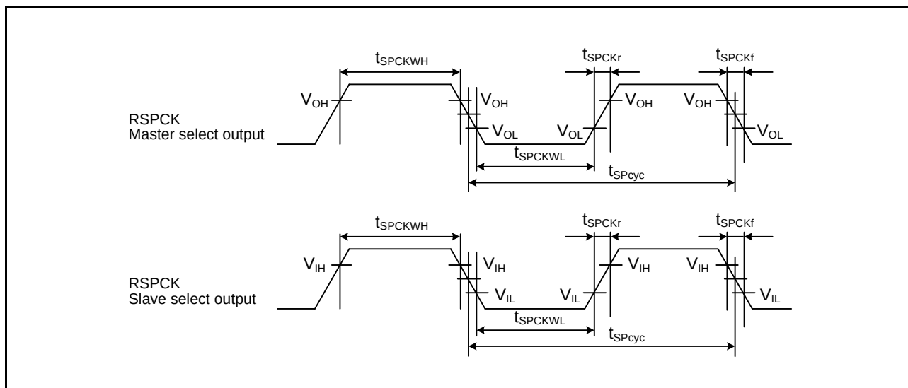
Figure 33.11 RSPI Clock Timing
