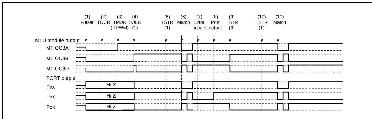
Figure 16.169 Error Occurrence in Reset-Synchronized PWM Mode, Recovery in Reset-Synchronized PWM Mode
