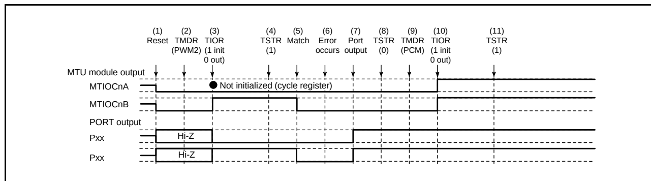
Figure 16.156 Error Occurrence in PWM Mode 2, Recovery in Phase Counting Mode
