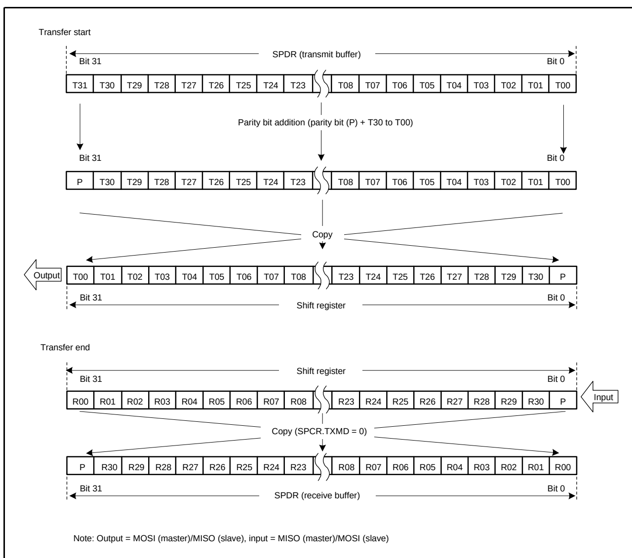
Figure 26.18 LSB First Transfer (2) (32-Bit Data, Parity Function Enabled)
