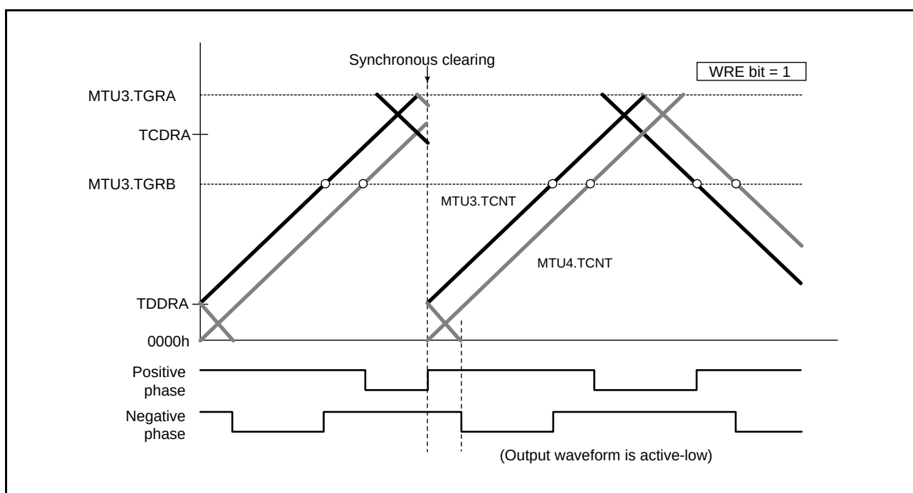
Figure 16.60 Example of Synchronous Clearing in Interval Tb at Crest (Timing (6) in Figure 16.57; Bit WRE of TWCR or TWCRB is 1)
