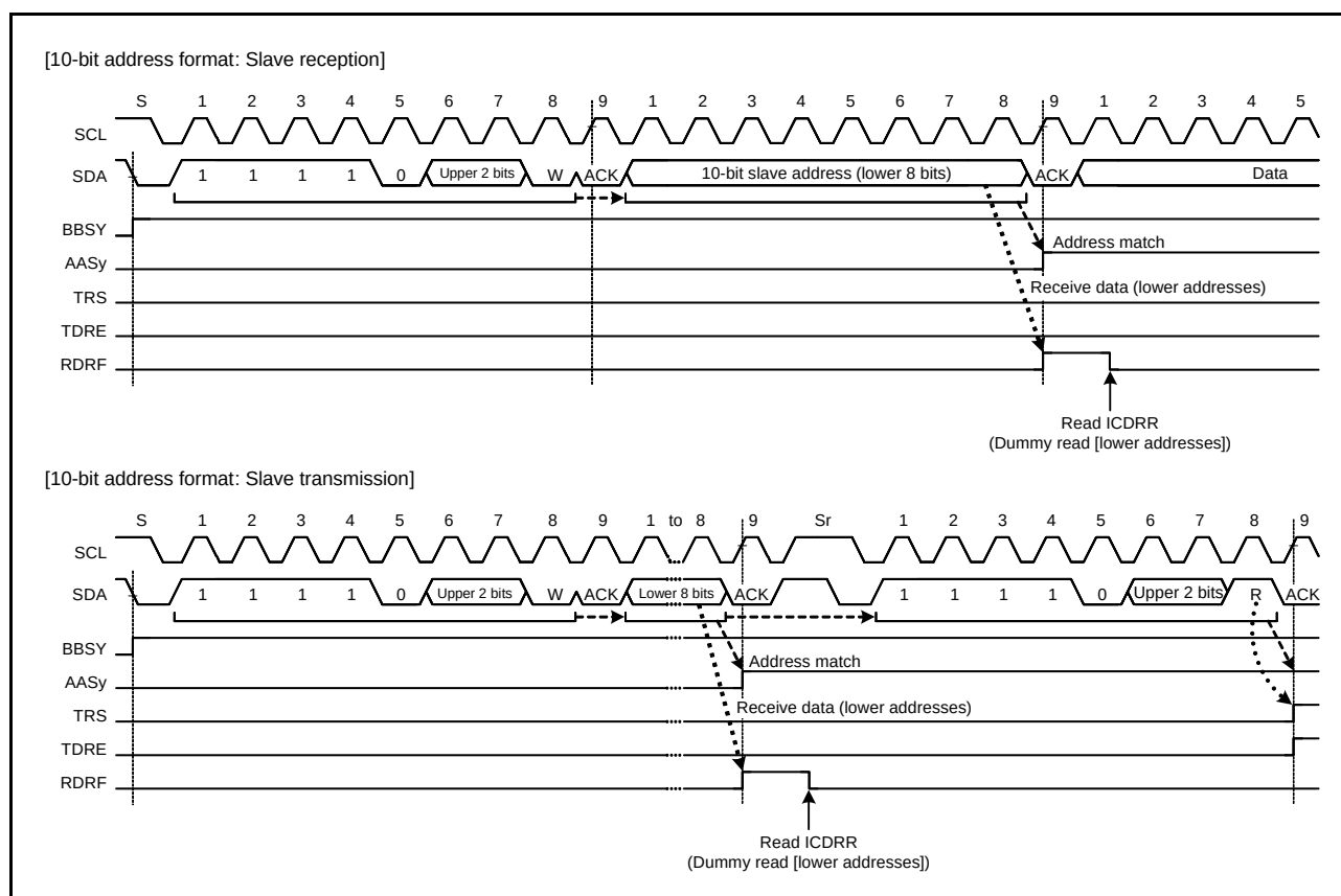
Figure 24.24 AASy Flag Set Timing with 10-Bit Address Format Selected
