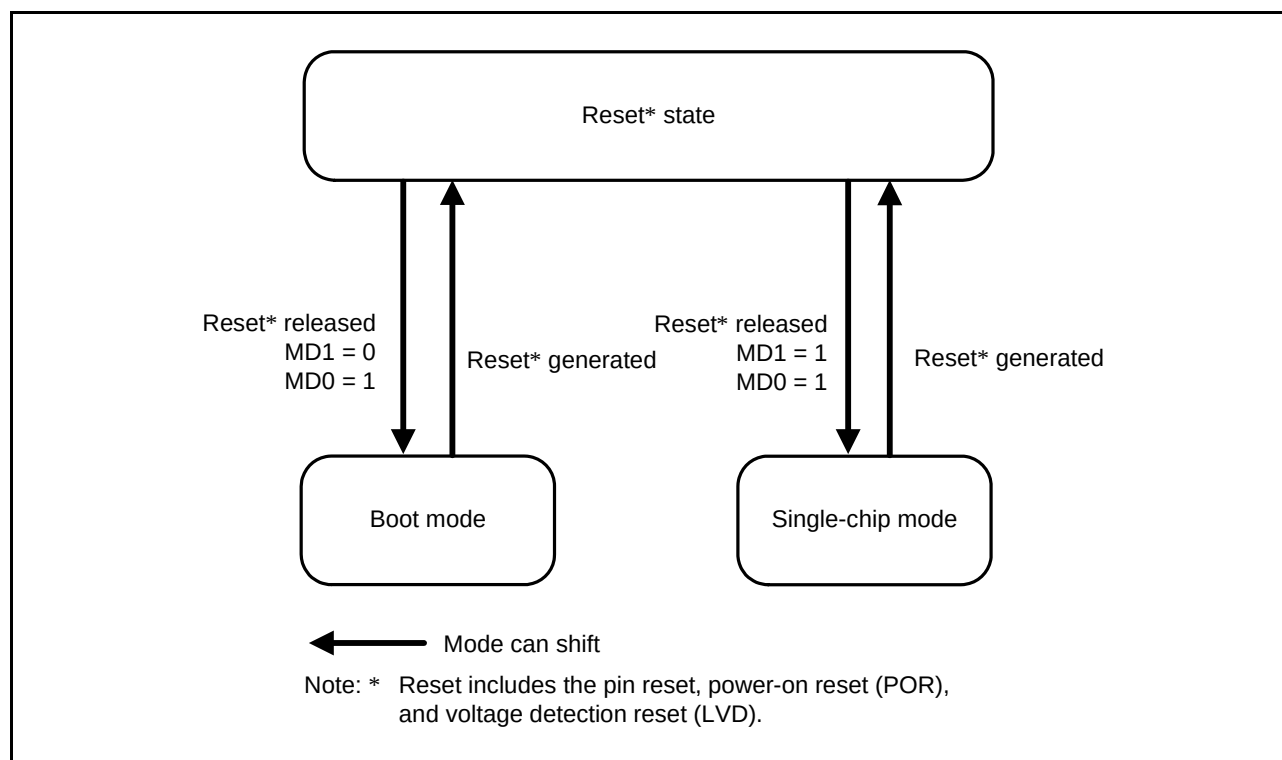
Figure 3.1 Setting of Pins MD1 and MD0 and Operating Modes
