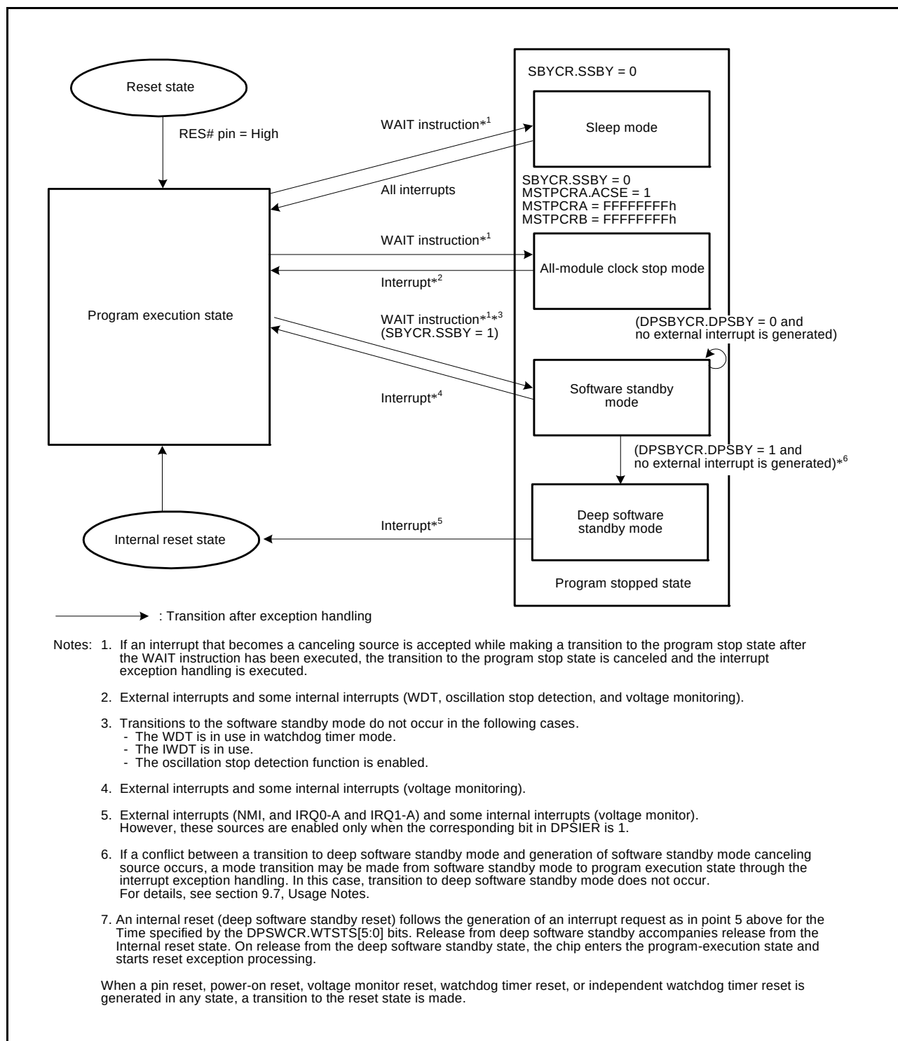
Figure 9.1 Mode Transitions
