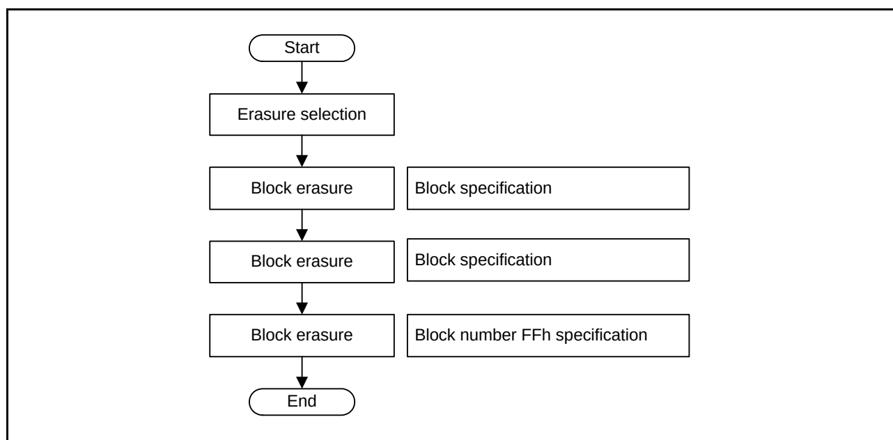
Figure 31.32 Procedure for ROM Erasure in Boot Mode
