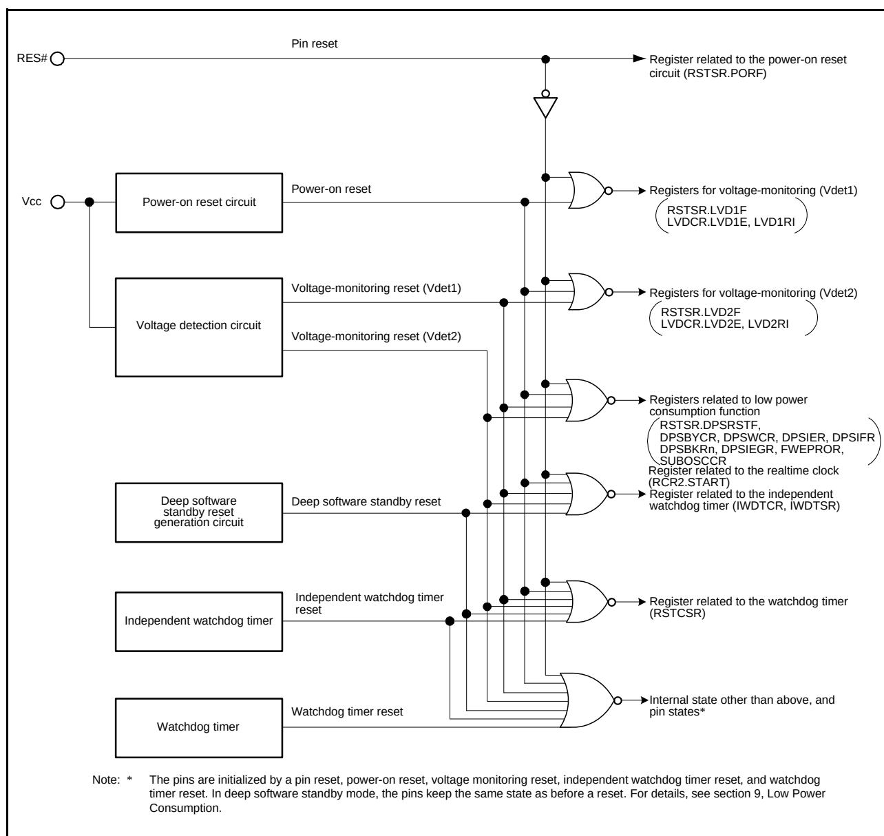
Figure 6.1 Block Diagram of Reset Circuit
