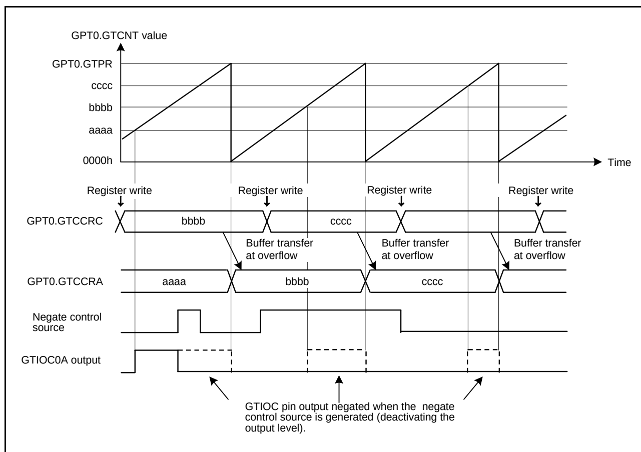
Figure 18.82 Example of GTIOC Pin Output Negate Control Operation (Saw-Wave Up-Counting, Buffer Operation, Active Level: 1, High Output at GTCCRA Compare Match, Low Output at Cycle End)
