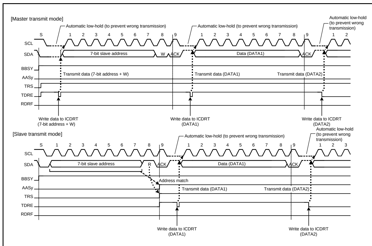
Figure 24.29 Automatic Low-Hold Operation in Transmit Mode
