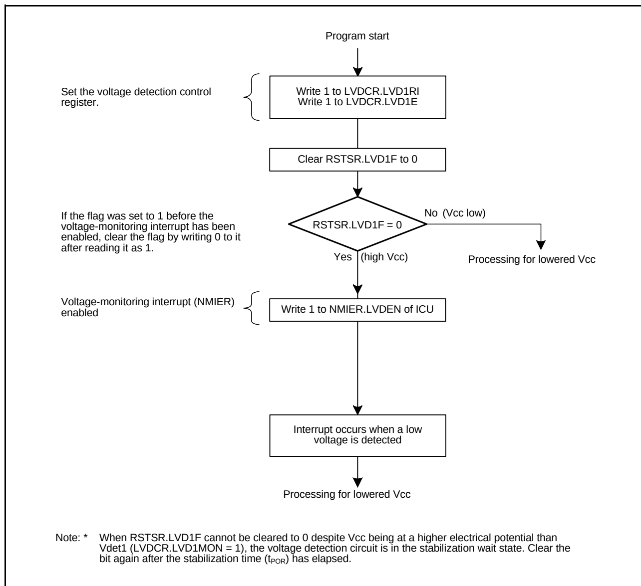
Figure 7.5 Example of Procedure for Setting Voltage-Monitoring Interrupt
