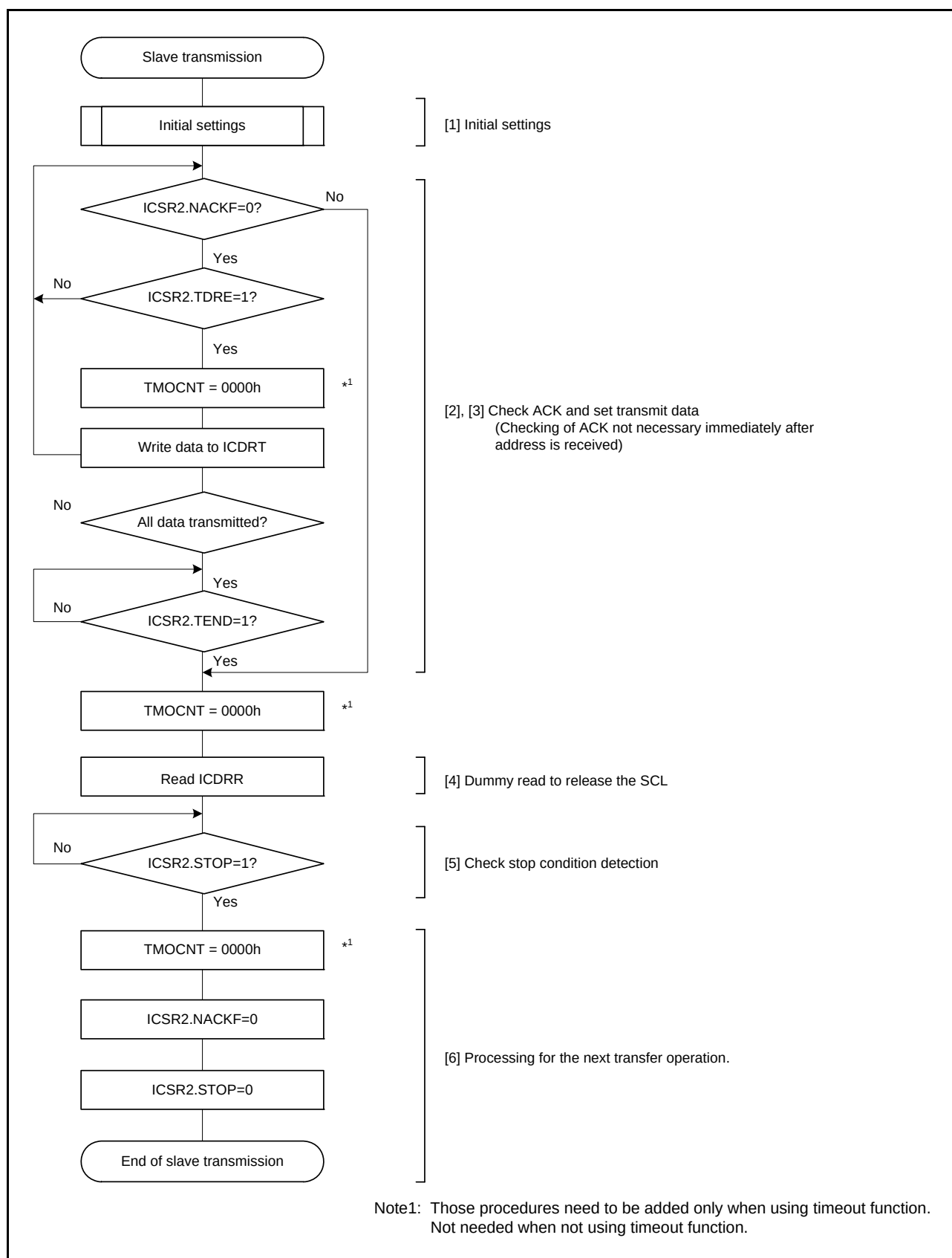
Figure 24.14 Example of Slave Transmission Flowchart
