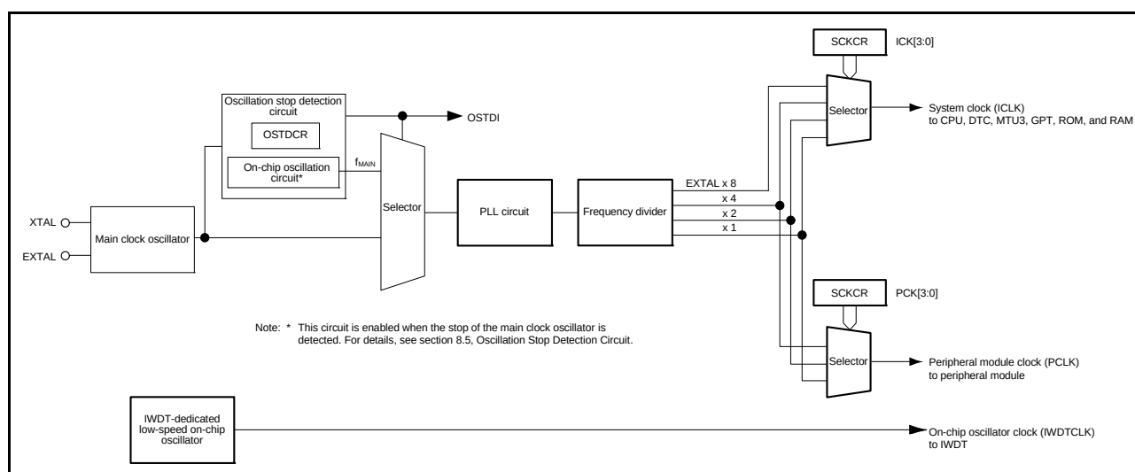
Figure 8.1 Block Diagram of Clock Generation Circuit
