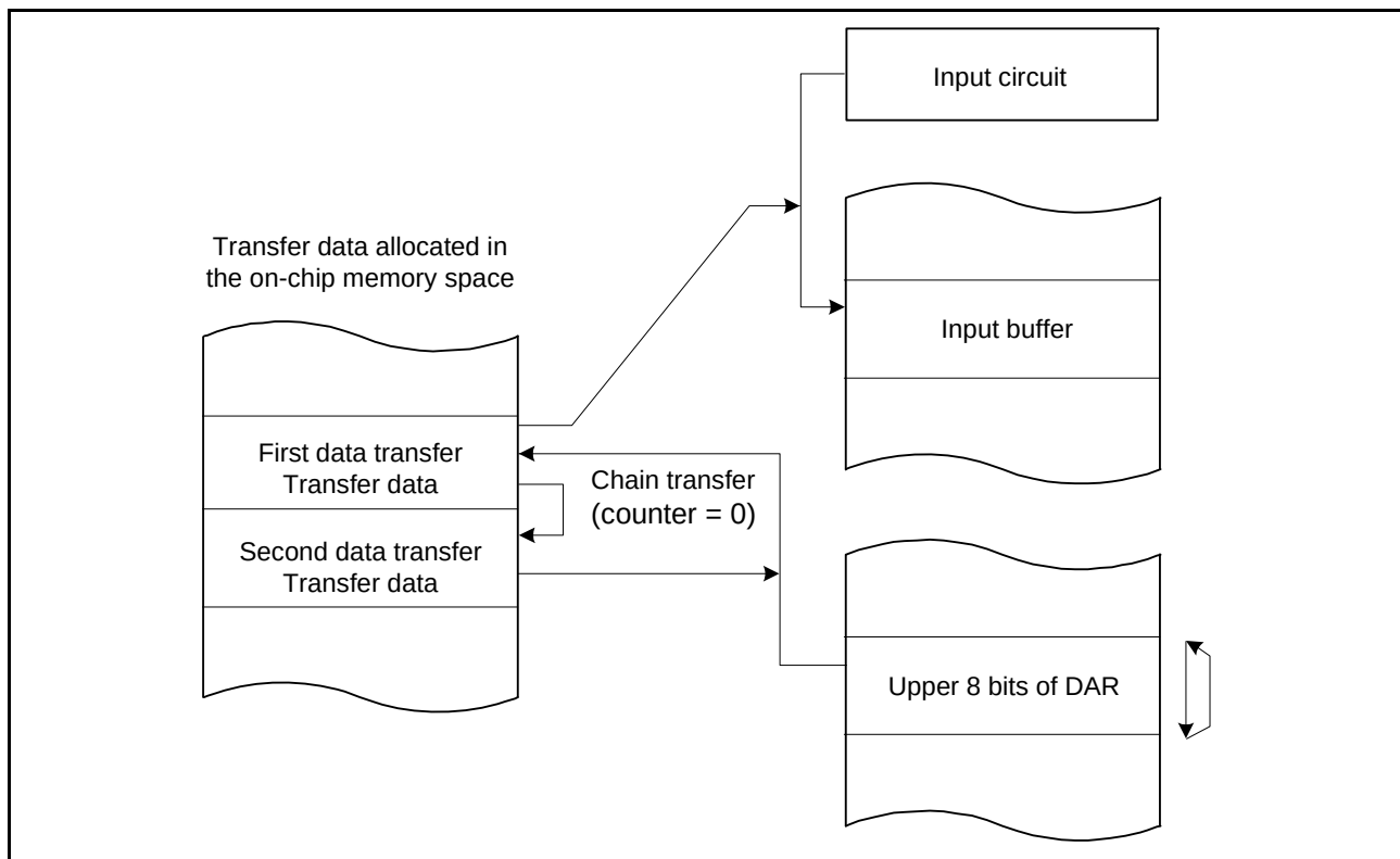
Figure 14.15 Chain Transfer when Counter = 0
