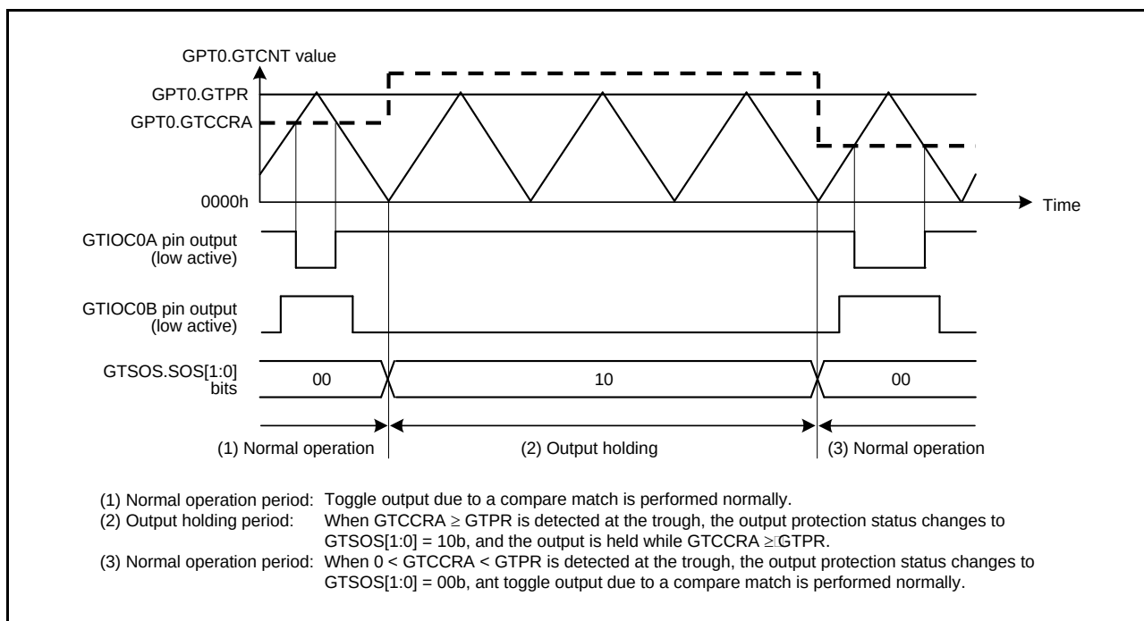
Figure 18.88 Example of Output Protection Function Operation When GTCCRA \geq GTPR is set during Buffer Transfer at Troughs (Restored to 0 < GTCCRA < GTPR during Buffer Transfer at Troughs, Active Level: Low)
