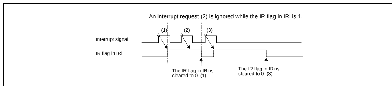
Figure 11.3 Timing for Re-setting of the IRI. IR Flag
