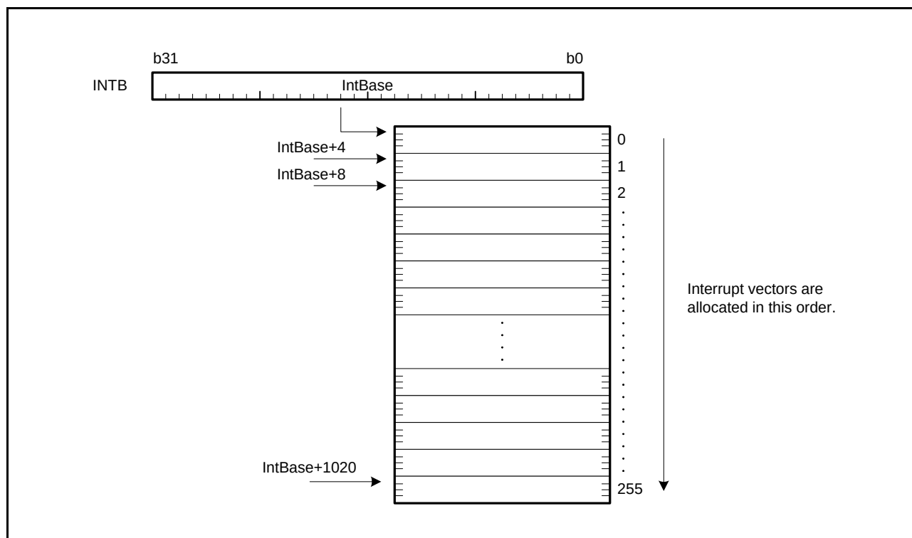
Figure 2.9 Relocatable Vector Table
