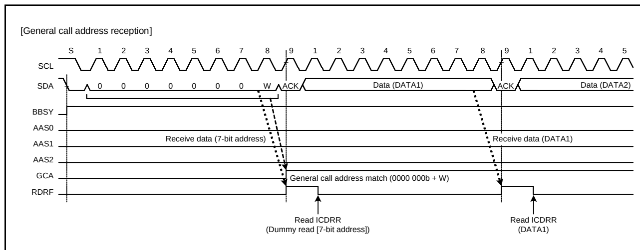
Figure 24.26 Timing of GCA Flag Setting during Reception of General Call Address
