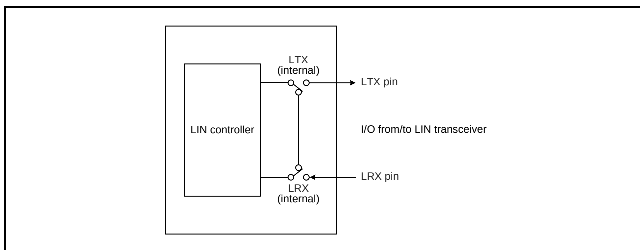
Figure 27.16 LIN Self-Test Mode Connection
