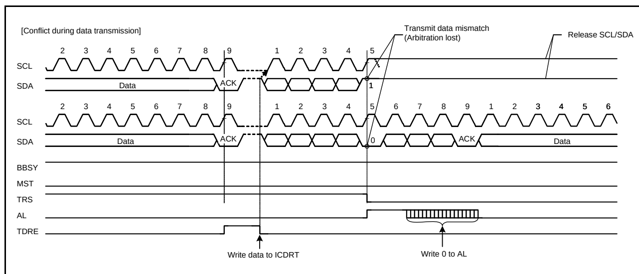
Figure 24.35 Example of Slave Arbitration Lost Detection (SALE = 1)
