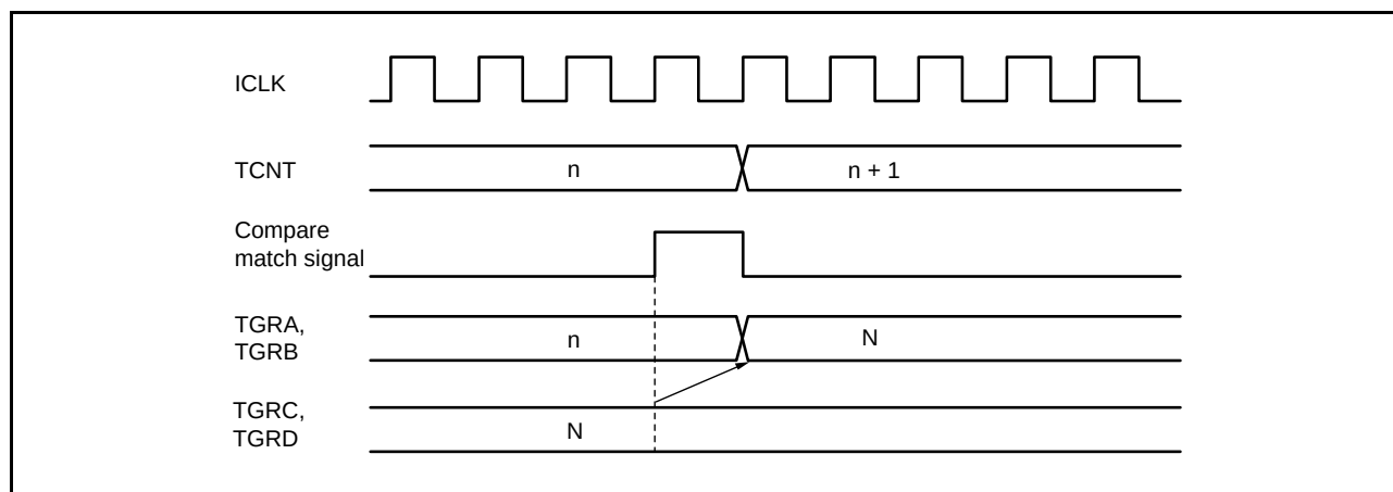
Figure 16.111 Buffer Operation Timing (Compare Match)
