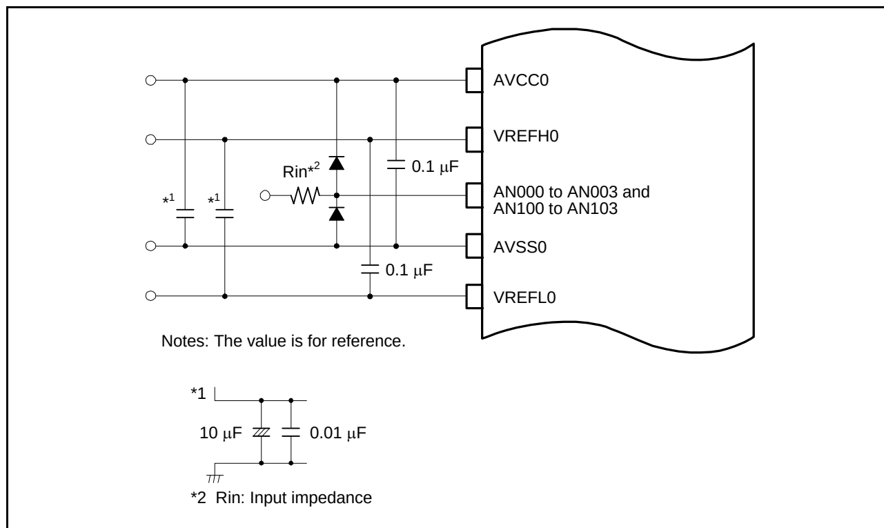
Figure 28.12 Example of a Protective Circuit for Analog Inputs
