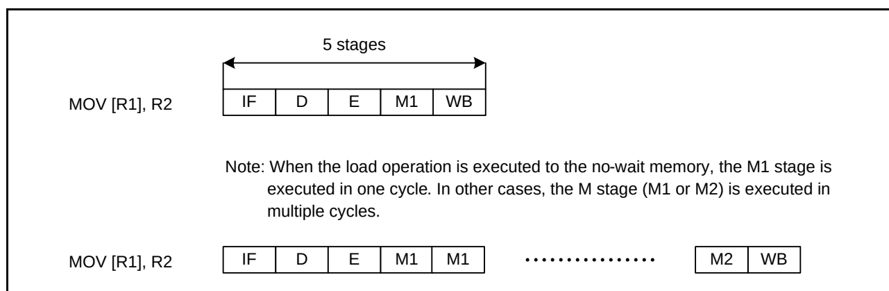
Figure 2.12 Load Operation
