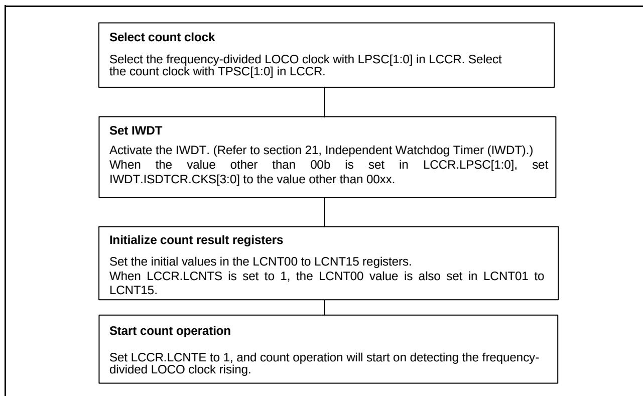
Figure 18.78 Example for Setting LOCO Count Function Operation
