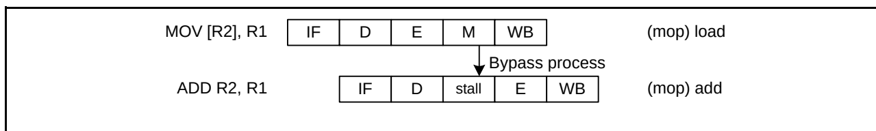
Figure 2.23 When the Subsequent Instruction Uses an Operand Read from the Memory
