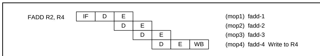
Figure 2.19 Floating-Point Operation Instruction (Register-Register, Immediate-Register)
