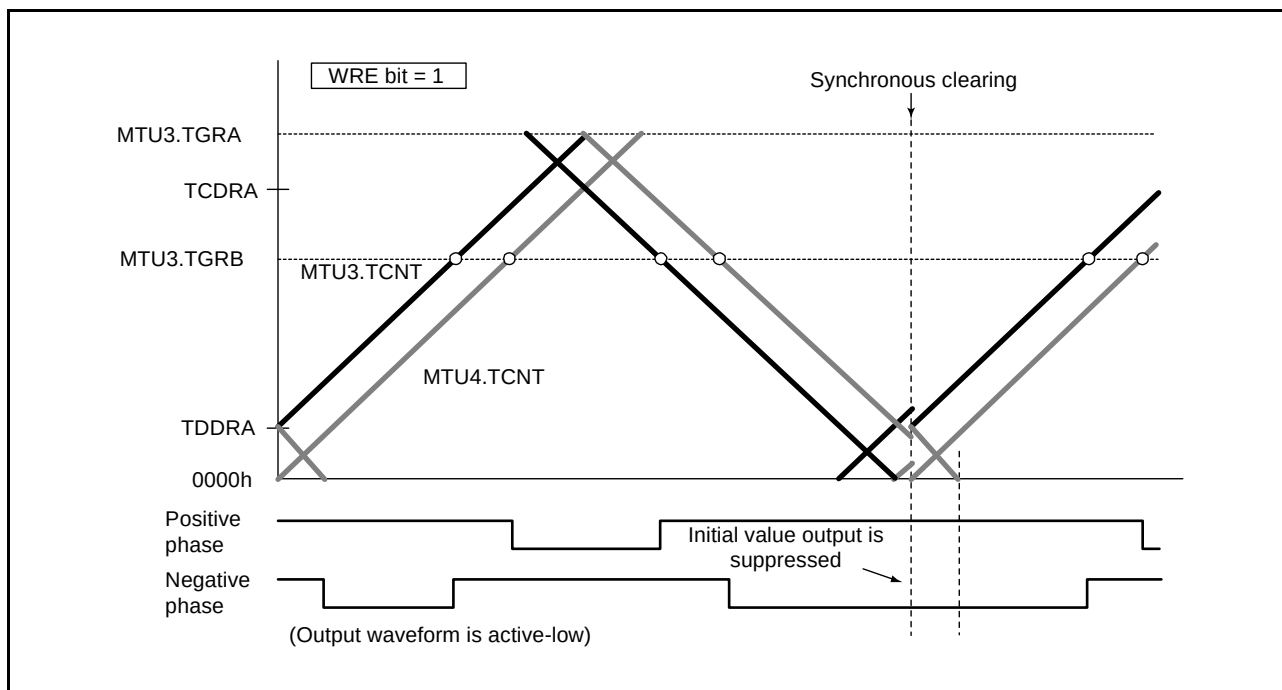
Figure 16.62 Example of Synchronous Clearing in Interval Tb at Trough (Timing (11) in Figure 16.57; Bit WRE of TWCRB is 1)
