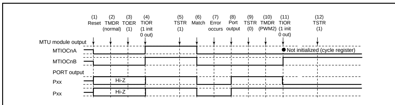
Figure 16.143 Error Occurrence in Normal Mode, Recovery in PWM Mode 2
