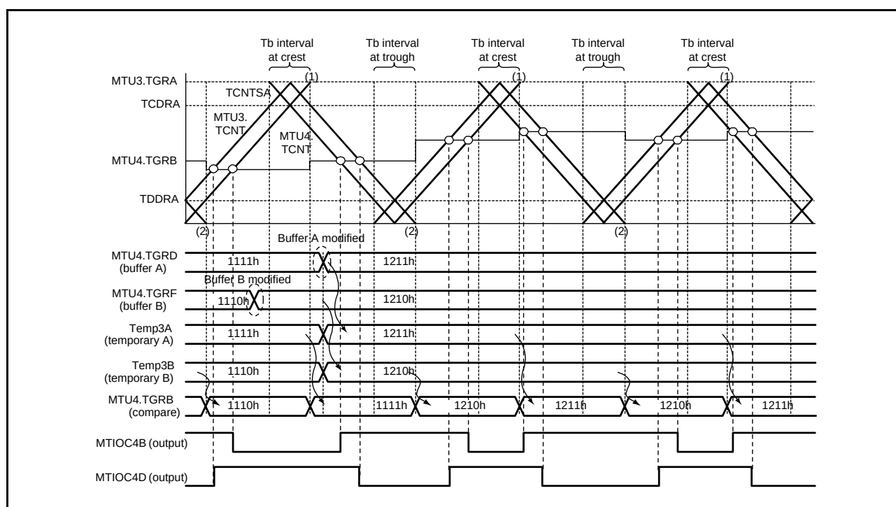
Figure 16.74 Example of Double Buffer Operation
