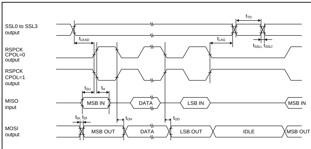
Figure 33.12 RSPI Timing (Master, CPHA = 0)
