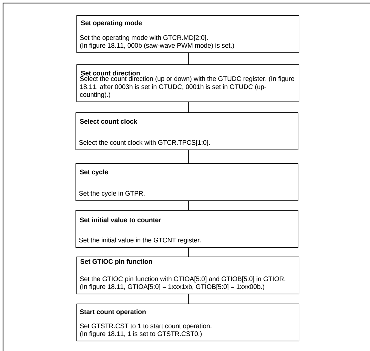
Figure 18.12 Example for Setting Input Capture Operation
