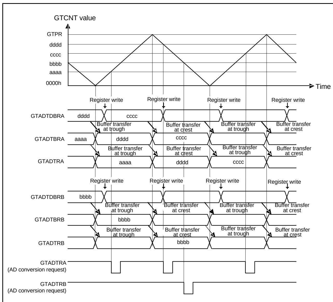
Figure 18.75 Example of A/D Converter Start Request Timing Operation (Triangle Waves, Double Buffer Operation, Buffer Transfer at Both Troughs and Crests, A/D Converter Start Requested by GTADTRA0 at Both Up-Counting and Down-Counting, A/D Converter Start Requested by GTADTRB0 at Down-Counting,)
