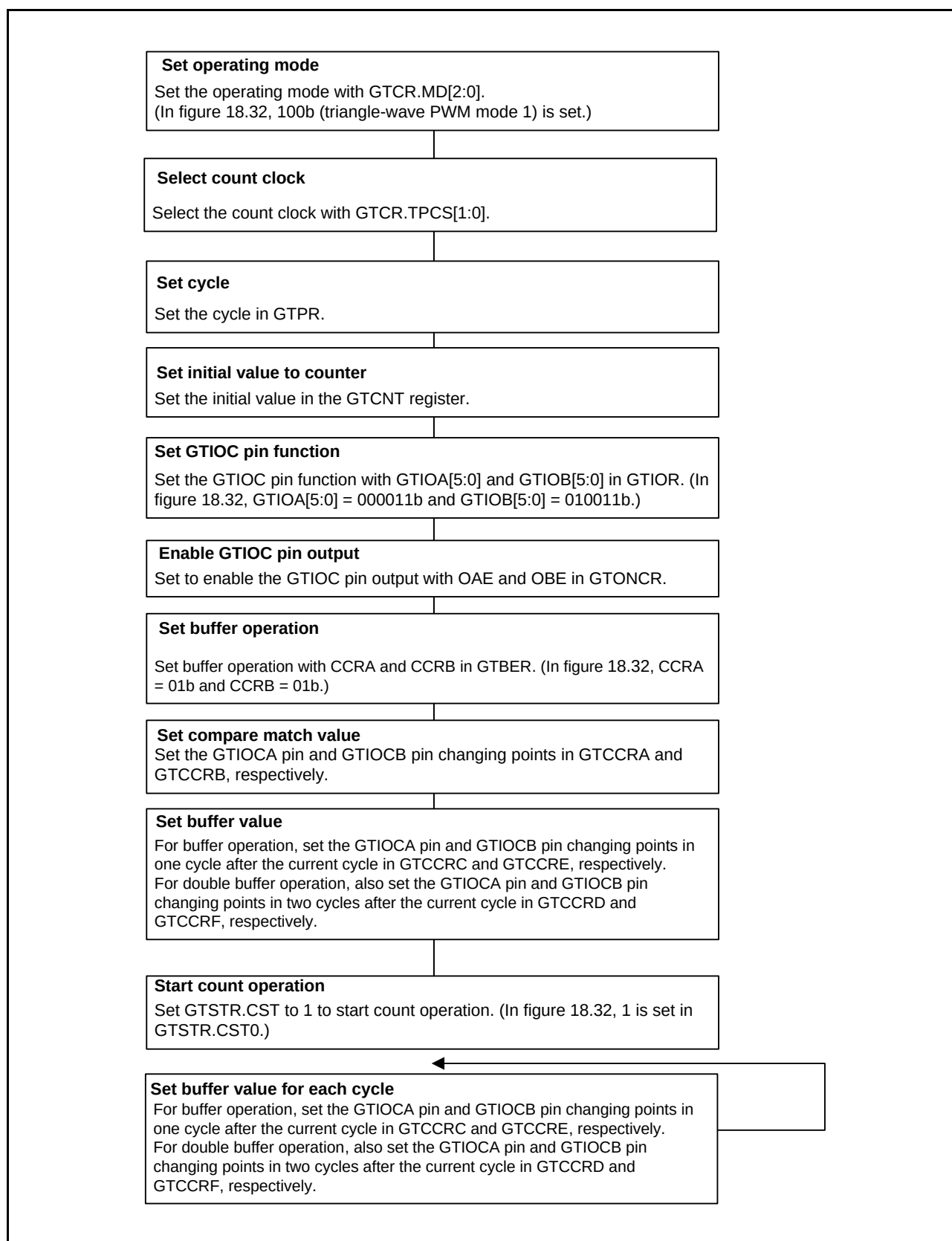
Figure 18.33 Example for Setting Triangle-Wave PWM Mode 1
