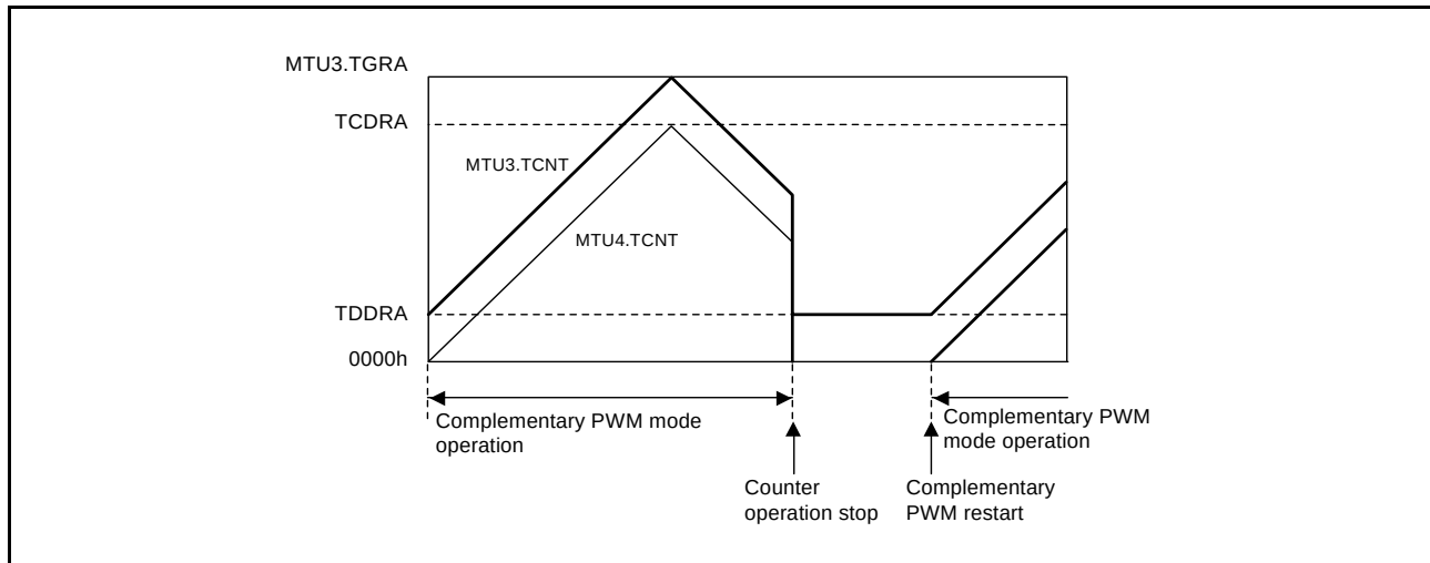
Figure 16.136 Counter Value when Stopped in Complementary PWM Mode
