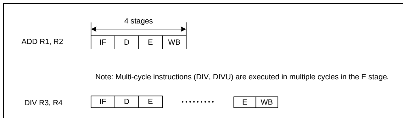
Figure 2.11 Operation for Register-Register, Immediate-Register
