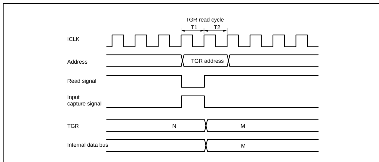
Figure 16.131 Contention between TGR Read Operation and Input Capture (MTU5)
