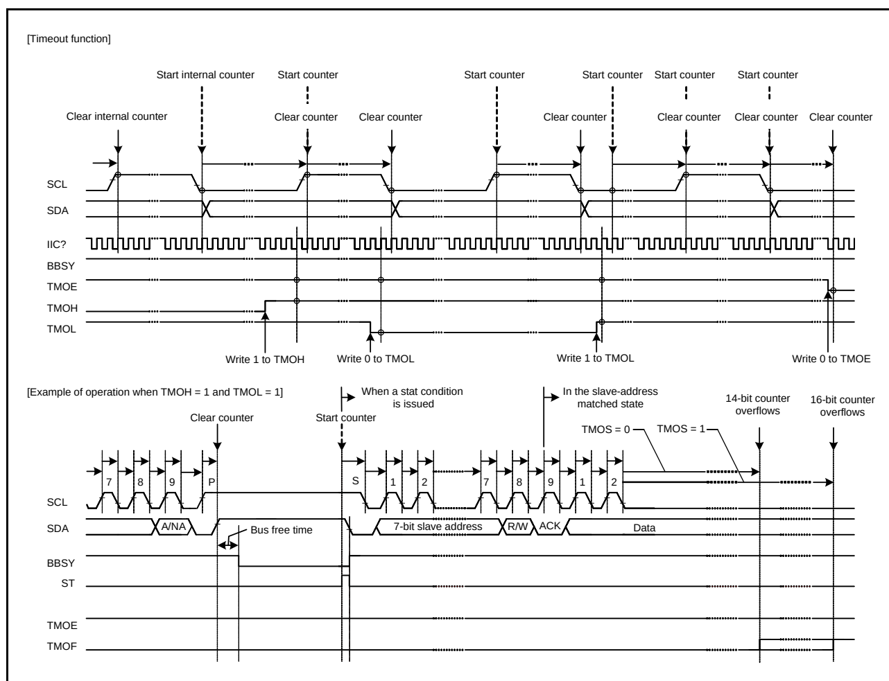
Figure 24.38 Timeout Function (TMOE, TMOS, TMOH, and TMOL Bits)
