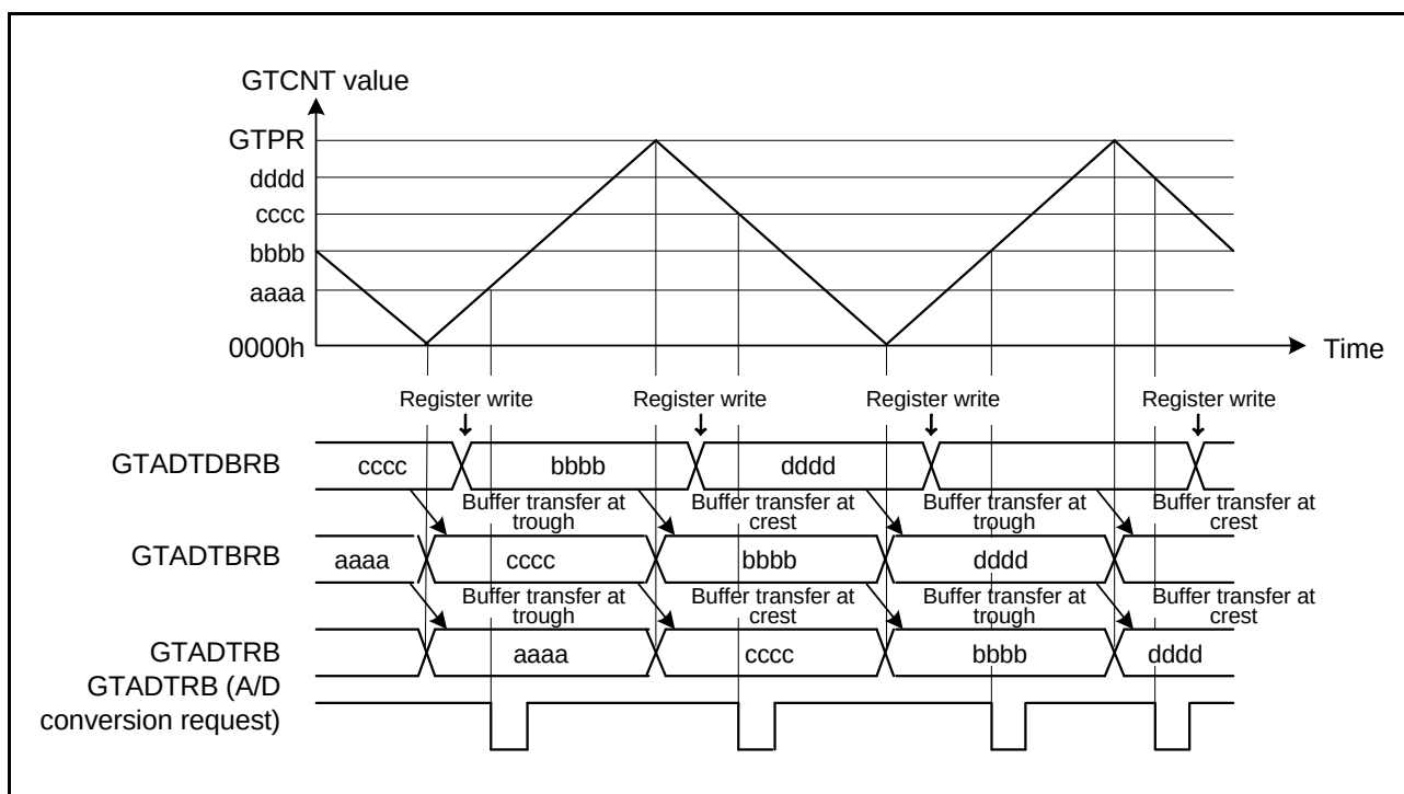
Figure 18.26 Example of GTADTRA and GTADTRB Double Buffer Operation (Triangle Waves, Buffer Transfer at Both Troughs and Crests, A/D Converter Start Request Generated by Both Up- and Down-Counting)
