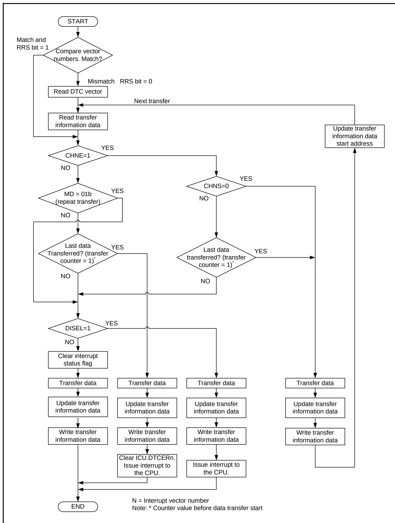
Figure 14.4 Operation Flowchart of the DTC
