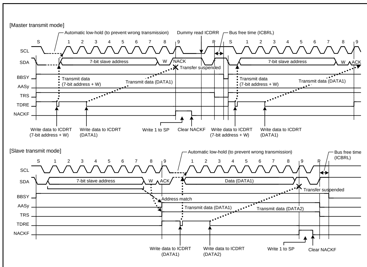
Figure 24.30 Suspension of Data Transfer when NACK is Received (NACKIE = 1)
