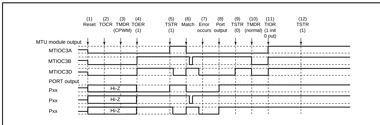
Figure 16.161 Error Occurrence in Complementary PWM Mode, Recovery in Normal Mode
