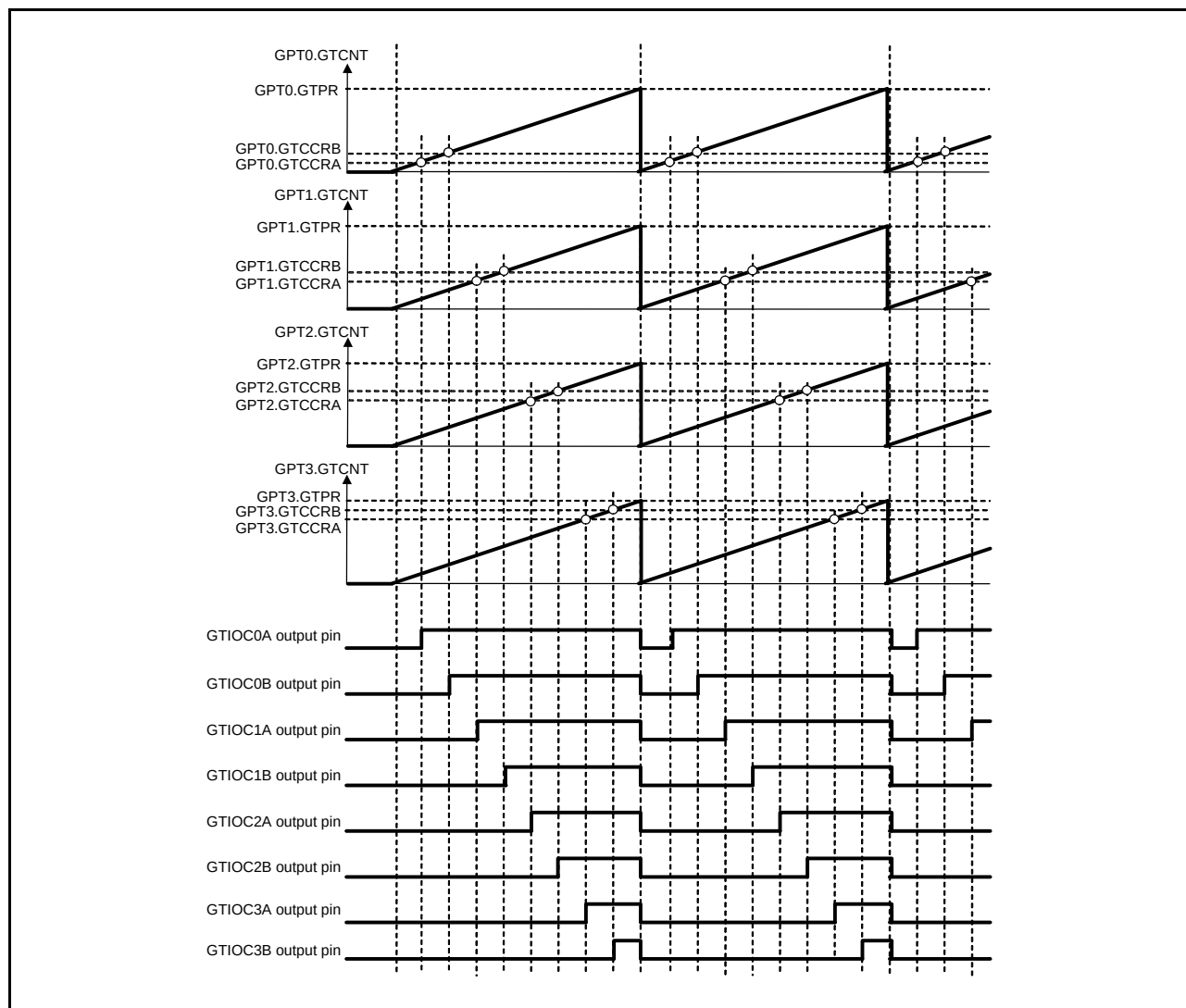
Figure 18.63 Example of Synchronized PWM Output
