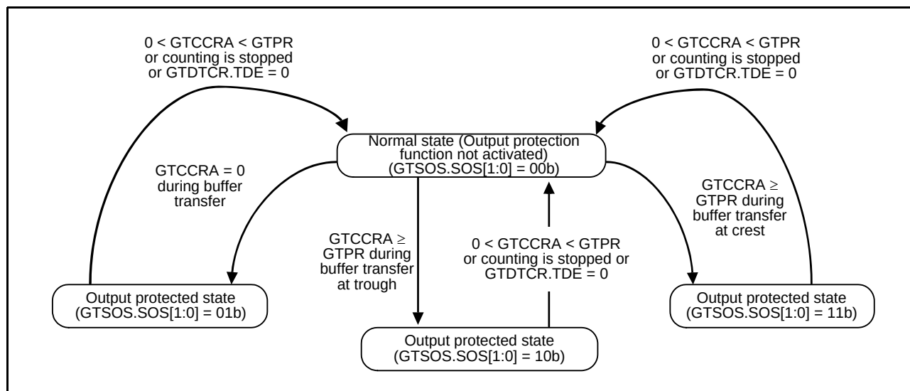
Figure 18.83 Output Protection Function
