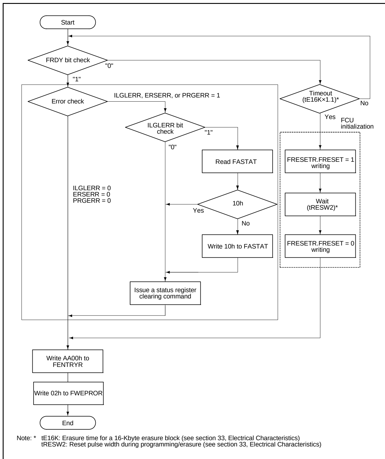
Figure 31.7 Procedure for Transition to ROM Read Mode
