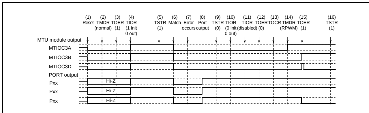
Figure 16.146 Error Occurrence in Normal Mode, Recovery in Reset-Synchronized PWM Mode
