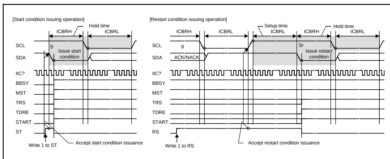
Figure 24.36 Start Condition/Restart Condition Issue Timing (ST and RS Bits)
