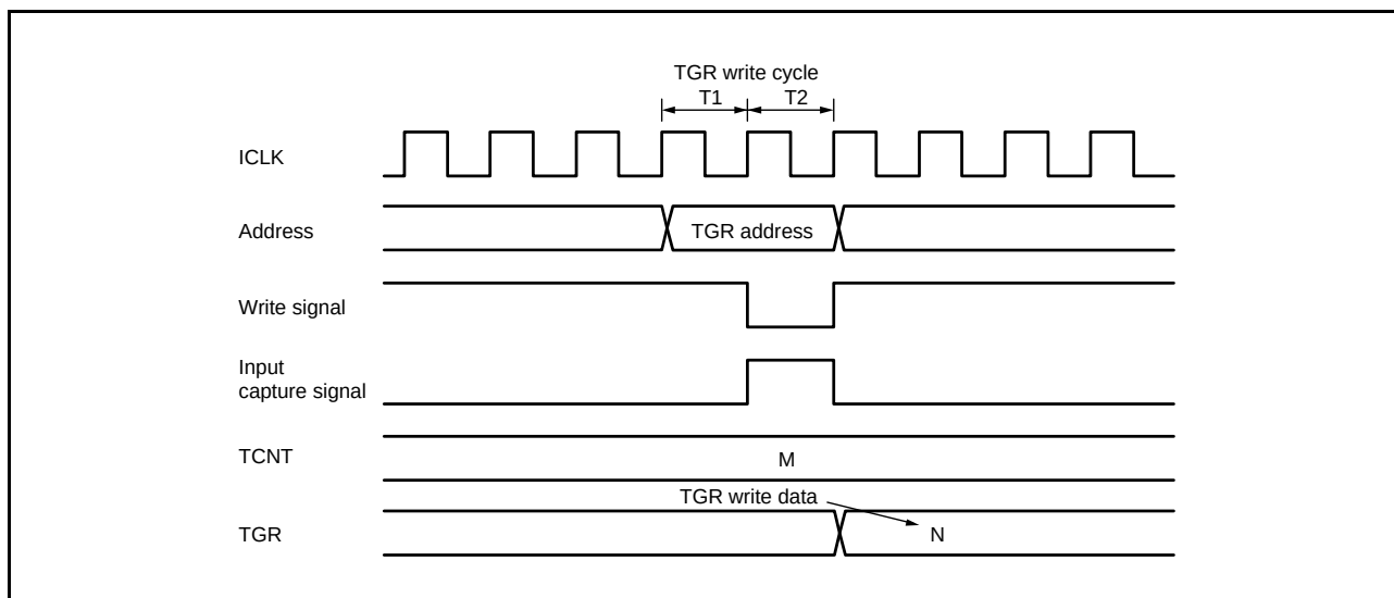
Figure 16.133 Contention between TGR Write Operation and Input Capture (MTU5)
