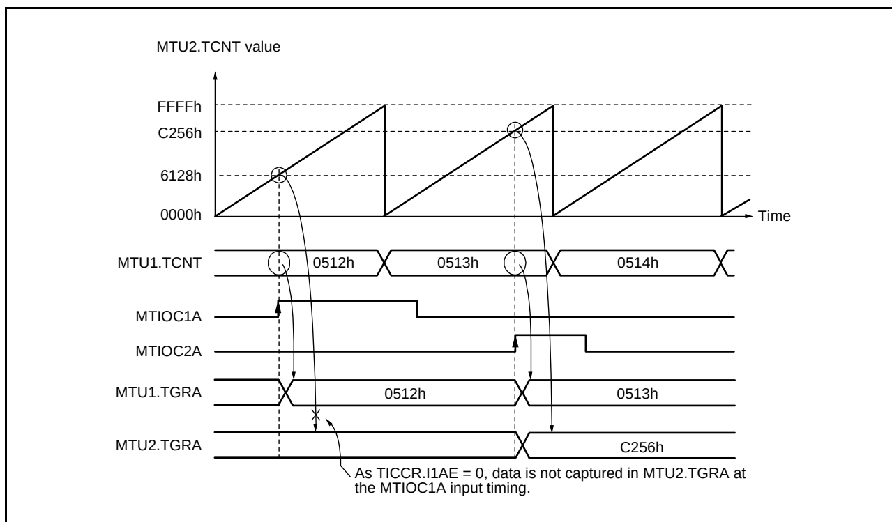
Figure 16.23 Cascaded Operation Example (b)
