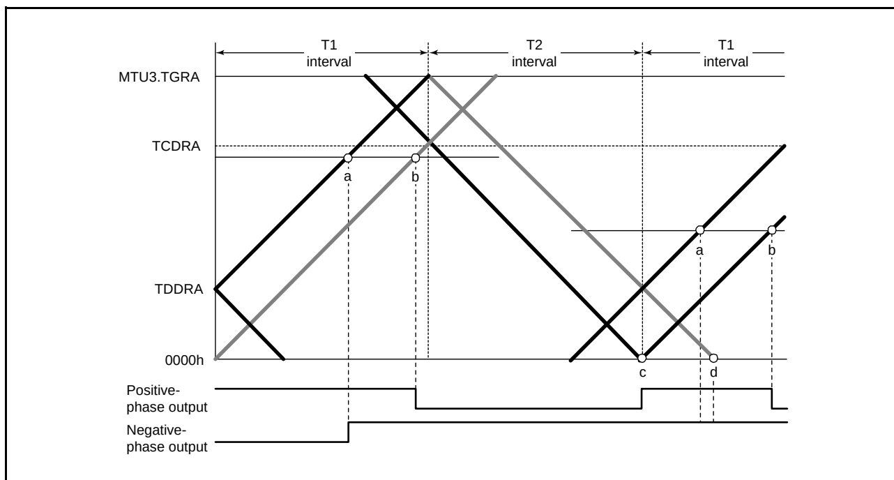
Figure 16.51 Example of 0% and 100% Waveform Output in Complementary PWM Mode (MTU3 and MTU4) (2)
