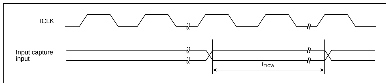
Figure 33.16 MTU3 Input/Output Timing
