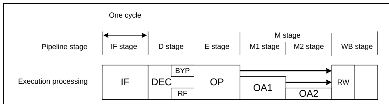
Figure 2.10 Pipeline Configuration and its Operation
