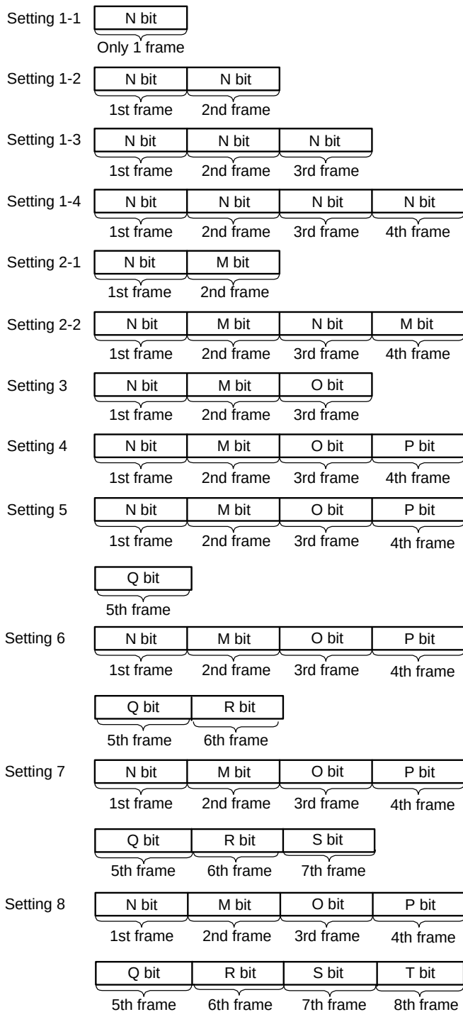
Figure 26.2 Frame Configurations and Examples of Combinations of Transmission and Reception Settings
