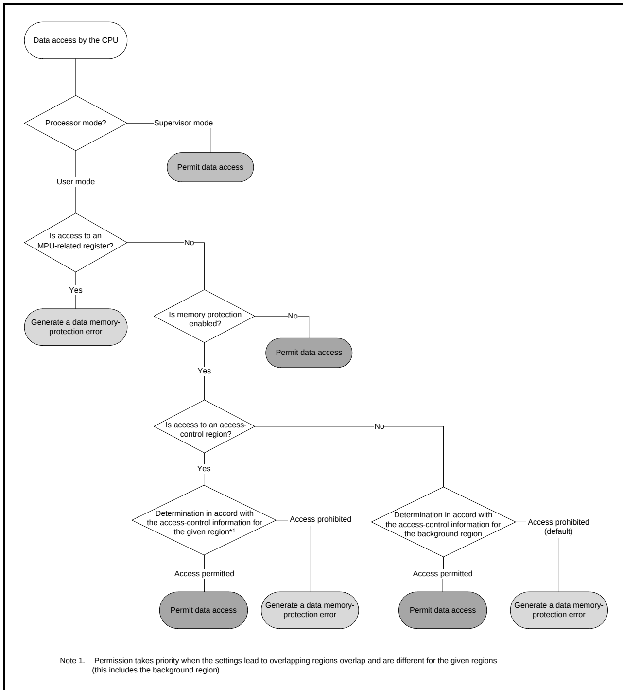
Figure 13.2 Flow of Determination for Data Access
