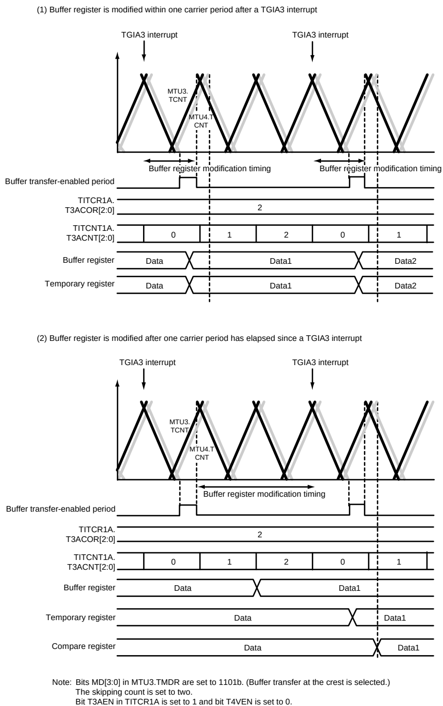
Figure 16.81 Example of Operation when Buffer Transfer is Linked with Interrupt Skipping (BTE[1:0] = 10b)
