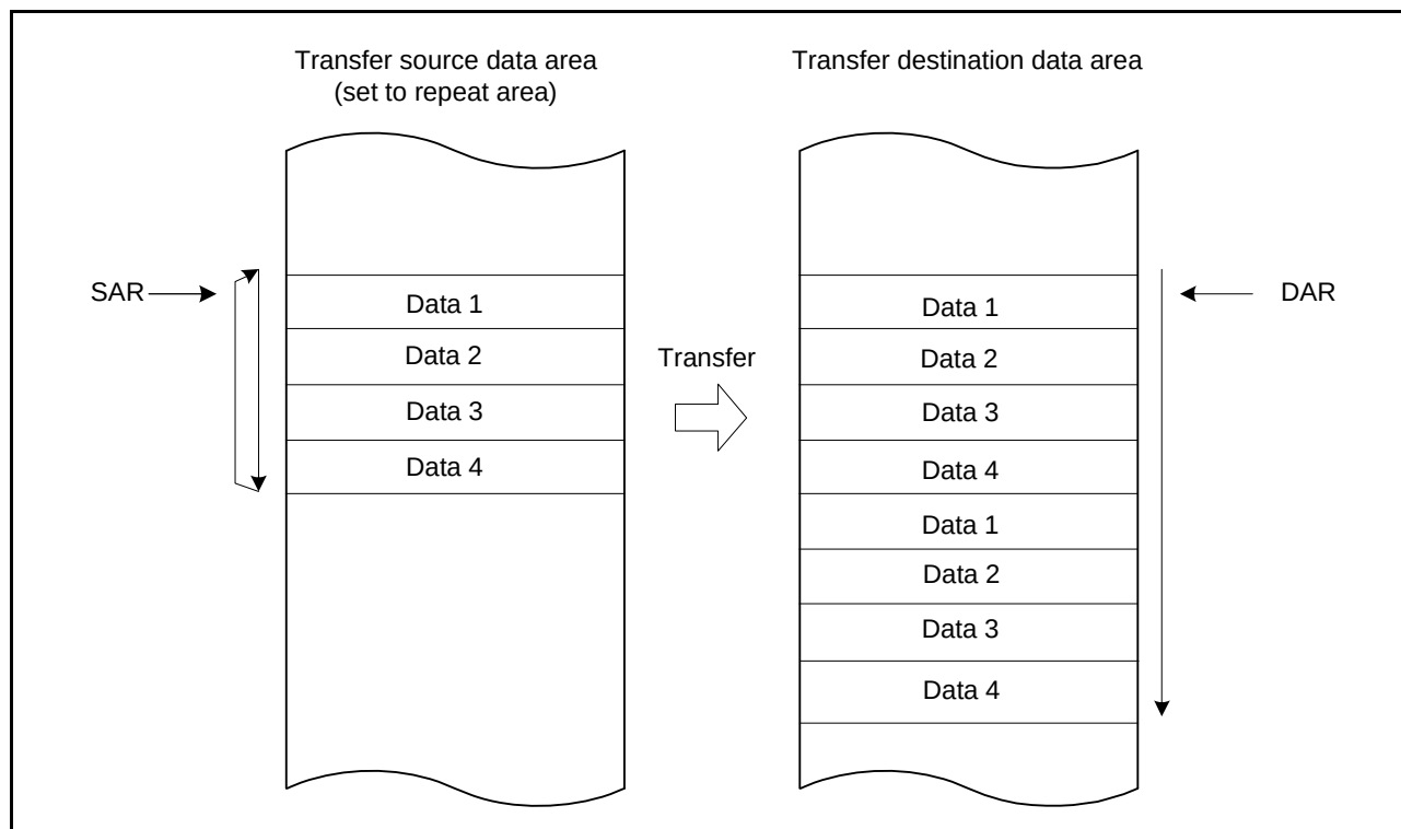
Figure 14.6 Memory Map of Repeat Transfer Mode (Transfer Source: Repeat Area)
