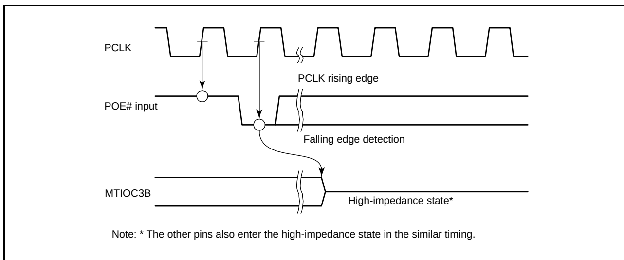
Figure 17.3 Falling Edge Detection
