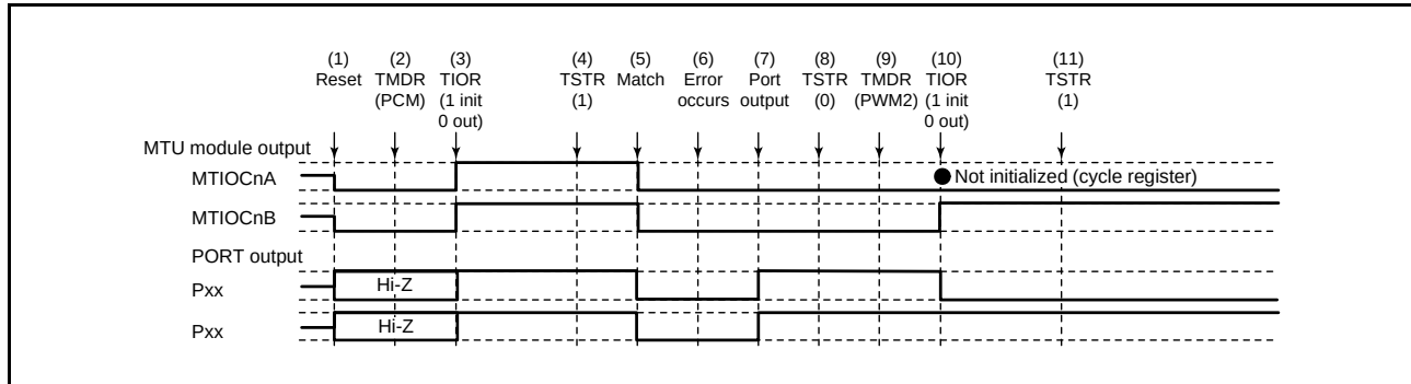
Figure 16.159 Error Occurrence in Phase Counting Mode, Recovery in PWM Mode 2
