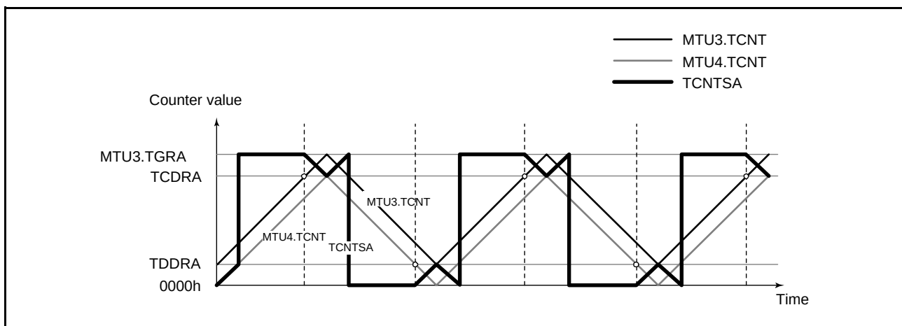
Figure 16.40 Counter Operation in Complementary PWM Mode
