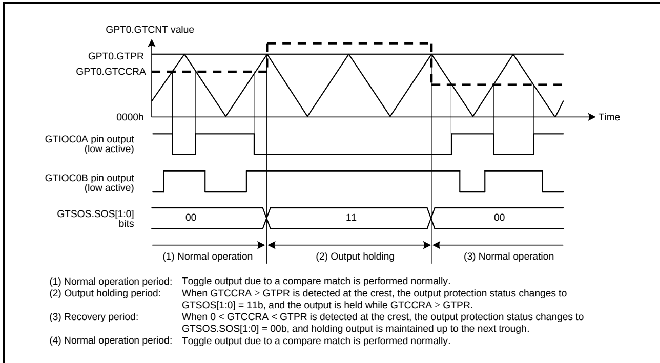
Figure 18.90 Example of Output Protection Function Operation When GTCCRA \geq GTPR is Set during Buffer Transfer at Crests (Restored to 0 < GTCCRA < GTPR during Buffer Transfer at Crests, Active Level: Low)
