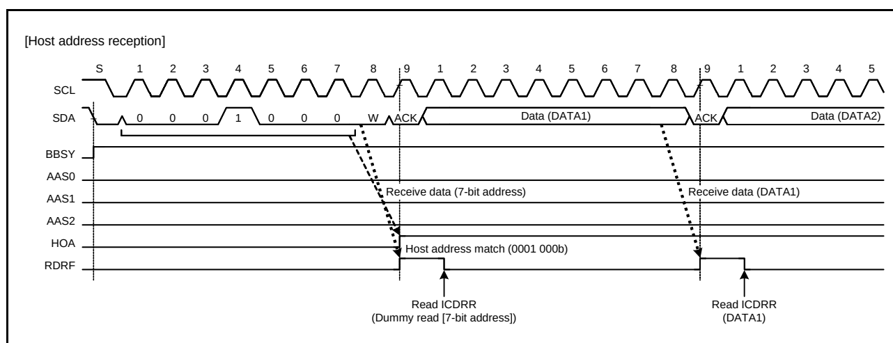
Figure 24.28 HOA Flag Set Timing during Reception of Host Address
