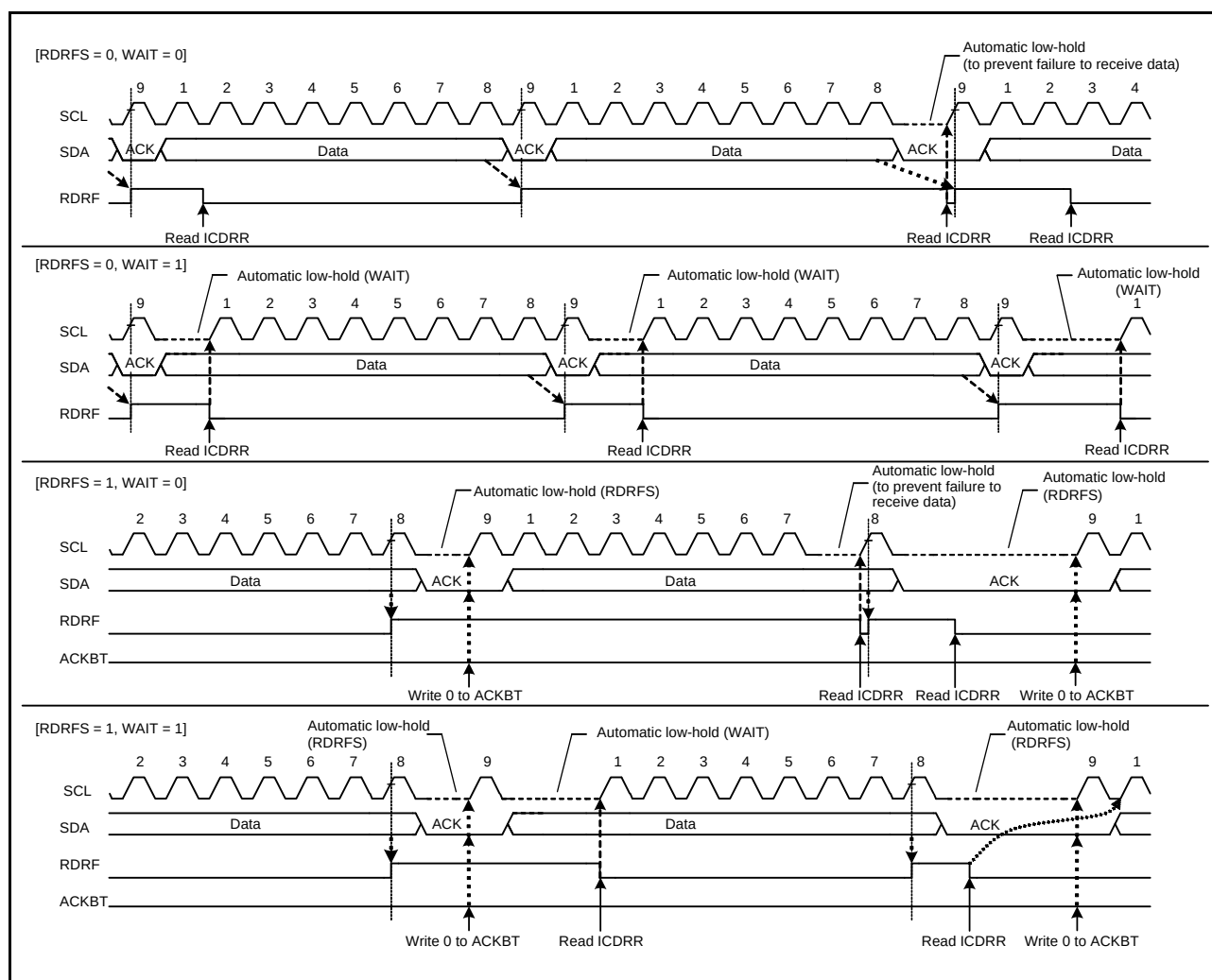
Figure 24.31 Automatic Low-Hold Operation in Receive Mode (Using RDRFS and WAIT Bits)
