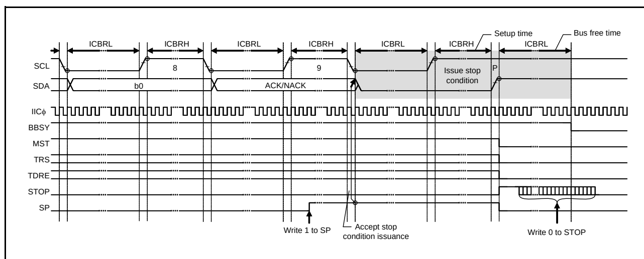
Figure 24.37 Stop Condition Issue Timing (SP Bit)
