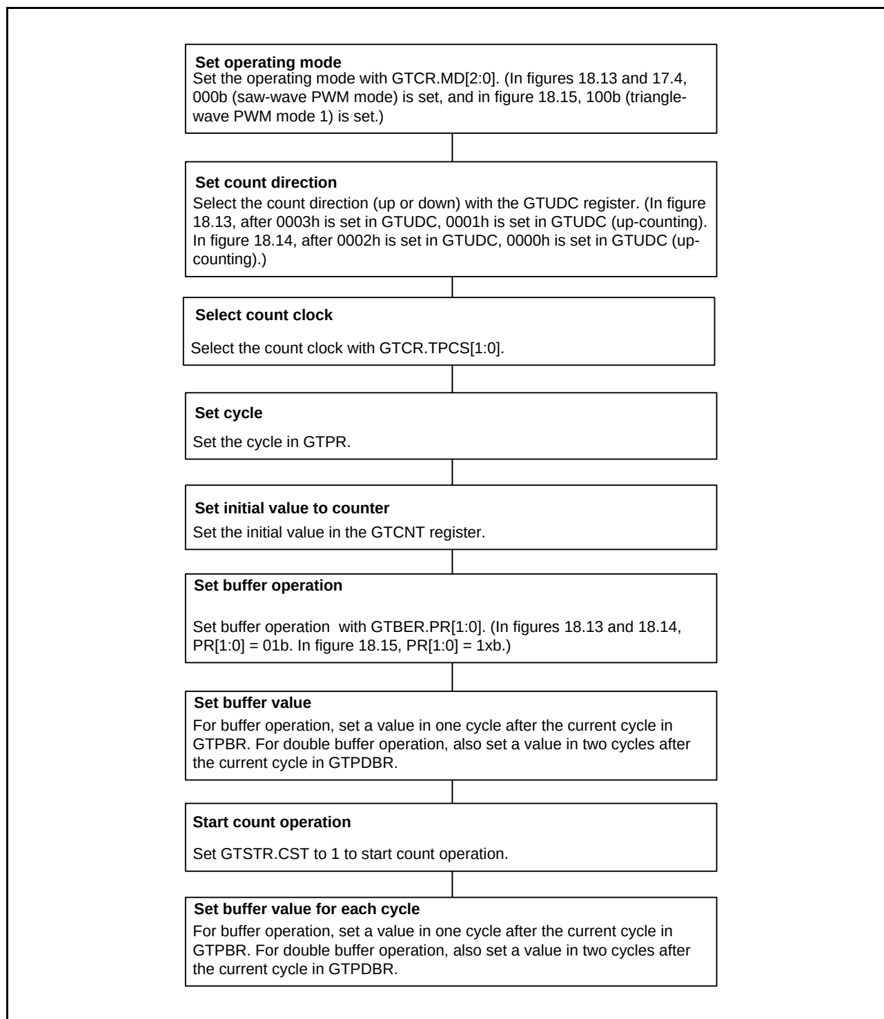
Figure 18.16 Example for Setting GTPR Buffer Operation
