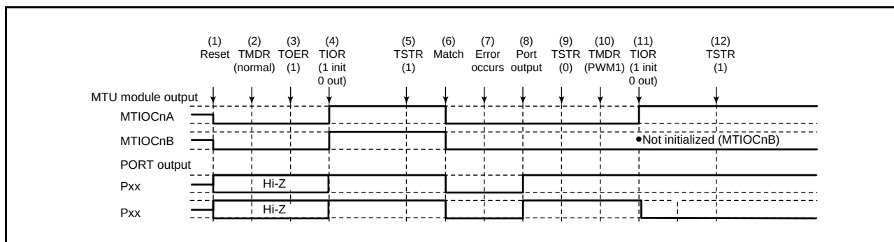
Figure 16.142 Error Occurrence in Normal Mode, Recovery in PWM Mode 1
