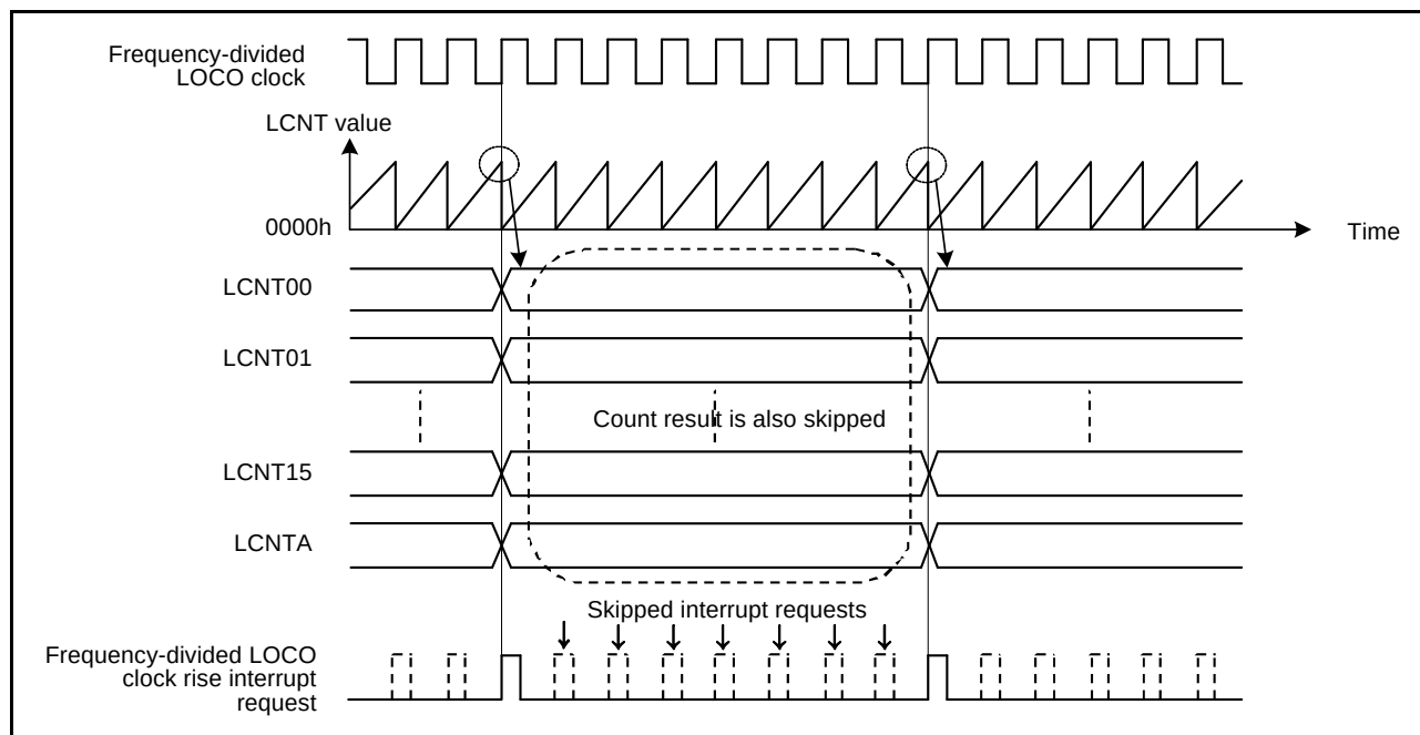
Figure 18.80 Example of LOCO Count Skipping Function Operation (Skipping Count: 7, Count Result Skipped)
