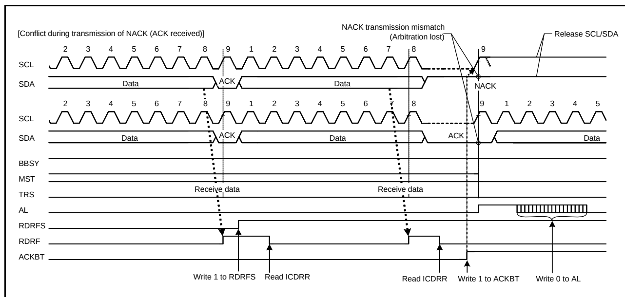
Figure 24.34 Example of Arbitration Lost Detection during Transmission of NACK (NALE = 1)
