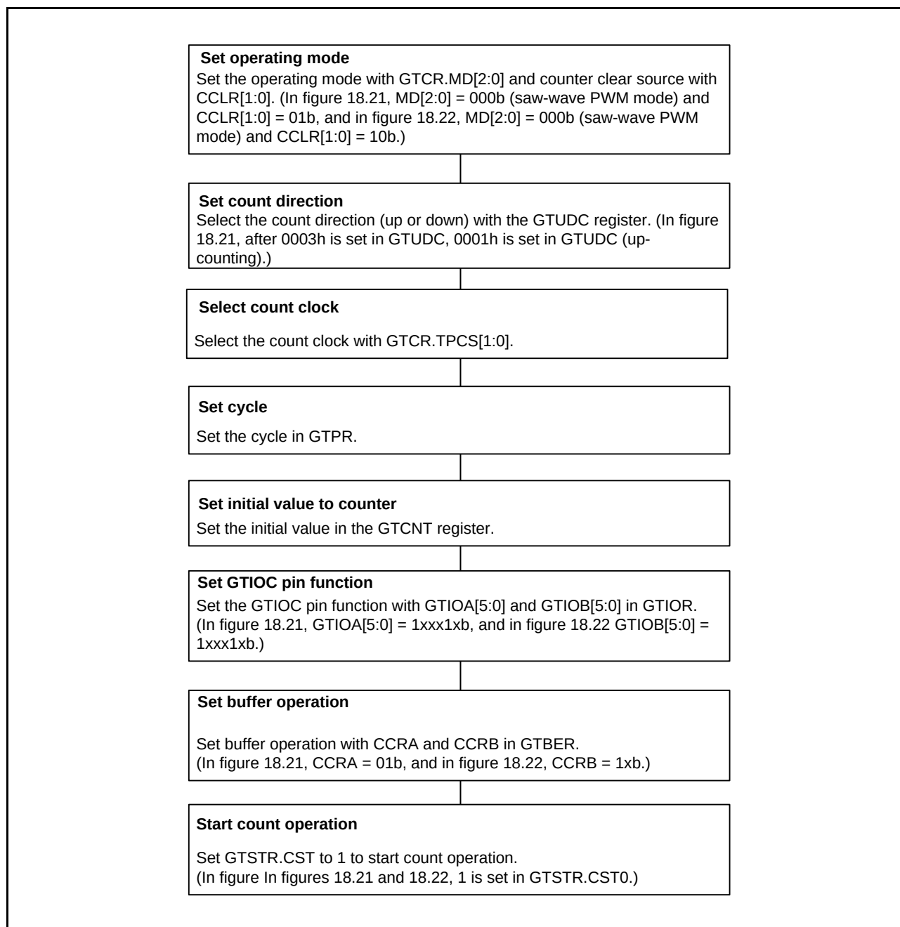
Figure 18.23 Example for Setting GTCRA and GTCCRB Buffer Operation (for Input Capture)
