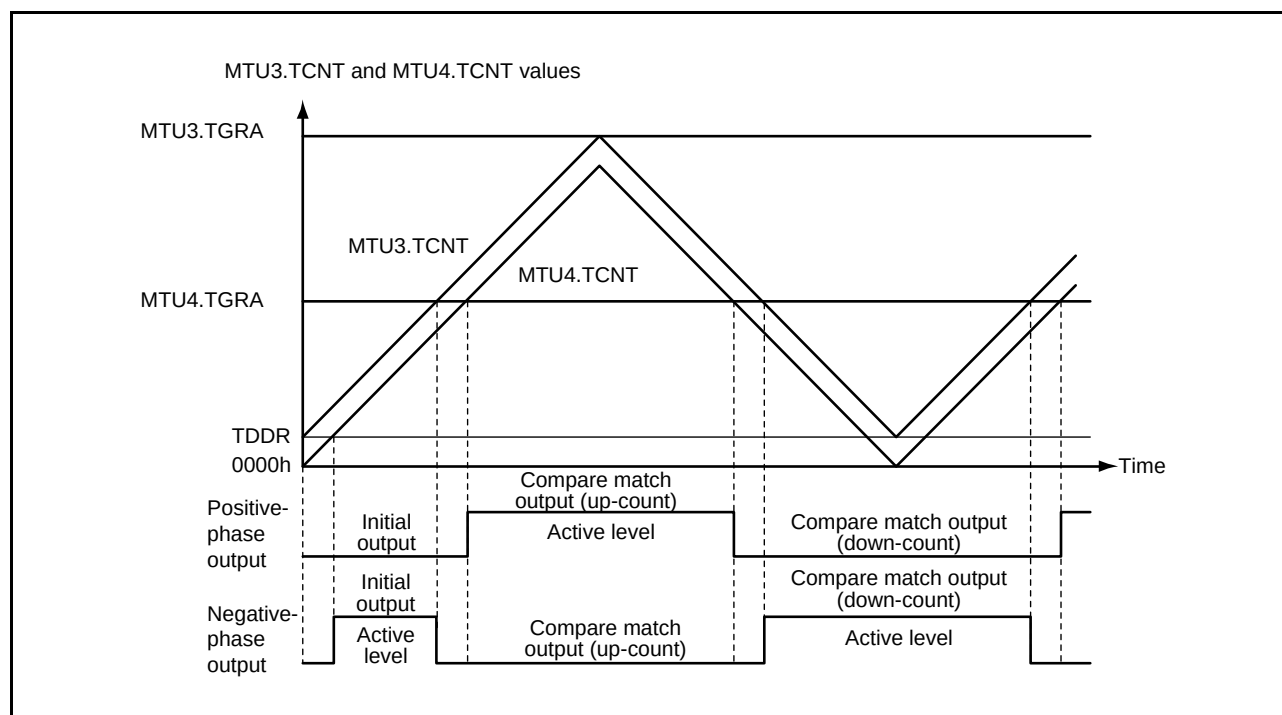
Figure 16.3 Example of Output in Complementary PWM Mode
