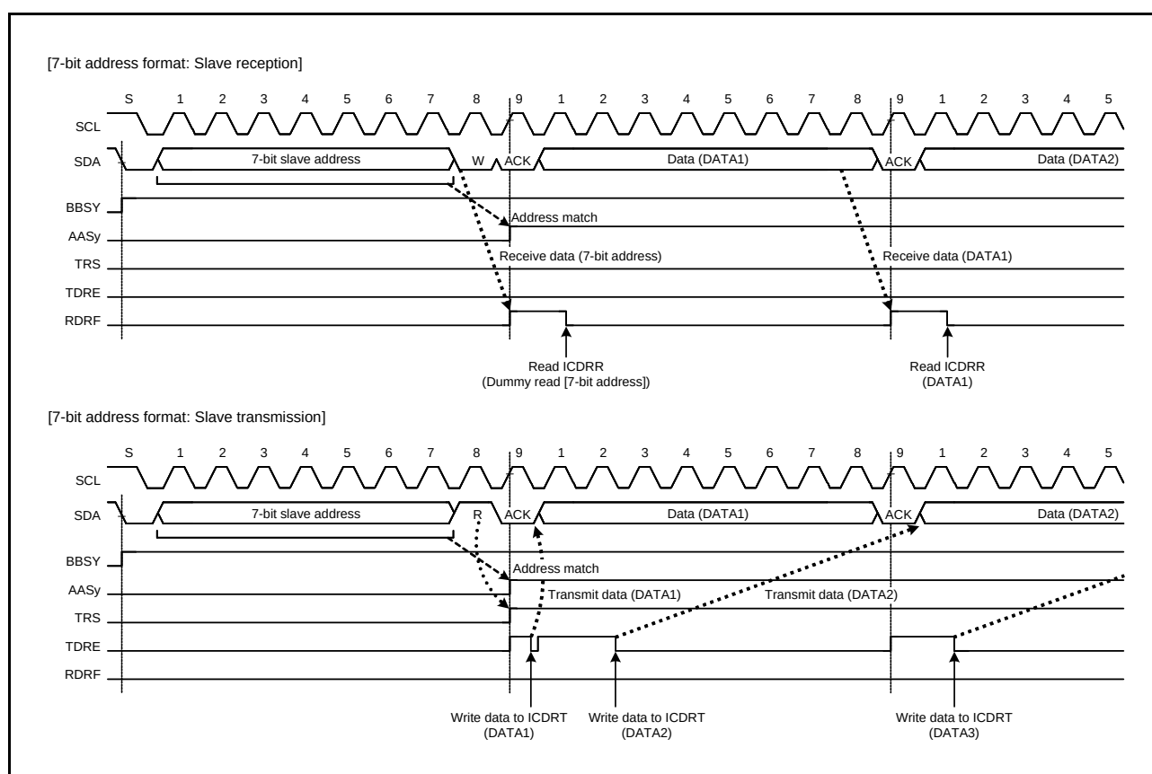
Figure 24.23 AASy Flag Set Timing with 7-Bit Address Format Selected
