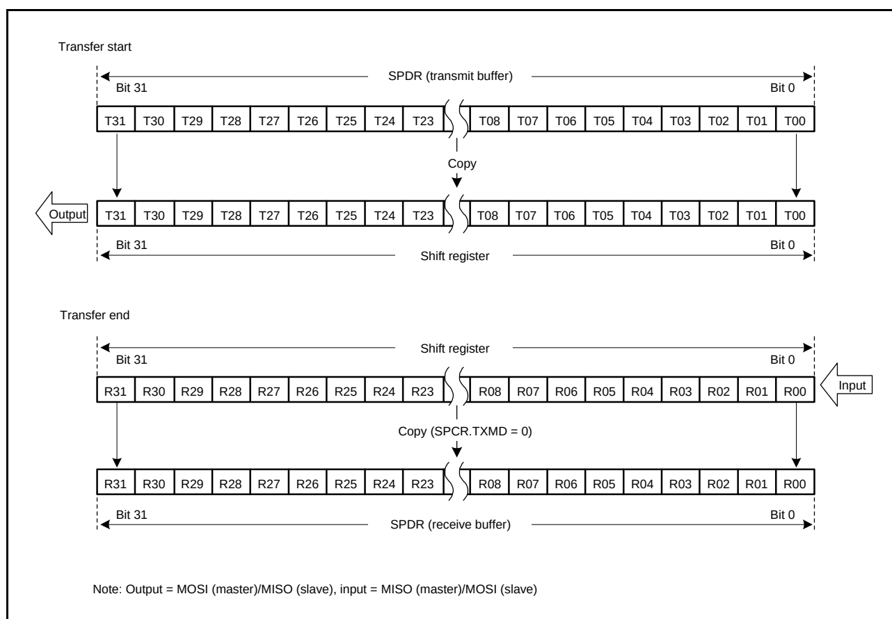
Figure 26.13 MSB First Transfer (1) (32-Bit Data, Parity Function Disabled)
