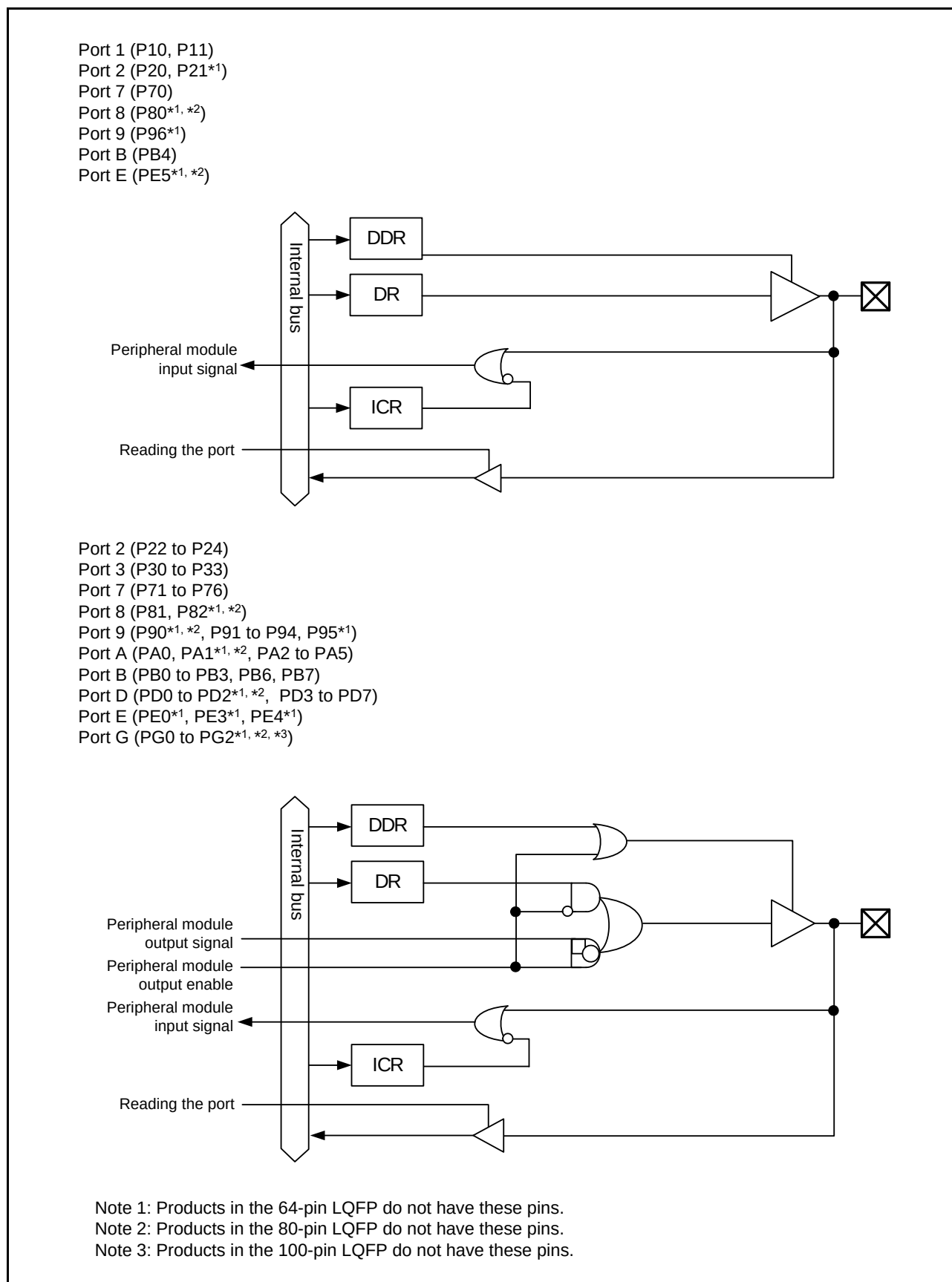
Figure 15.1 I/O Port Configuration (1)
