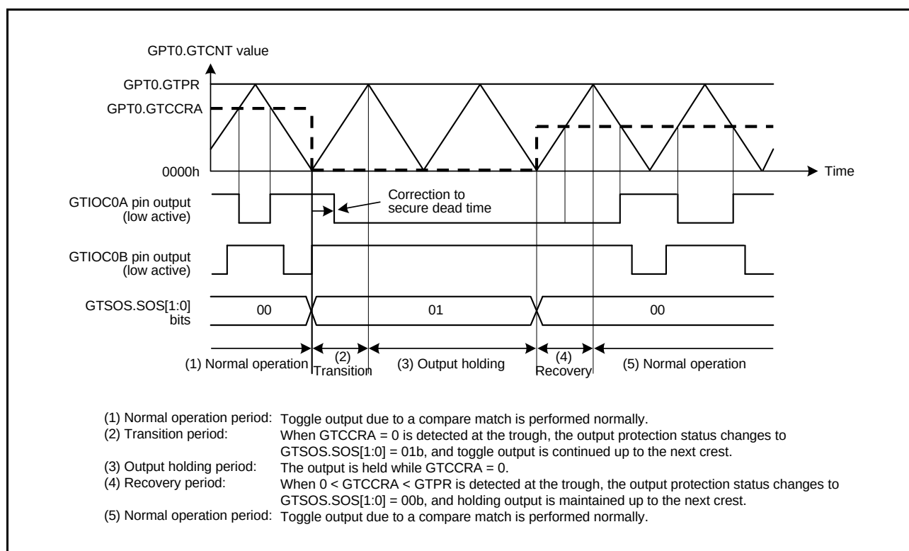
Figure 18.84 Example of Output Protection Function Operation When GTCCRA is Set to 0 during Buffer Transfer at Troughs (Restored to 0 < GTCCRA < GTPR during Buffer Transfer at Troughs, Active Level: Low)
