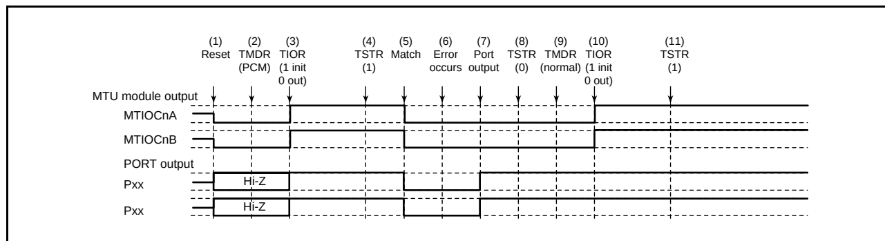
Figure 16.157 Error Occurrence in Phase Counting Mode, Recovery in Normal Mode
