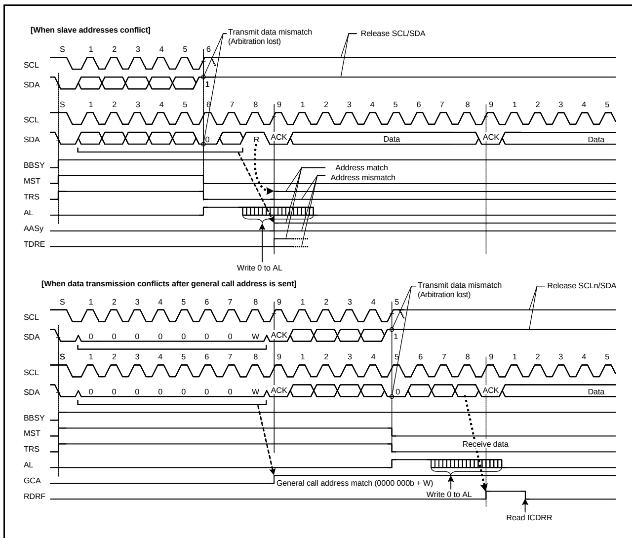
Figure 24.32 Examples of Master Arbitration Lost Detection (MALE = 1)
