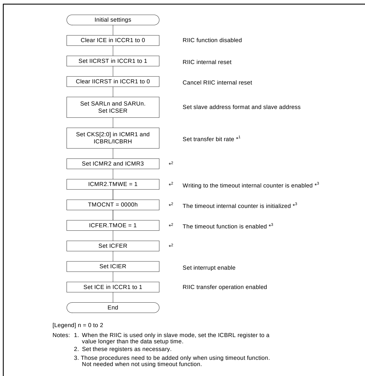
Figure 24.5 Example of RIIC Initialization Flow
