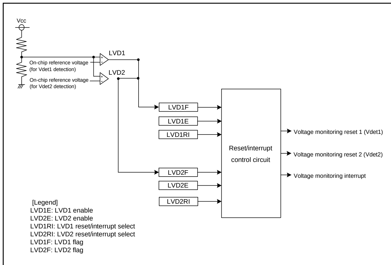
Figure 7.1 Block Diagram of Voltage Detection Circuit
