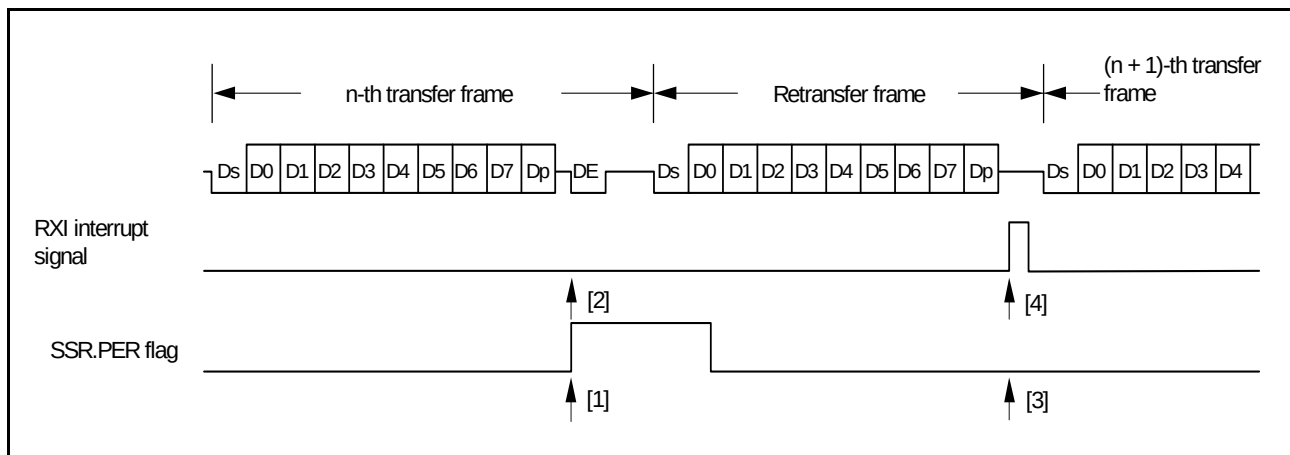
Figure 22.31 Data Retransfer Operation in SMC1 Reception Mode
