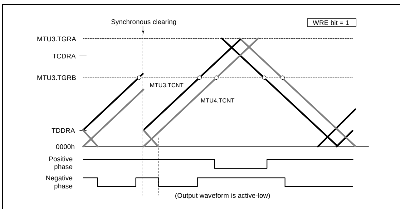
Figure 16.59 Example of Synchronous Clearing in Dead Time during Up-Counting (Timing (3) in Figure 16.57; Bit WRE of TWCR or TWCRB is 1)
