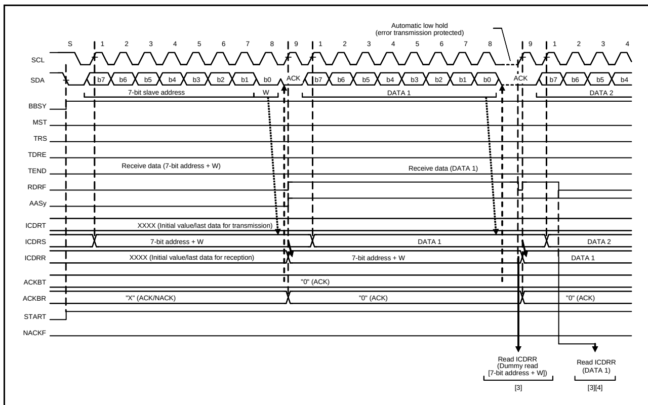
Figure 24.18 Slave Receive Operation Timing (1) (7-Bit Address Format, when RDRFS=0)
