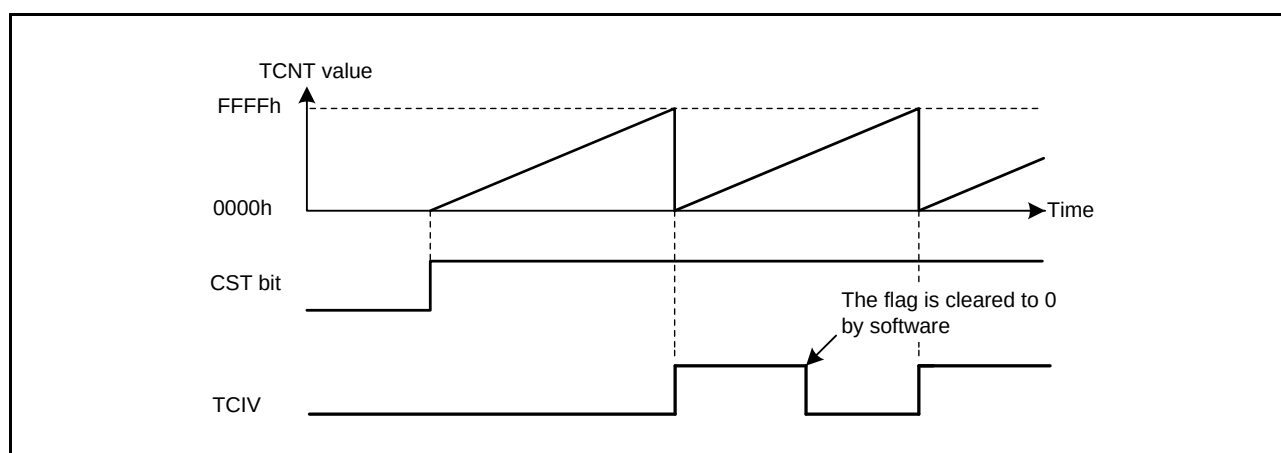
Figure 16.6 Free-Running Counter Operation
