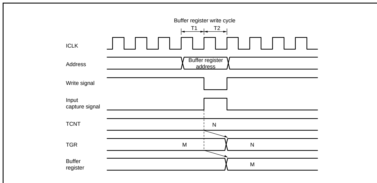
Figure 16.134 Contention between Buffer Register Write Operation and Input Capture
