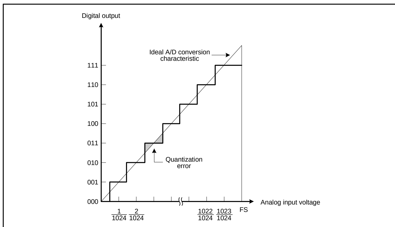
Figure 29.7 A/D Conversion Accuracy Definitions (1)
