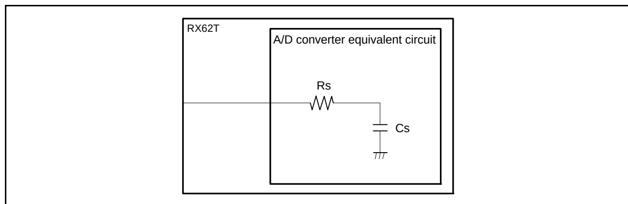
Figure 28.11 Equivalent Circuit for the Internal Circuit of Analog Input Pins
