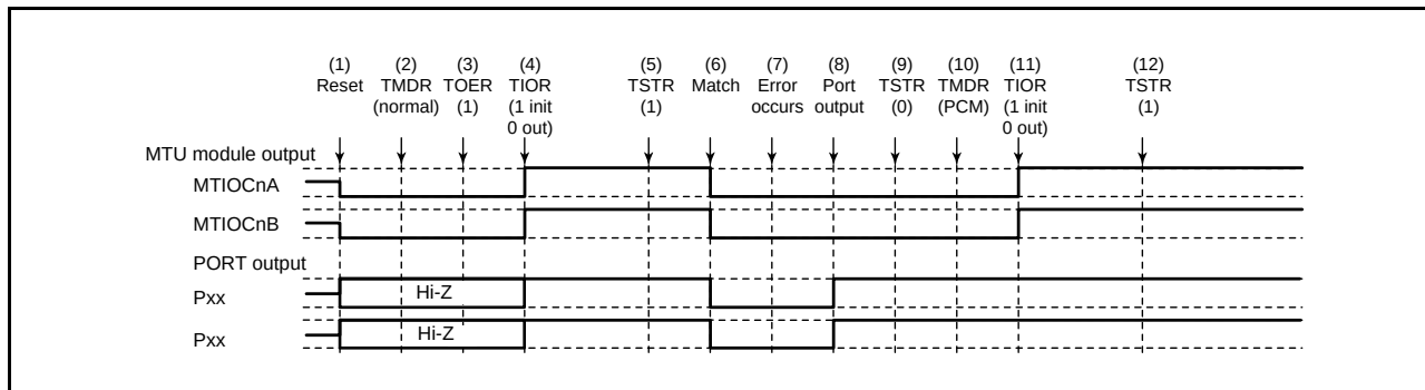
Figure 16.144 Error Occurrence in Normal Mode, Recovery in Phase Counting Mode
