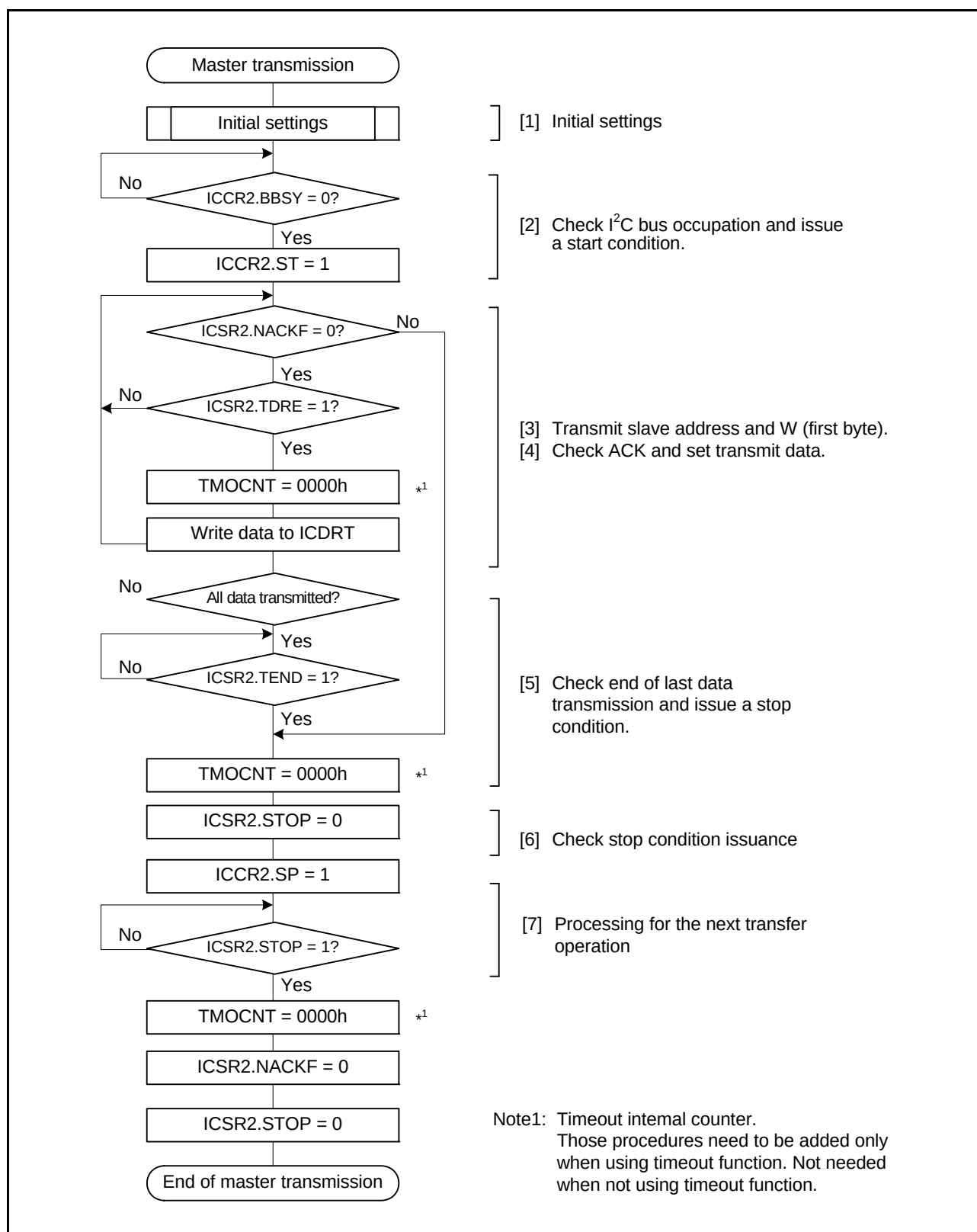
Figure 24.6 Example of Master Transmission Flowchart
