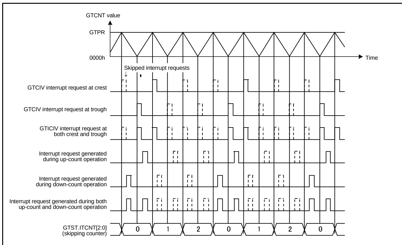
Figure 18.69 Example of Interrupt Skipping Function Operation (Triangle Waves, Counting and Skipping Crests, Skipping Count: 2)
