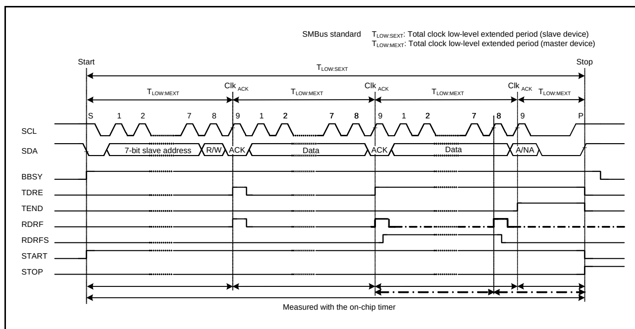
Figure 24.40 SMBus Timeout Measurement
