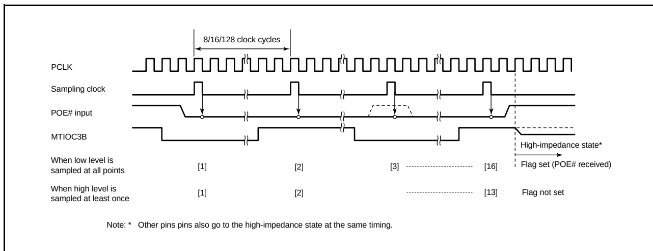
Figure 17.4 Low-Level Detection Operation
