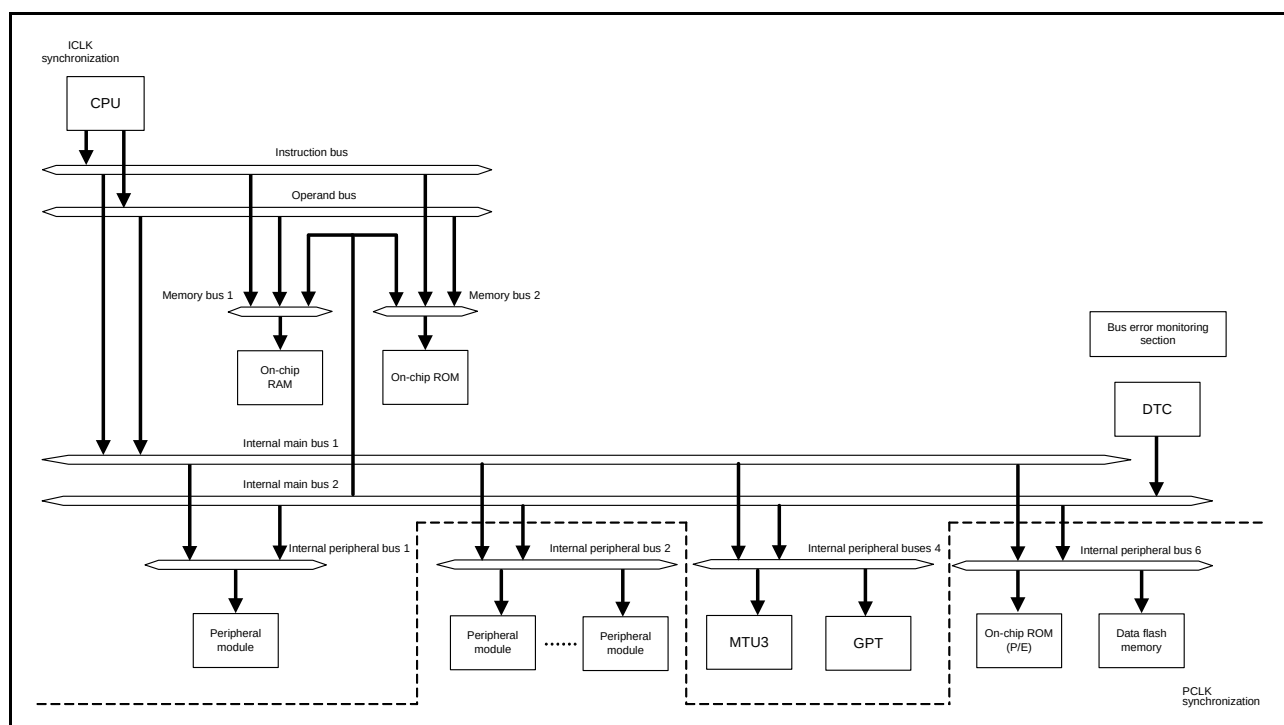
Figure 12.1 Bus Configuration
