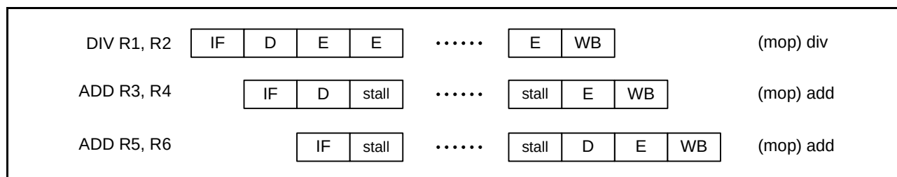
Figure 2.20 When an Instruction which Requires Multiple Cycles is Executed in the E Stage
