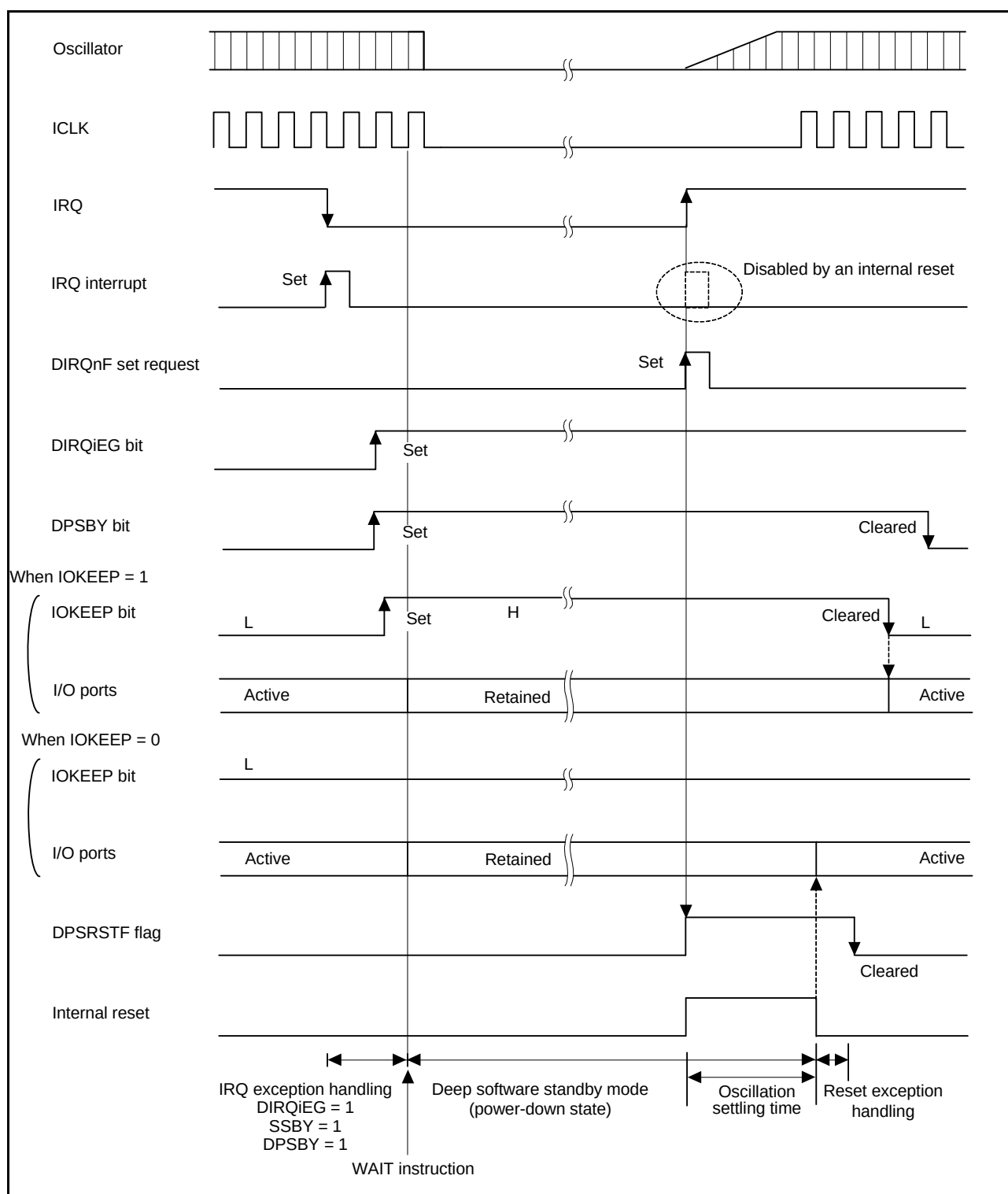
Figure 9.3 Example of Deep Software Standby Mode Application
