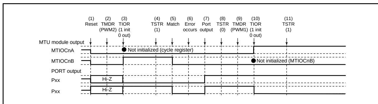
Figure 16.154 Error Occurrence in PWM Mode 2, Recovery in PWM Mode 1
