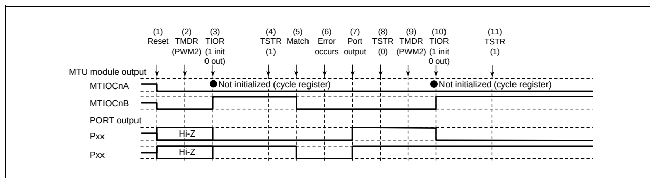
Figure 16.155 Error Occurrence in PWM Mode 2, Recovery in PWM Mode 2
