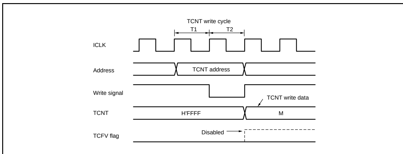
Figure 16.140 Contention between TCNT Write Operation and Overflow
