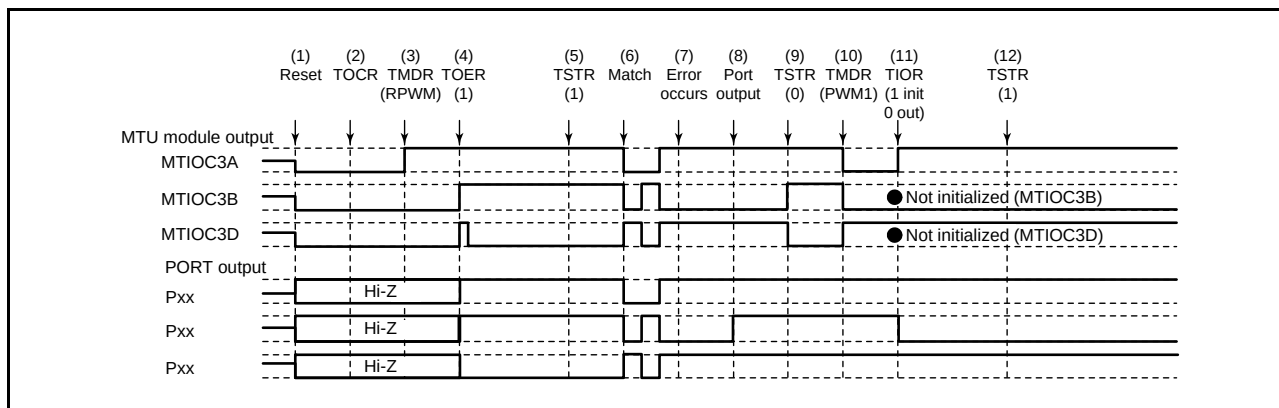
Figure 16.167 Error Occurrence in Reset-Synchronized PWM Mode, Recovery in PWM Mode 1
