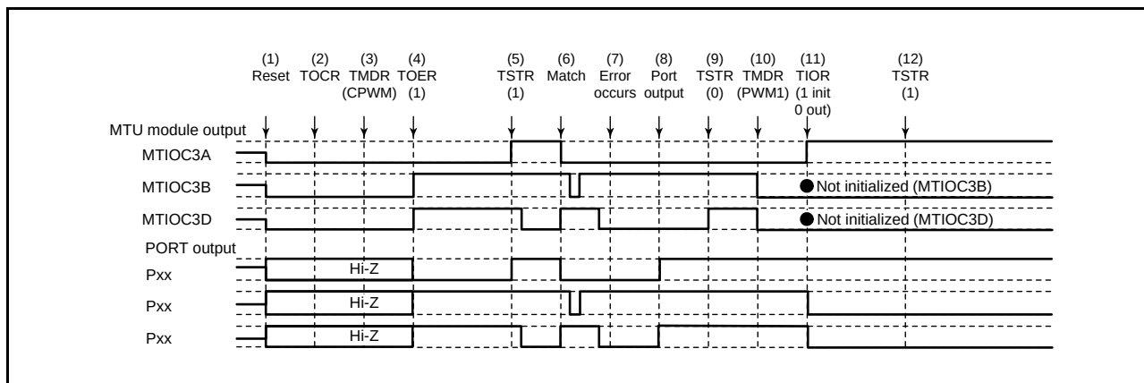
Figure 16.162 Error Occurrence in Complementary PWM Mode, Recovery in PWM Mode 1
