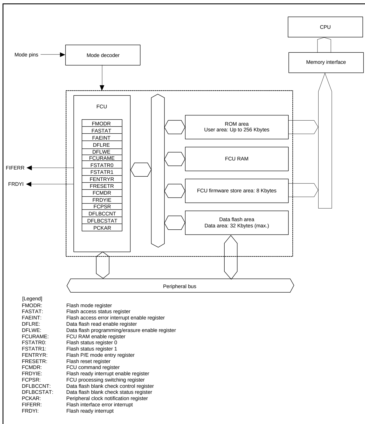
Figure 31.1 Block Diagram of ROM
