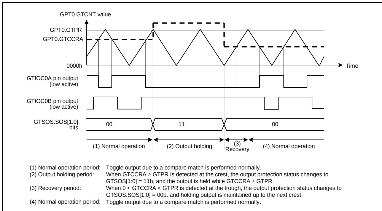
Figure 18.91 Example of Output Protection Function Operation When GTCCRA \geq GTPR is Set during Buffer Transfer at Crests (Restored to 0 < GTCCRA < GTPR during Buffer Transfer at Troughs, Active Level: Low)
