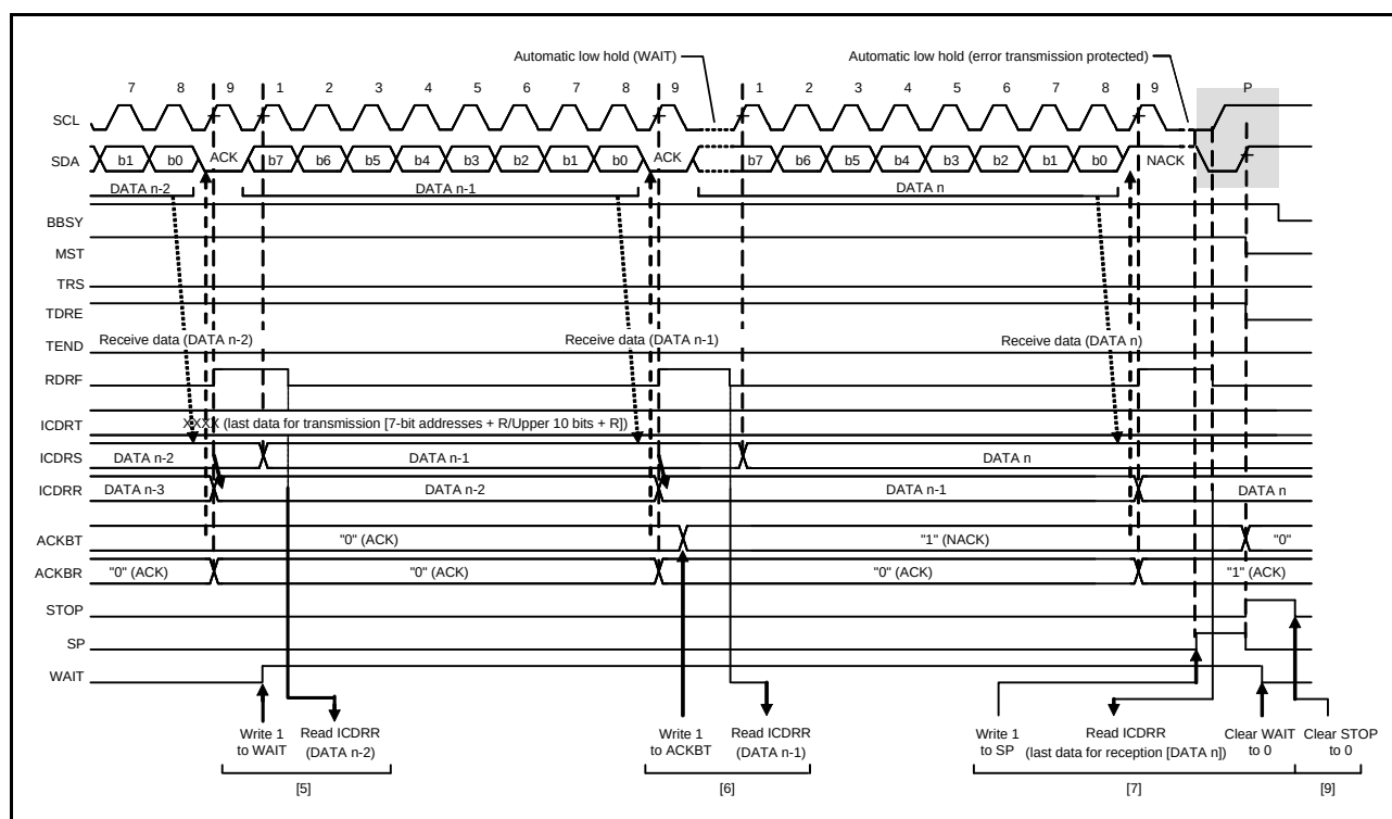
Figure 24.13 Master Receive Operation Timing (3) (when RDRFS=0)
