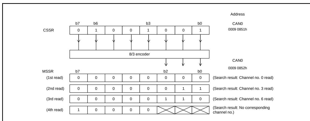
Figure 25.4 Write and Read of CSSR and MSSR
