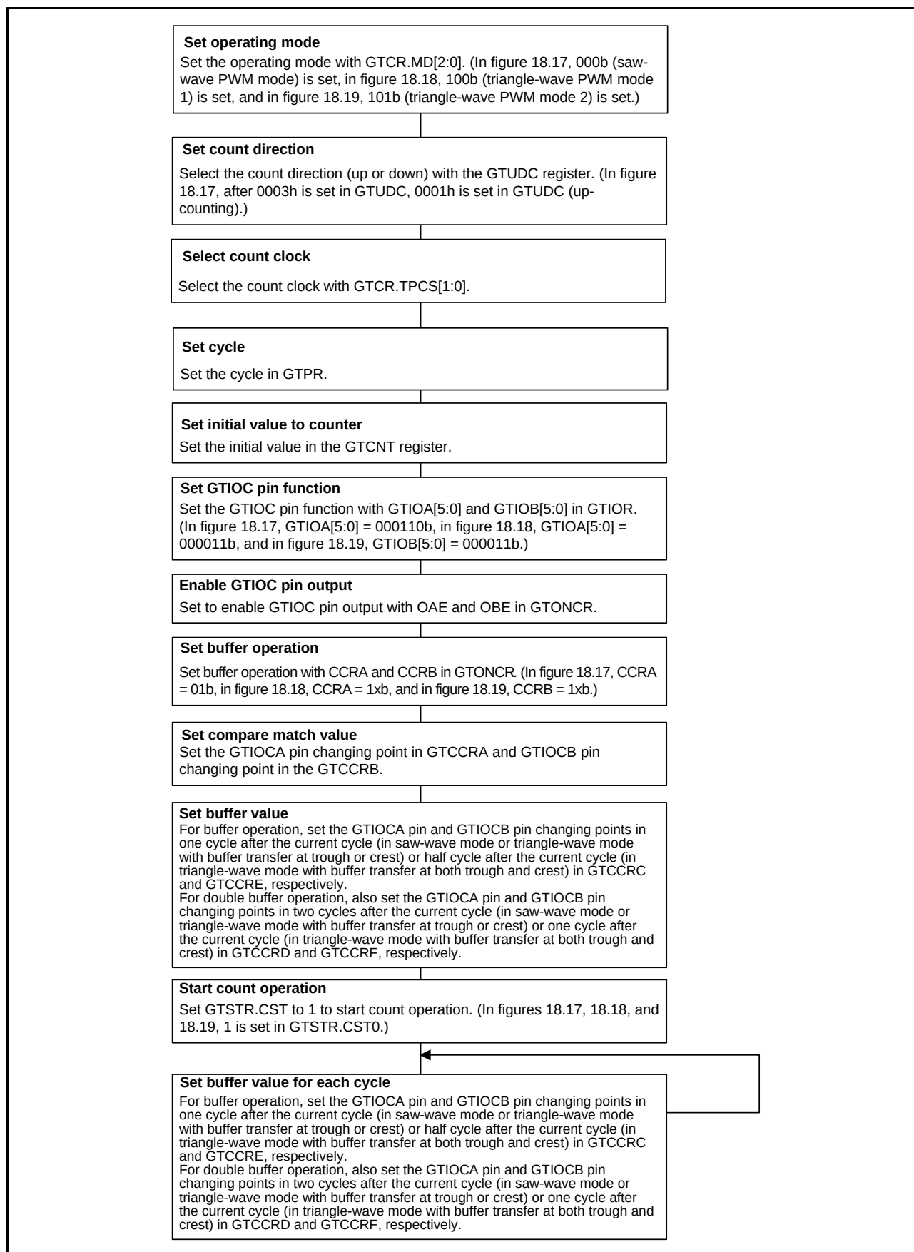
Figure 18.20 Example for Setting GTCRA and GTCCRB Buffer Operation (for Output Compare)
