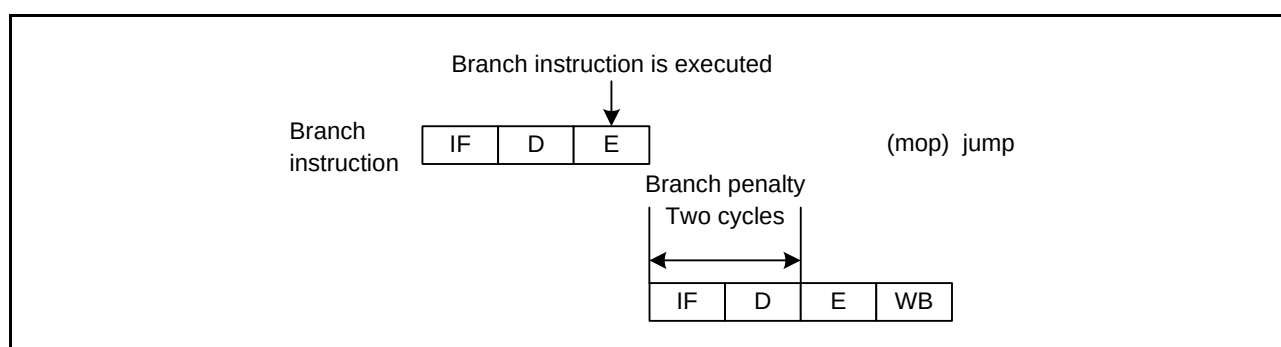
Figure 2.22 When a Branch Instruction is Executed (While the Condition is Satisfied for Unconditional/ Conditional Branch Instruction)
