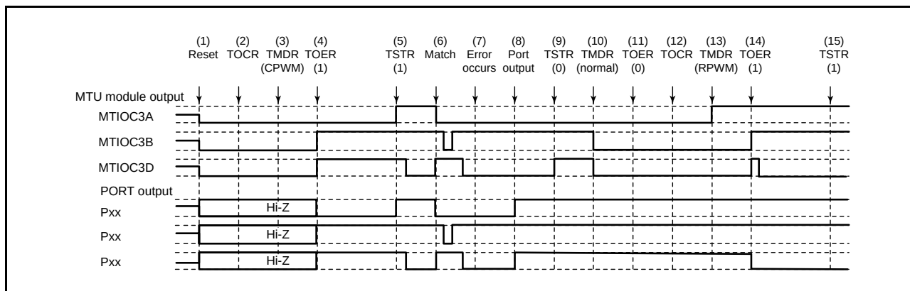
Figure 16.165 Error Occurrence in Complementary PWM Mode, Recovery in Reset-Synchronized PWM Mode
