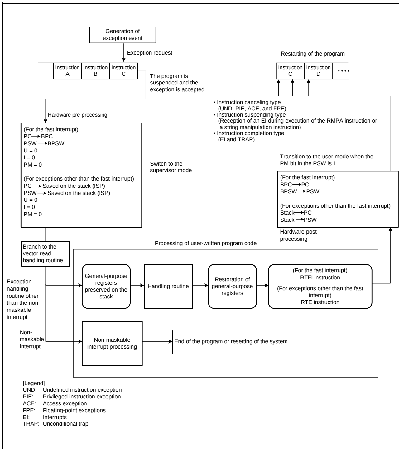
Figure 10.2 Outline of the Exception Handling Procedure
