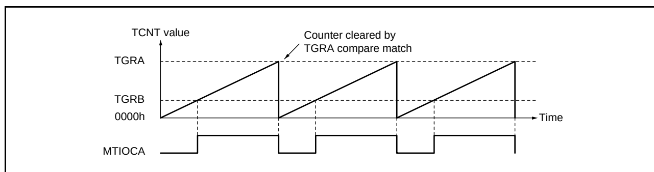
Figure 16.27 Example of PWM Mode 1 Operation
