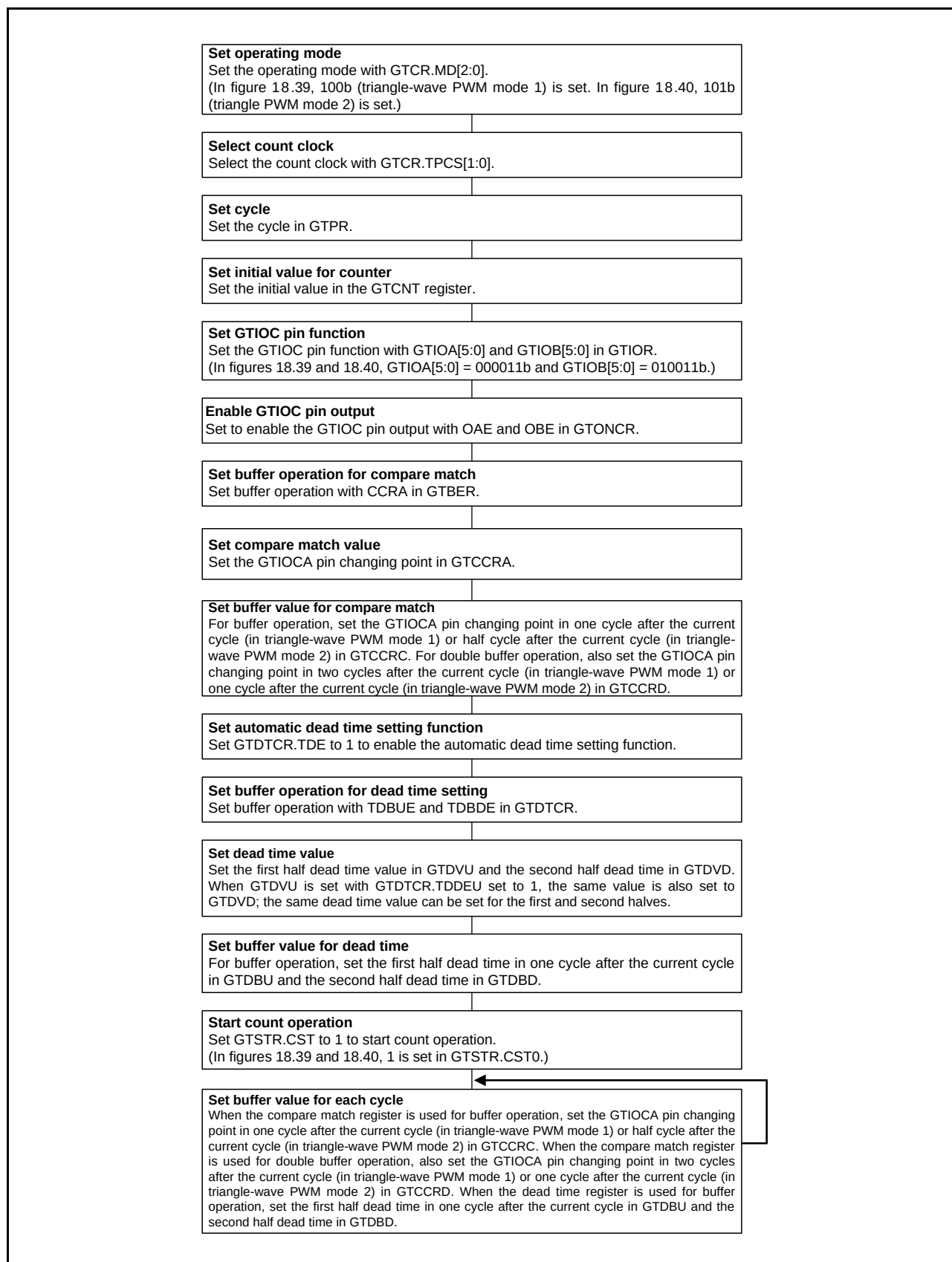
Figure 18.42 Example for Setting Automatic Dead Time Setting Function (Triangle-Wave PWM Mode 1 or 2)
