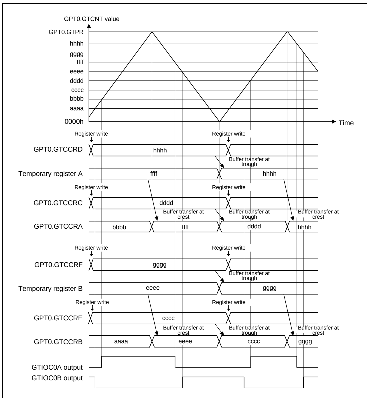
Figure 18.36 Example of Triangle-Wave PWM Mode 3 Operation (Low Output from GTIOC0A and High Output from GTIOC0B at Count Start, Toggle Output at GTCCRA/GTCCRB Compare Match, Output Retained at Cycle End)
