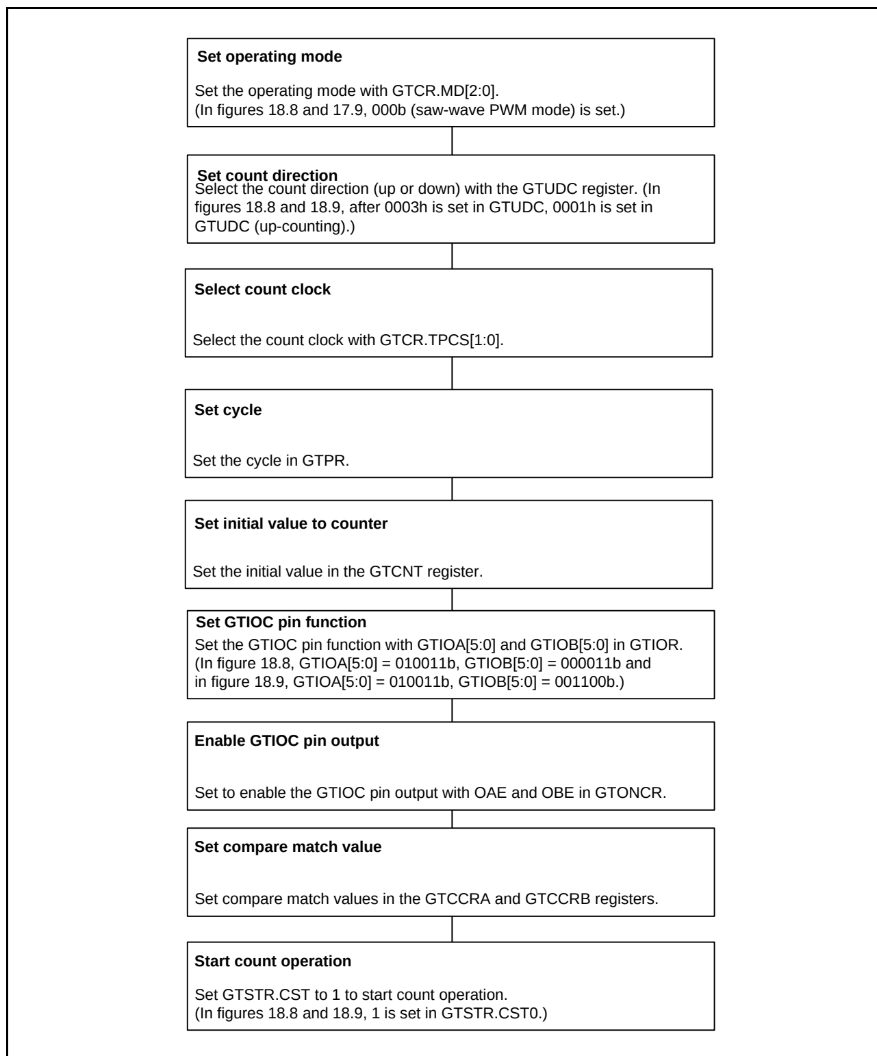
Figure 18.10 Example for Setting Toggled Output Operation
