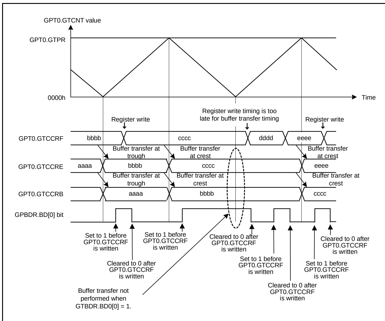
Figure 18.81 Example of Operation for Disabling Buffer Operation (Triangle Waves, Double Buffer Operation, Buffer Transfer at Both Troughs and Crests)
