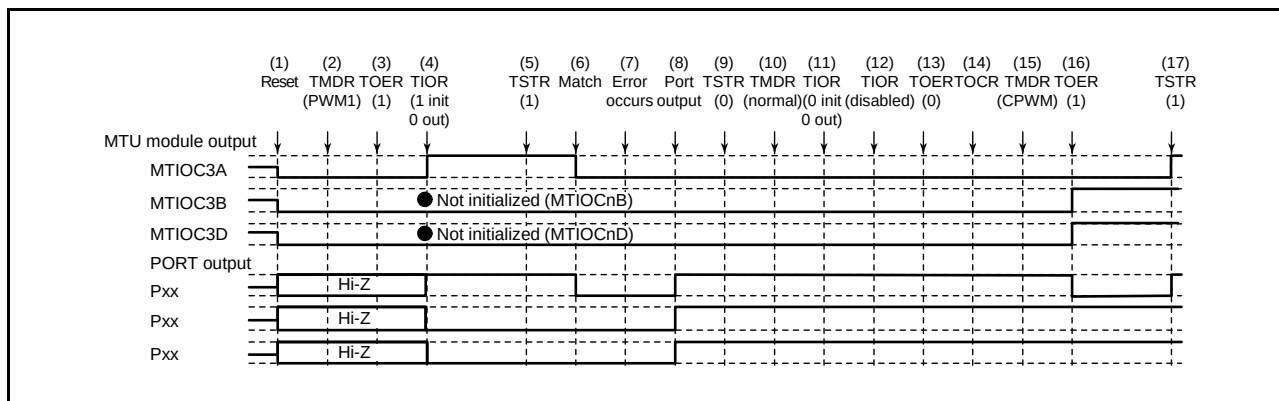
Figure 16.151 Error Occurrence in PWM Mode 1, Recovery in Complementary PWM Mode
