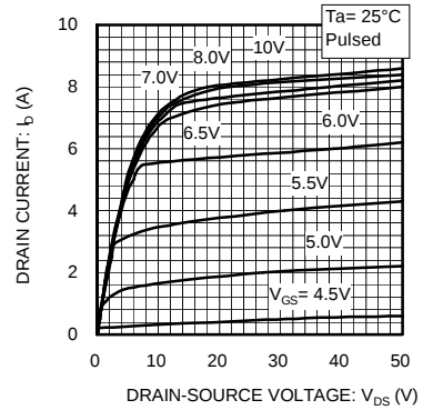
Fig.2 Typical Output Characteristics (I)
