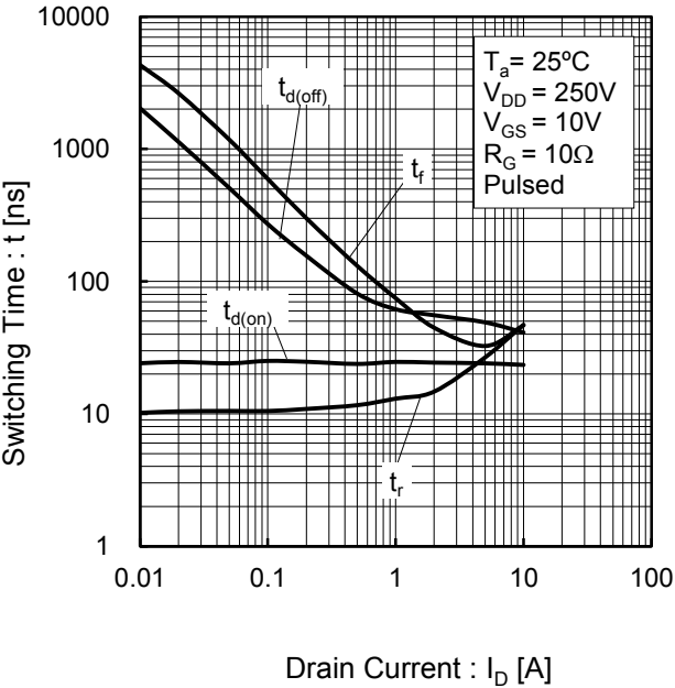
Fig.20 Switching Characteristics
