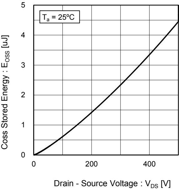
Fig.19 Coss Stored Energy
