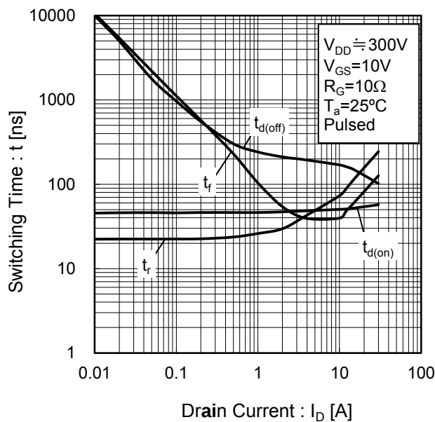
Fig.20 Switching Characteristics
