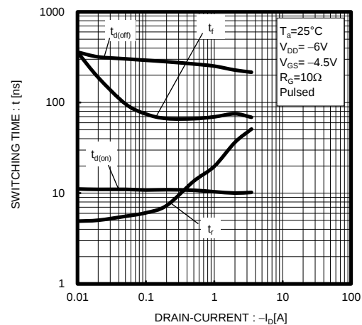
Fig.12 Switching Characteristics
