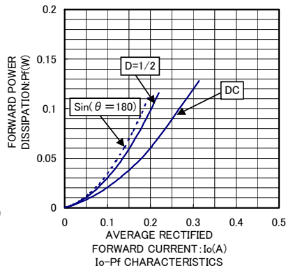
Io-Pf CHARACTERISTICS
