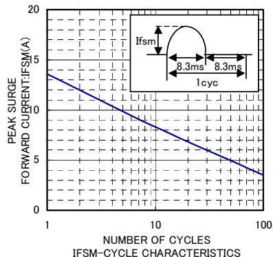
IFSM-CYCLE CHARACTERISTICS
