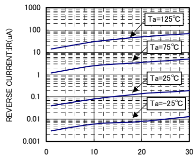
VR-IR CHARACTERISTICS
