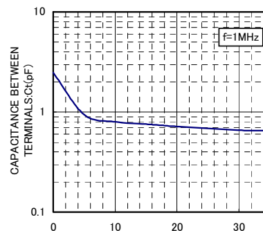
VR-Ct CHARACTERISTICS
