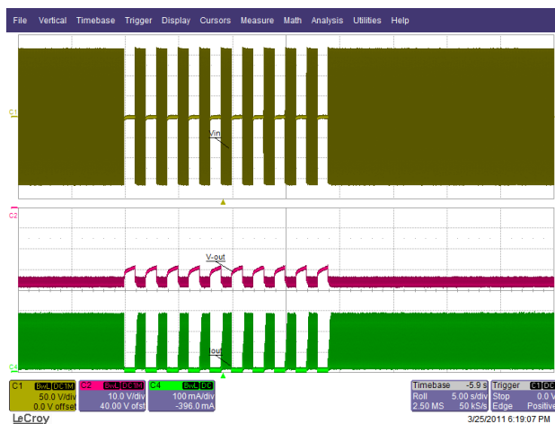
Figure 42 – 115 VAC / 50 Hz, 1 s On - 1 s Off. Load: 35 V LED String. Ch1: V_{IN} , 50 V / div. Ch2: V_{OUT} , 10 V / div. Ch4: I_{OUT} , 100 mA / div., 5 s / div.
