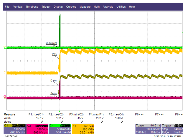
Figure 39 – 135 VAC / 63 Hz, Output Shorted.
