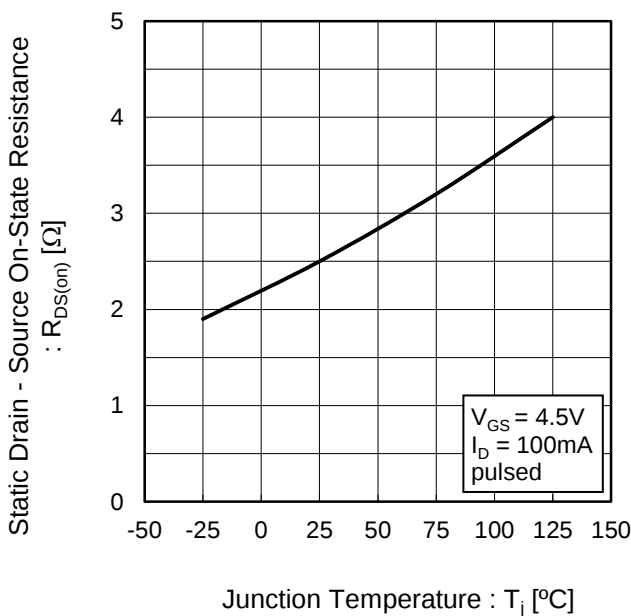
Fig.11 Static Drain - Source On - State Resistance vs. Junction Temperature
