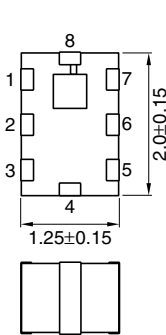
Top view
