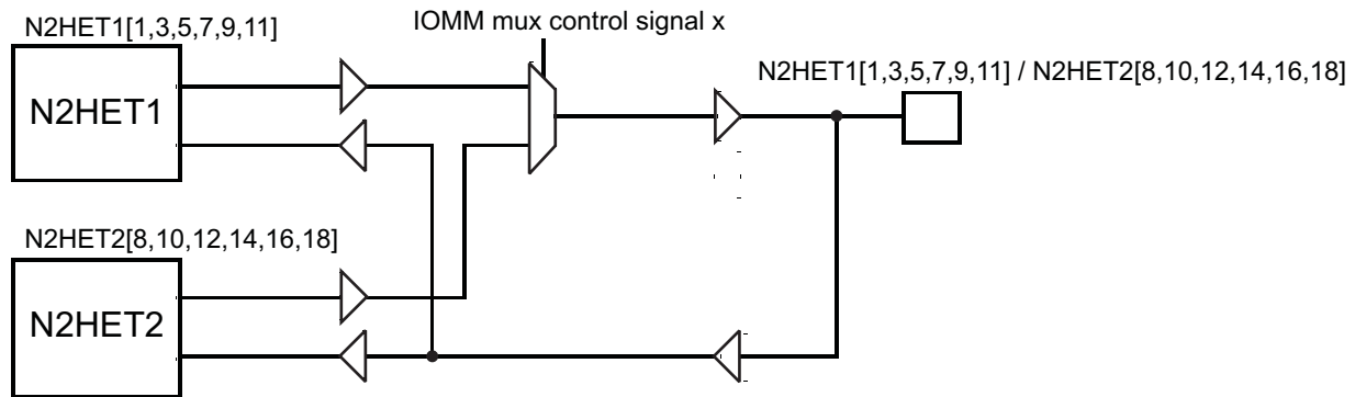
Figure 5-7. N2HET Monitoring
