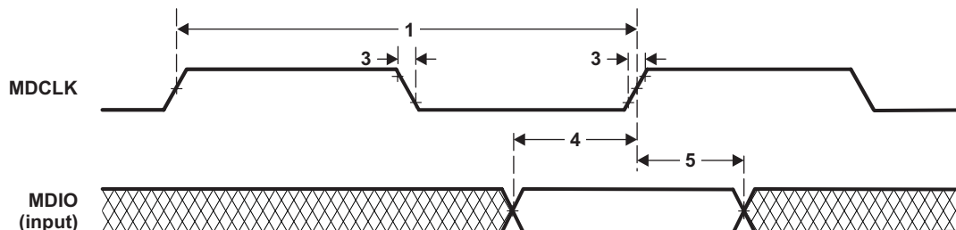
Figure 5-20. MDIO Input Timing
