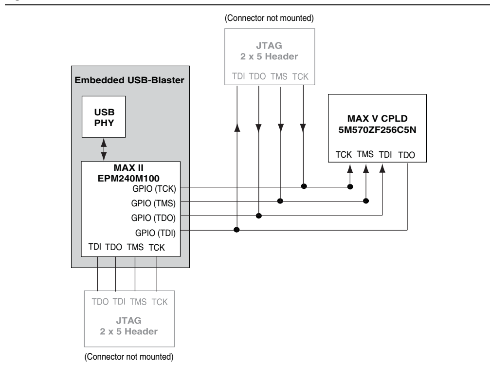
Figure 2–3. JTAG Chain
