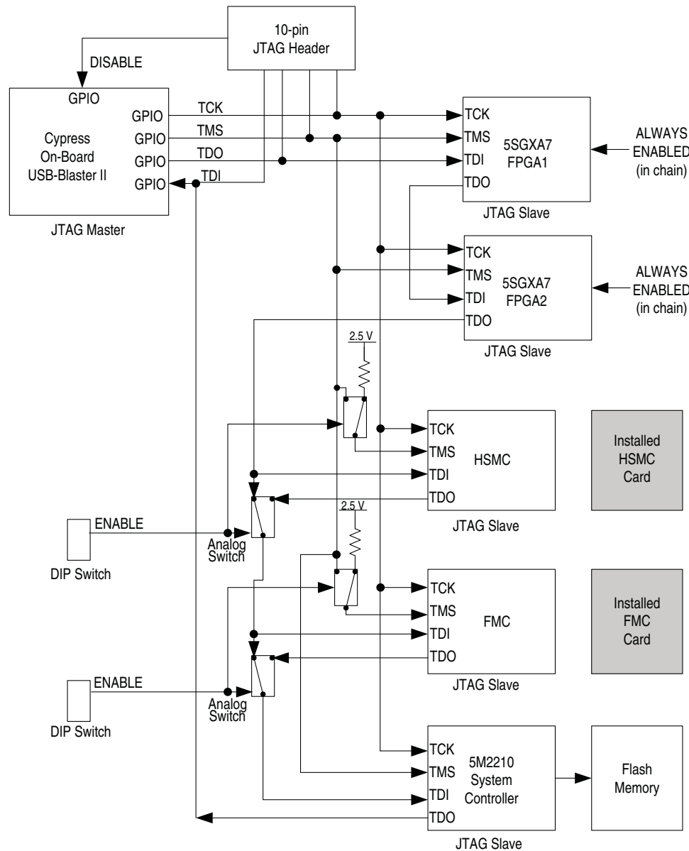
Figure 2-3. JTAG Chain
