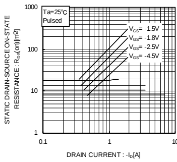
Fig.4 Static Drain-Source On-State Resistance vs. Drain Current(I)
