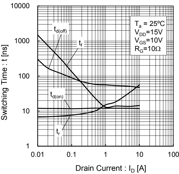
Fig.19 Switching Characteristics
