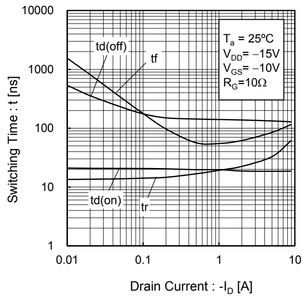
Fig.21 Switching Characteristics
